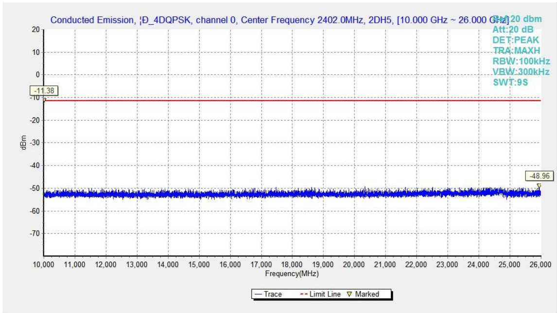
Fig.47. Conducted spurious emission: \pi/4 DQPSK, Channel 0, 10GHz - 26GHz
