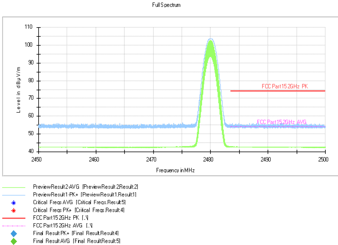
Fig.23. Frequency Band Edges: GFSK, Channel 78, Hopping Off, ch11, 2.45 GHz - 2.50GHz
