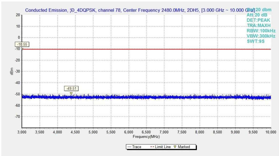
Fig.56. Conducted spurious emission: \pi/4 DQPSK, Channel 78, 3GHz - 10GHz
