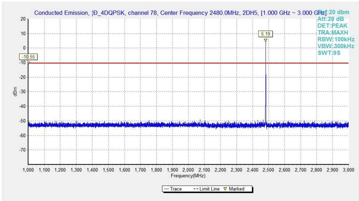
Fig.55. Conducted spurious emission: \pi/4 DQPSK, Channel 78, 1GHz - 3GHz
