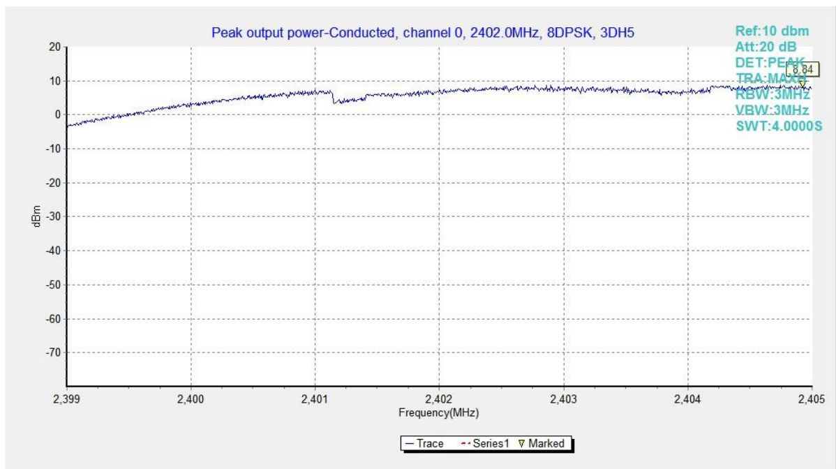
Fig.7. Peak Output Power -Conducted: 8DPSK, Channel 0,
