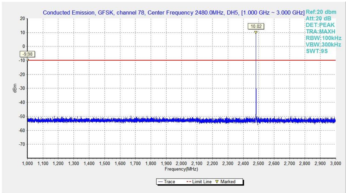
Fig.40. Conducted spurious emission: GFSK, Channel 78, 1GHz - 3GHz
