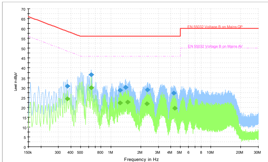
Fig.B.9.1 AC Powerline Conducted Emission- Bluetooth BLE 5.0
