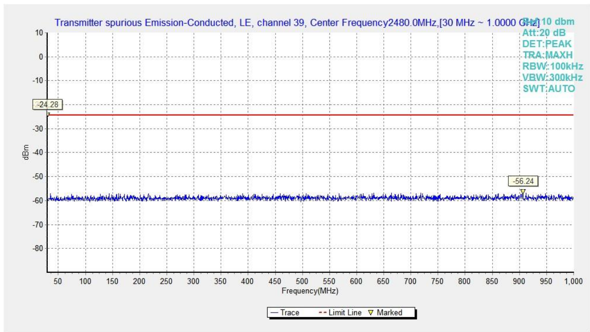
Fig.24. Transmitter Spurious Emission - Conducted: GFSK, 2480 MHz, 30MHz - 1GHz
