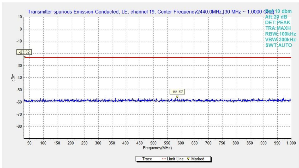
Fig.19. Transmitter Spurious Emission - Conducted: GFSK, 2440 MHz, 30MHz - 1GHz
