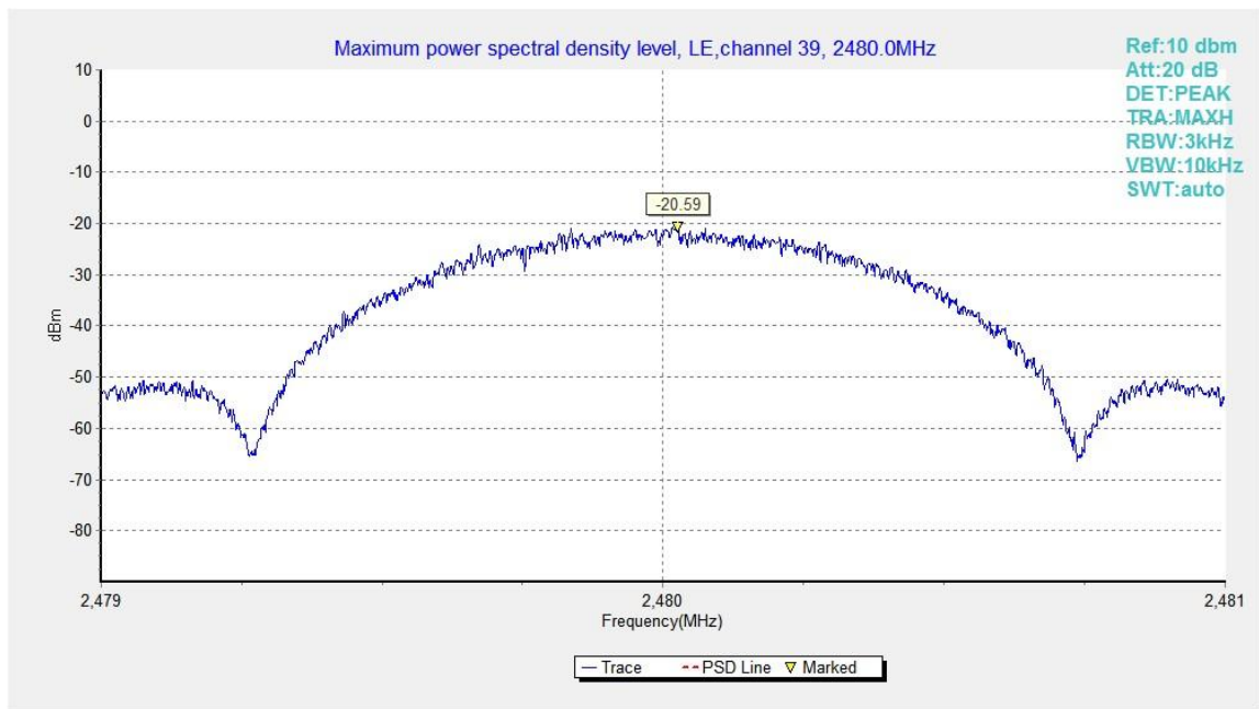
Fig.33. Maximum Power Spectral Density Level Function: GFSK, 2480 MHz
