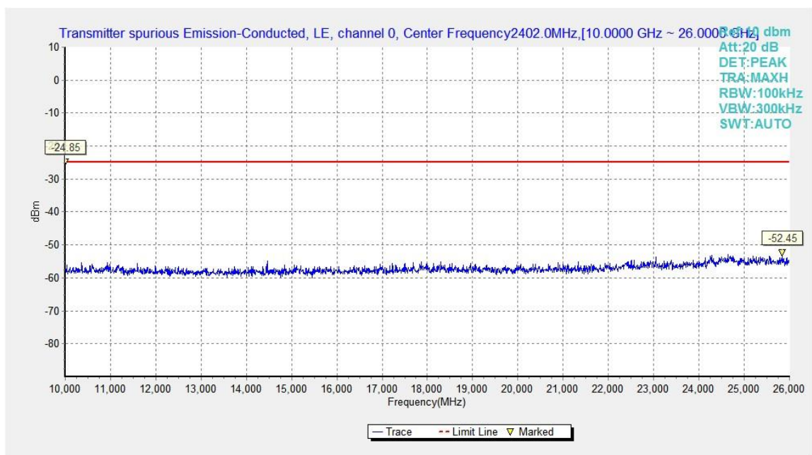
Fig.17. Transmitter Spurious Emission - Conducted: GFSK, 2402 MHz, 10GHz - 26GHz
