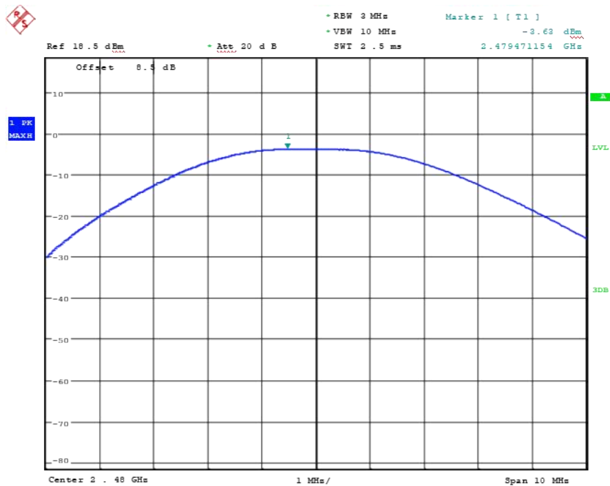
Fig.6. Peak Conducted Output Power: BLE, 2Mbps, Channel 39,
