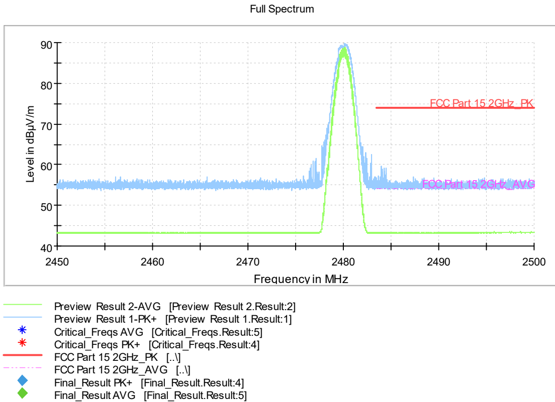
Fig.10. Frequency Band Edges: BLE 4.0 GFSK, 2480 MHz, Hopping Off , 2.45 GHz - 2.50GHz
