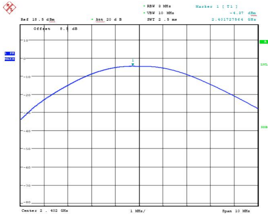
Fig.1. Peak Conducted Output Power: BLE, 1Mbps, Channel 0,
