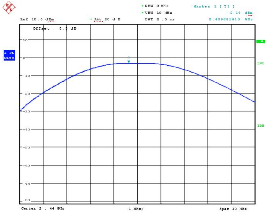
Fig.5. Peak Conducted Output Power: BLE, 2Mbps, Channel 19,
