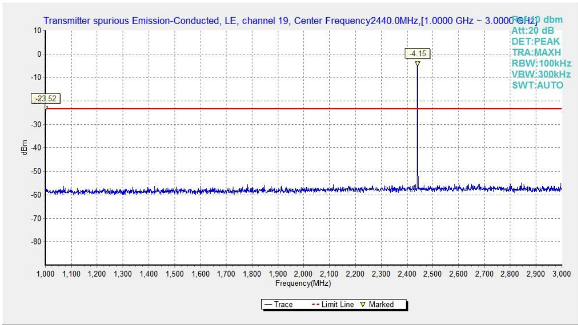
Fig.20. Transmitter Spurious Emission - Conducted: GFSK, 2440 MHz, 1GHz – 3GHz
