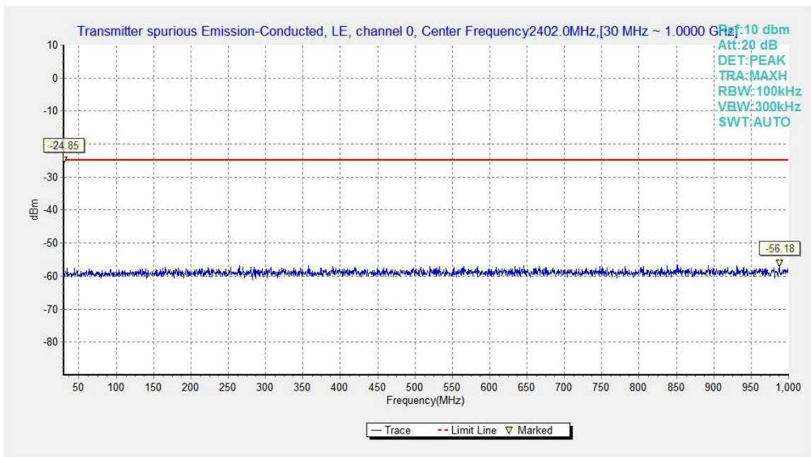
Fig.14. Transmitter Spurious Emission - Conducted: GFSK, 2402 MHz, 30MHz - 1GHz
