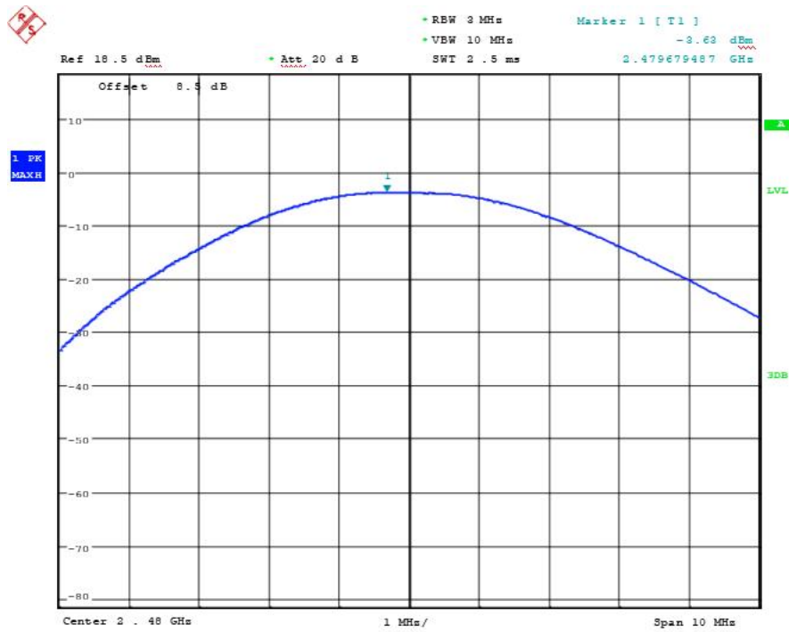
Fig.3. Peak Conducted Output Power: BLE, 1Mbps, Channel 39,
