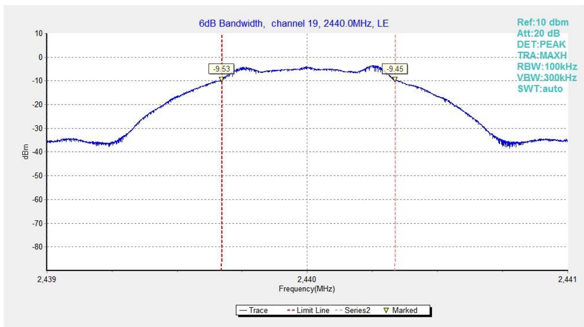
Fig.29. 6dB Bandwidth: GFSK, 2440 MHz
