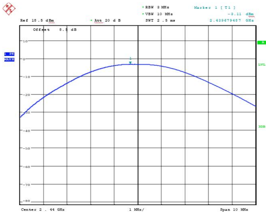
Fig.2. Peak Conducted Output Power: BLE, 1Mbps, Channel 19,
