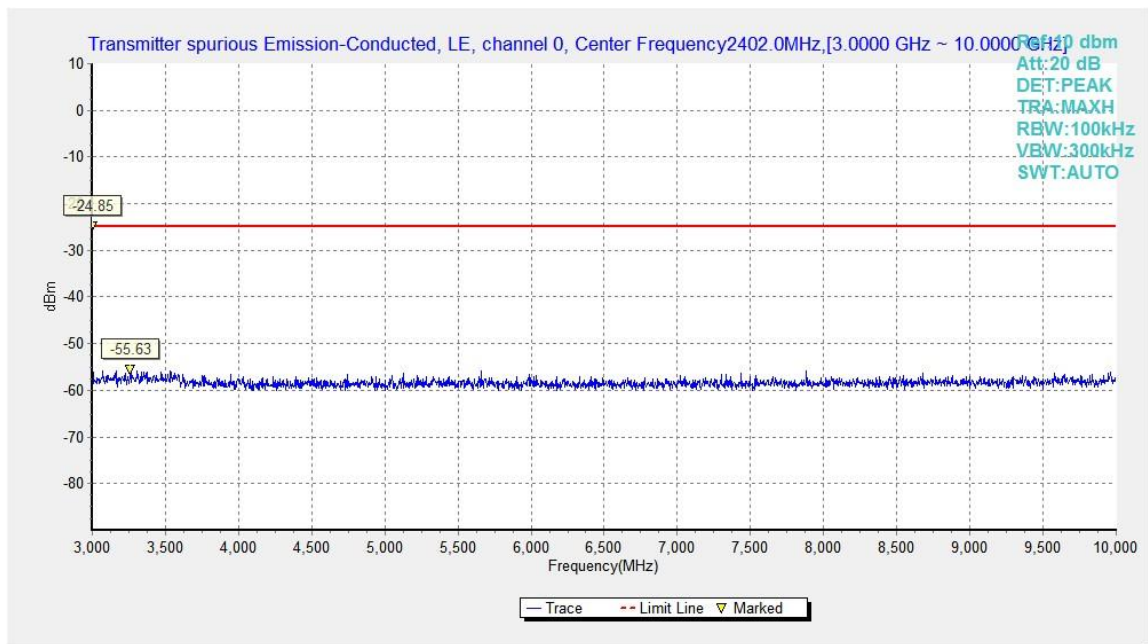
Fig.16. Transmitter Spurious Emission - Conducted: GFSK, 2402 MHz, 3GHz - 10GHz
