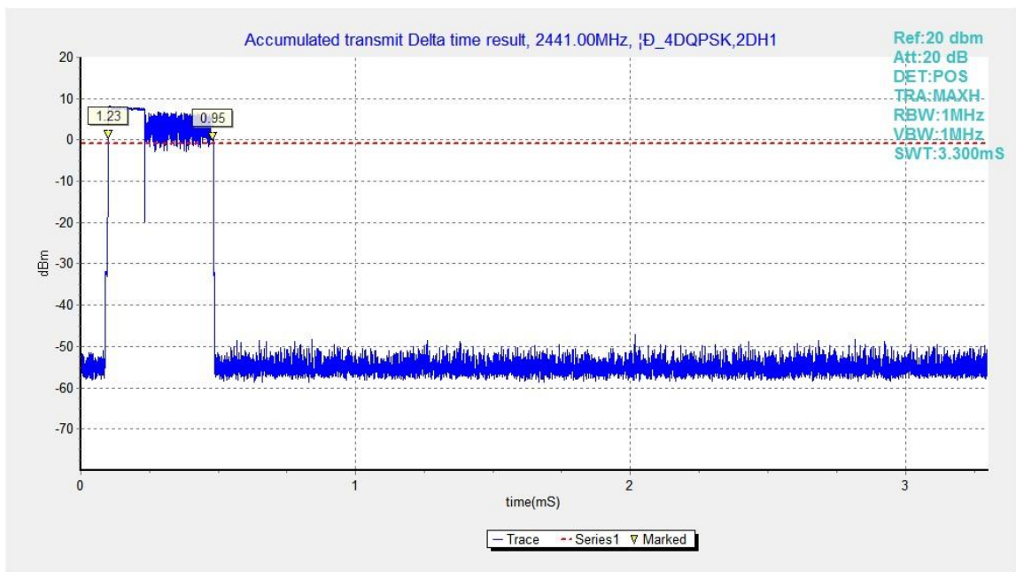
Fig.79. Time of occupancy (Dwell Time): Channel 39, Packet 2-DH1
