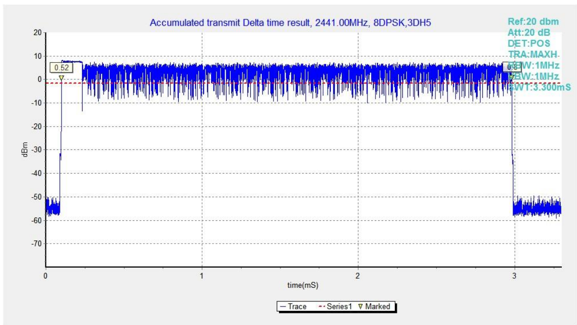
Fig.89. Time of occupancy (Dwell Time): Channel 39, Packet 3-DH5
