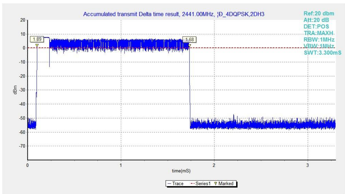
Fig.81. Time of occupancy (Dwell Time): Channel 39, Packet 2-DH3
