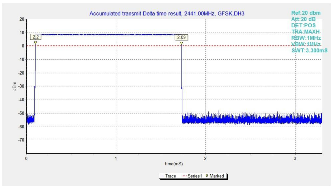
Fig.75. Time of occupancy (Dwell Time): Channel 39, Packet DH3
