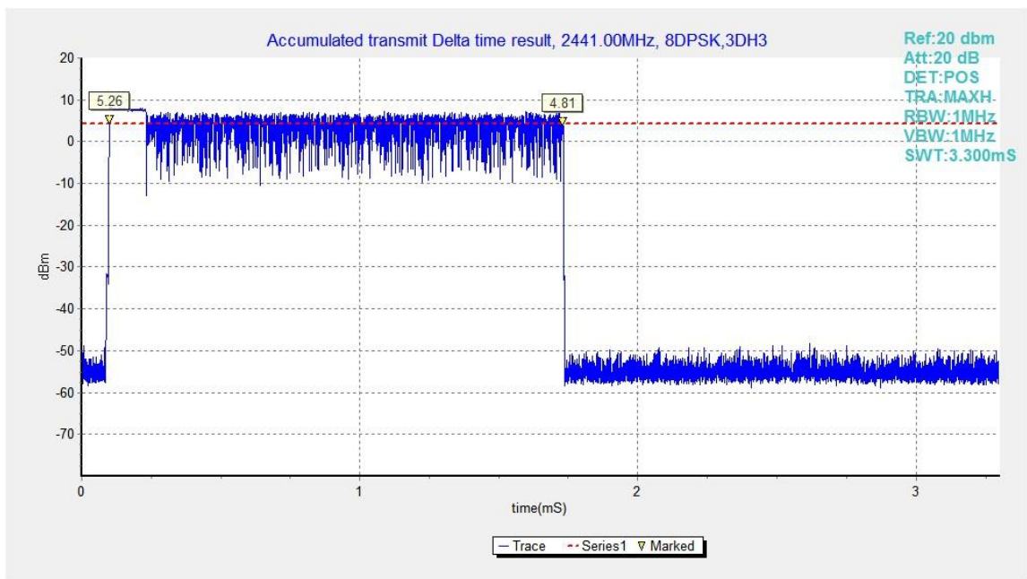
Fig.87. Time of occupancy (Dwell Time): Channel 39, Packet 3-DH3
