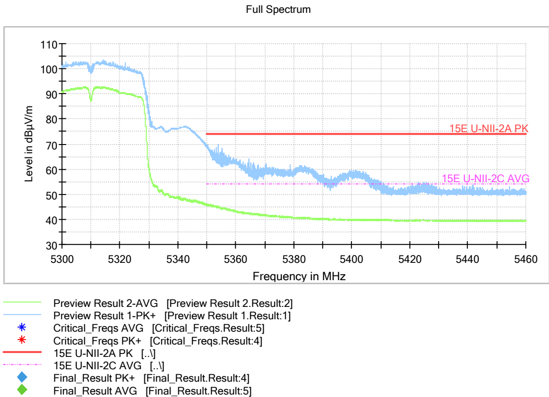
Fig.47 Band Edges (802.11n-HT40, 5310MHz)
