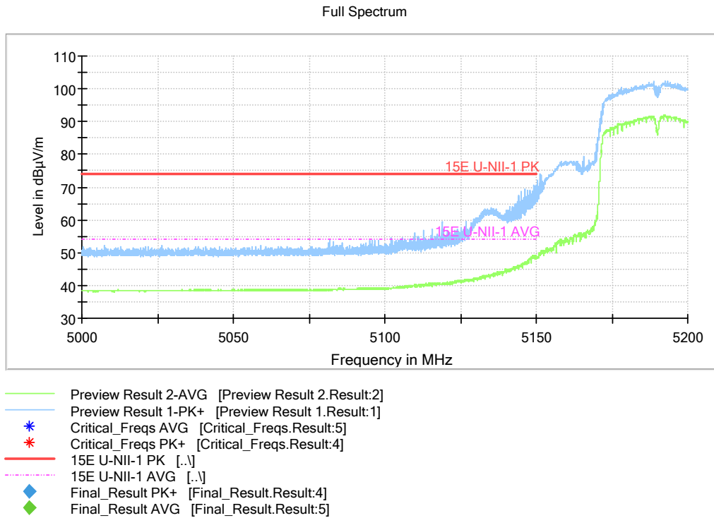
Fig.46 Band Edges (802.11n-HT40, 5190MHz)
