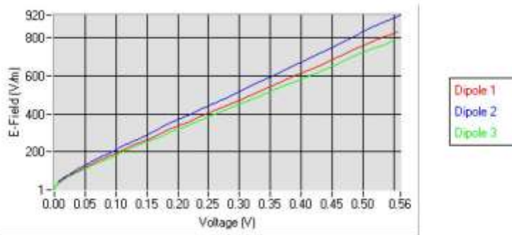
Calibration curves
