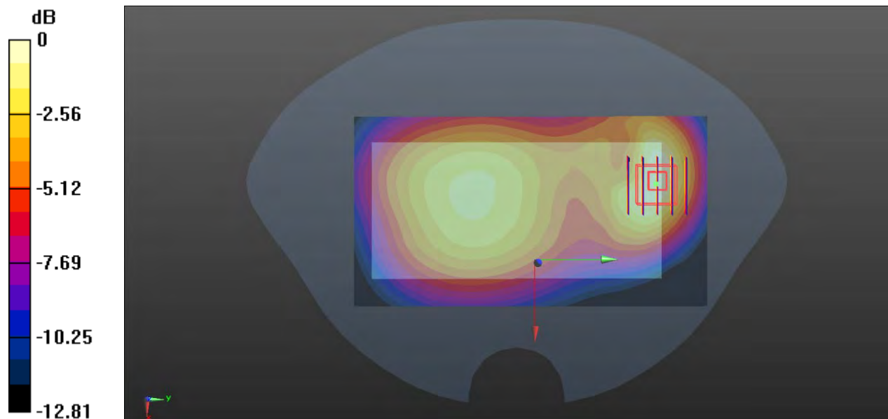
0 dB = 0.236 W/kg
