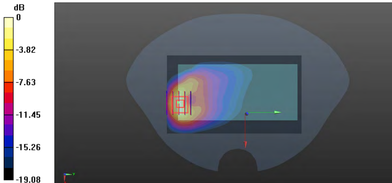
0 dB = 3.28 W/kg
