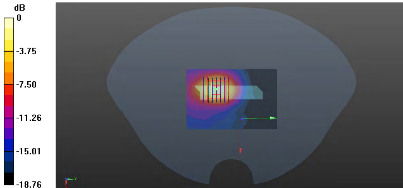
0 dB = 0.669 W/kg
