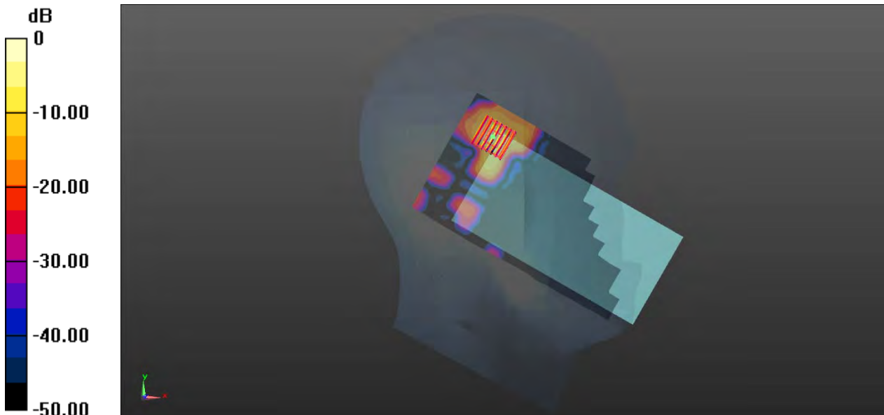
0 dB = 1.86 W/kg
