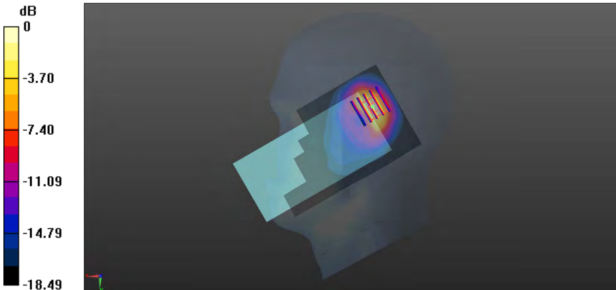
0 dB = 0.649 W/kg
