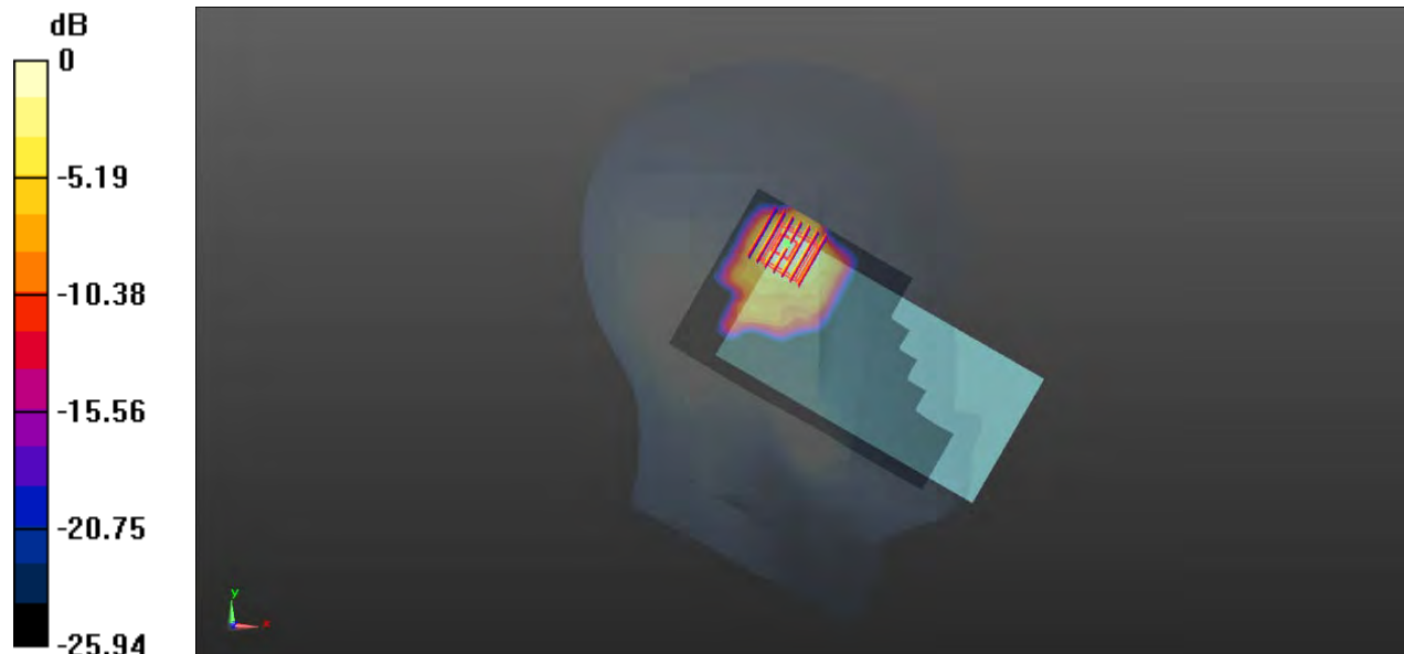
0 dB = 0.0760 W/kg
