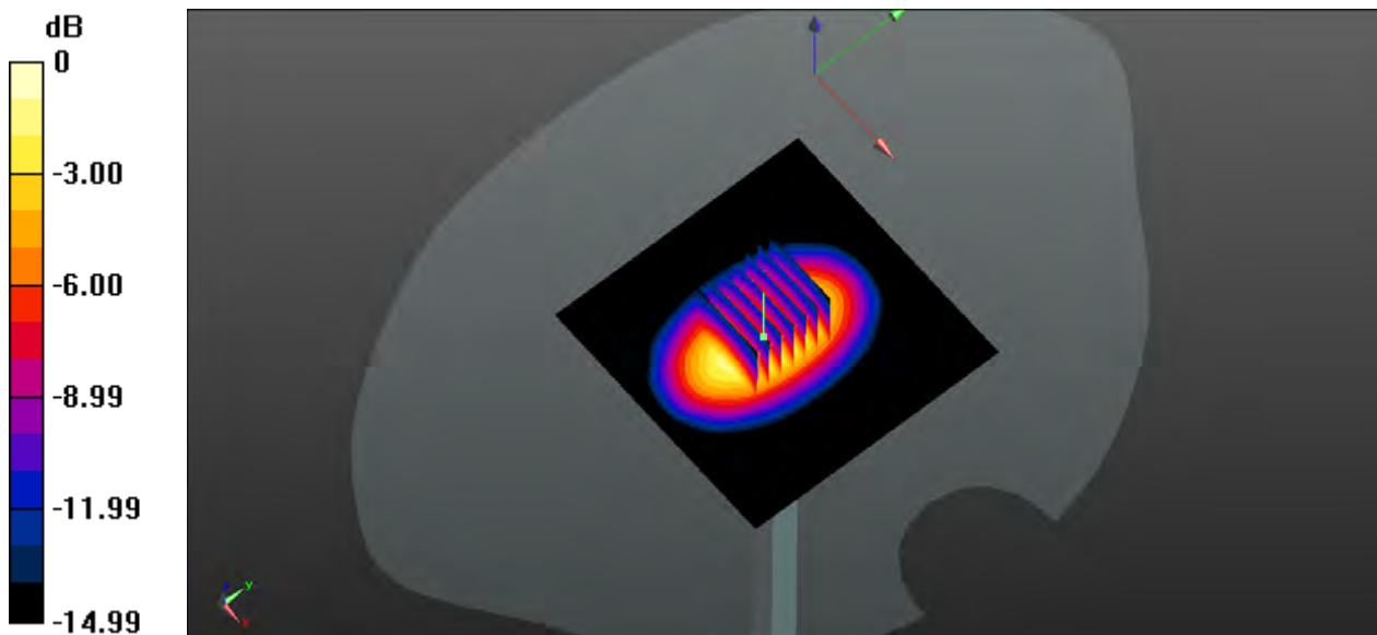
0 dB = 4.16 W/kg
