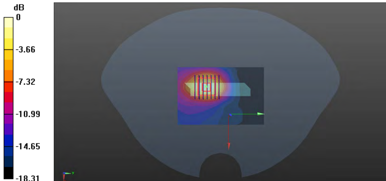
0 dB = 0.595 W/kg
