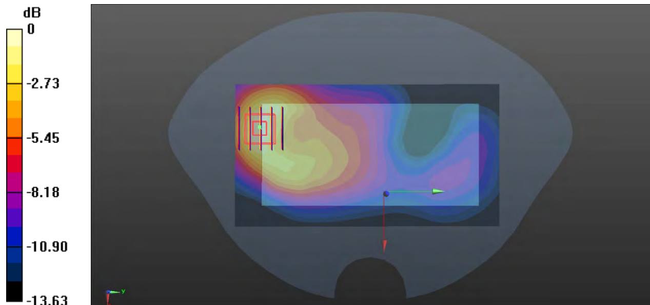
0 dB = 0.232 W/kg
