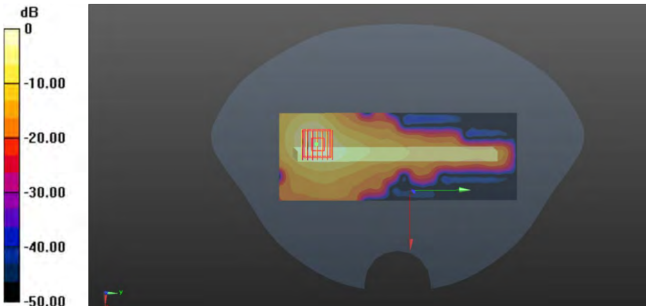
0 dB = 0.863 W/kg
