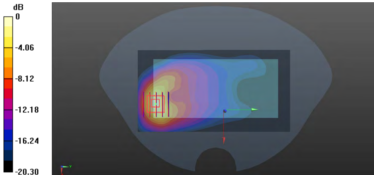
0 dB = 2.49 W/kg
