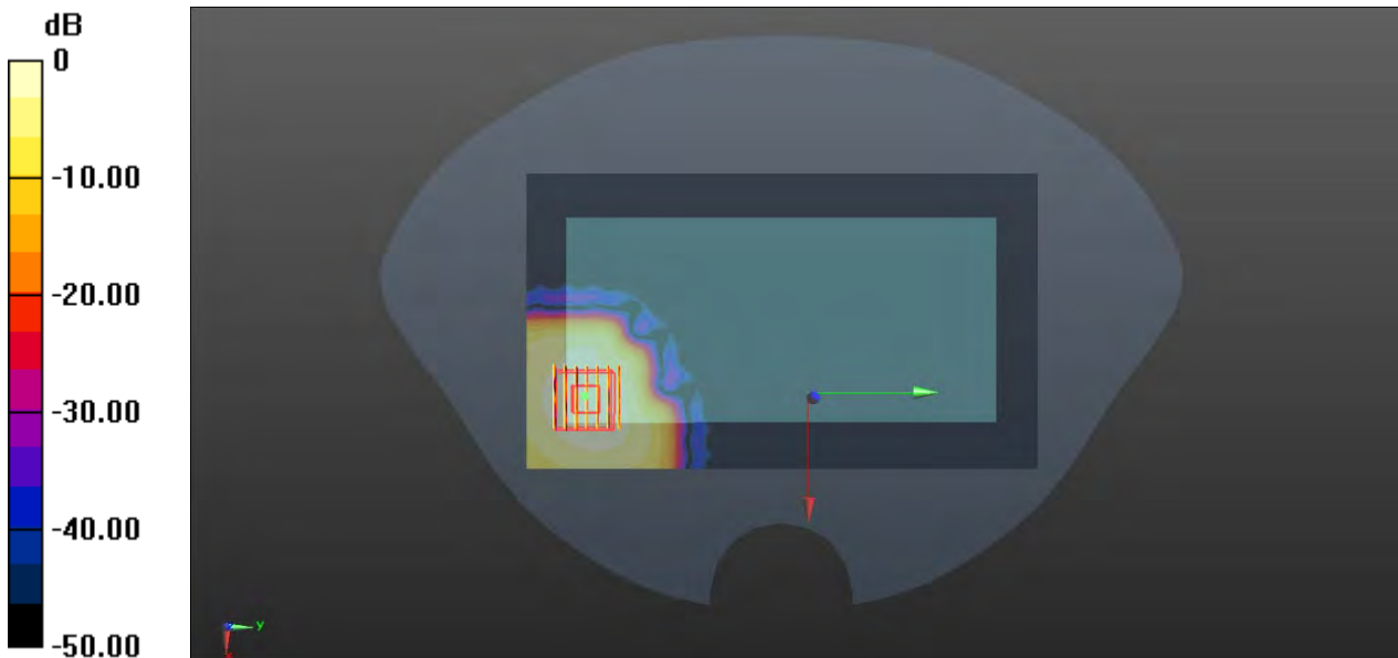
0 dB = 0.163 W/kg
