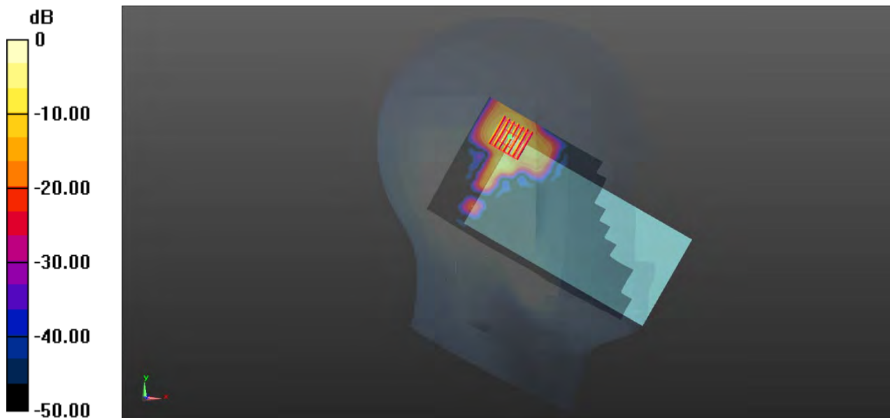
0 dB = 1.08 W/kg
