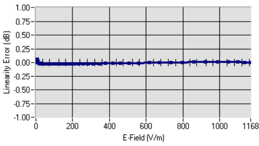
Linearity: +/- 1.49% (+/- 0.07 dB)
