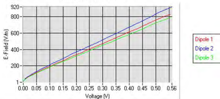
Calibration curves
