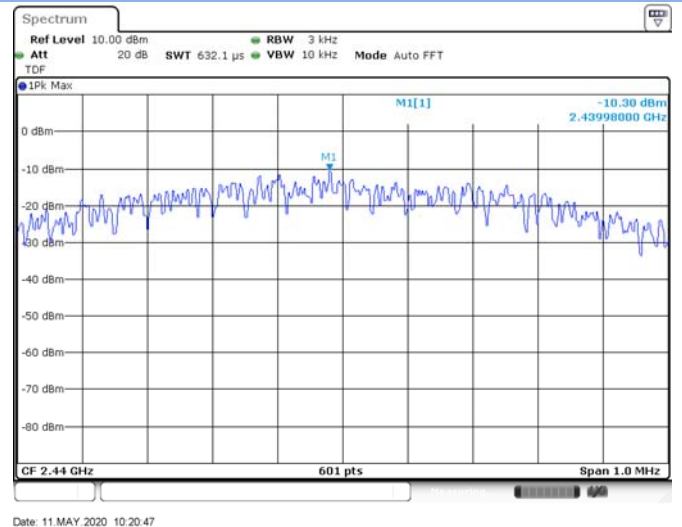
GFSK (BLE) MIDDLE CHANNEL
