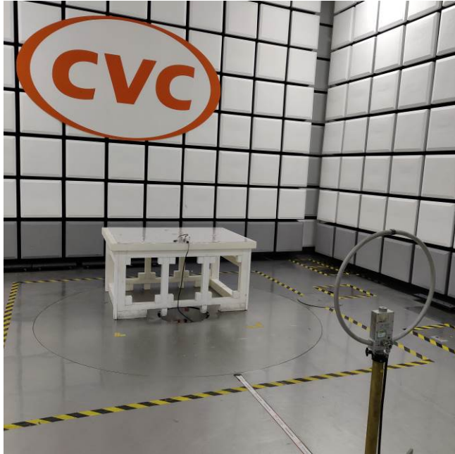
(1) Radiated spurious emission Test Setup-1(9KHz~30MHz)
