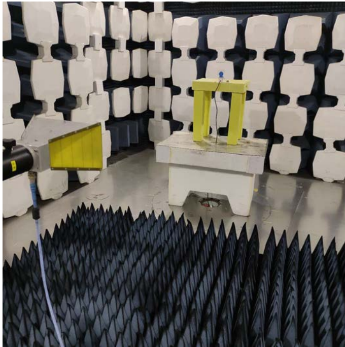
(3) Radiated spurious emission Test Setup-3(Above 1GHz)
