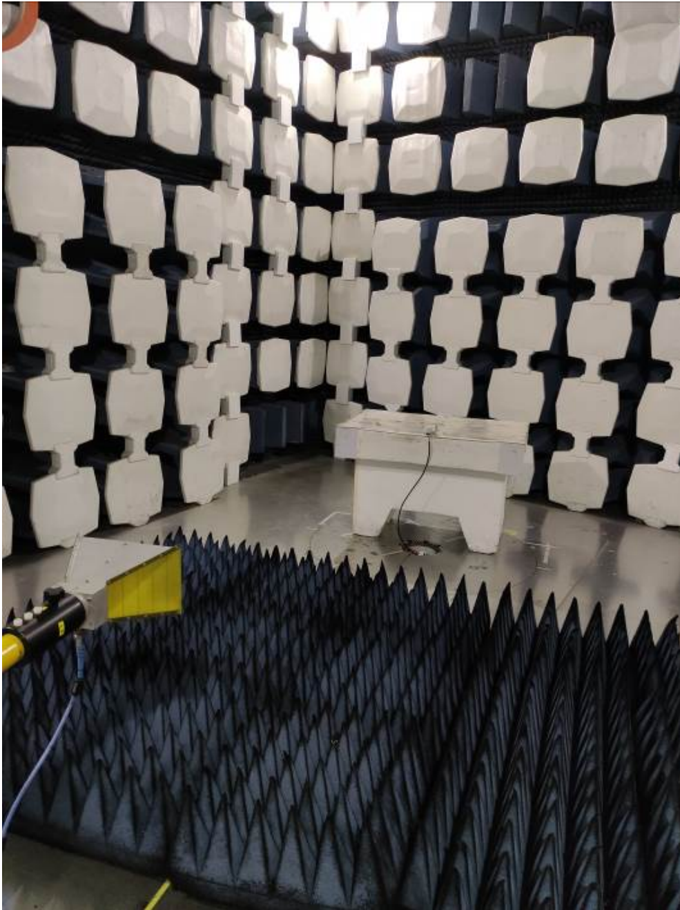
(2) Radiated spurious emission Test Setup(Above 1GHz)
