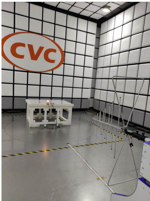
(2) Radiated spurious emission Test Setup-2(Below 1GHz)
