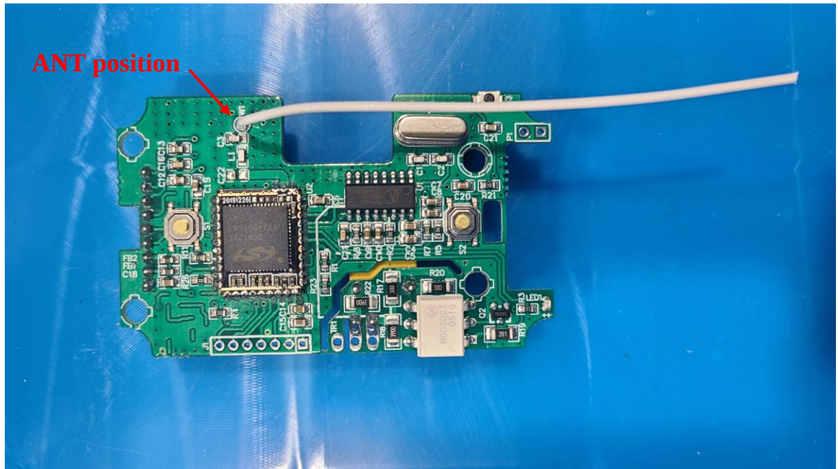
(7) EUT Photo
