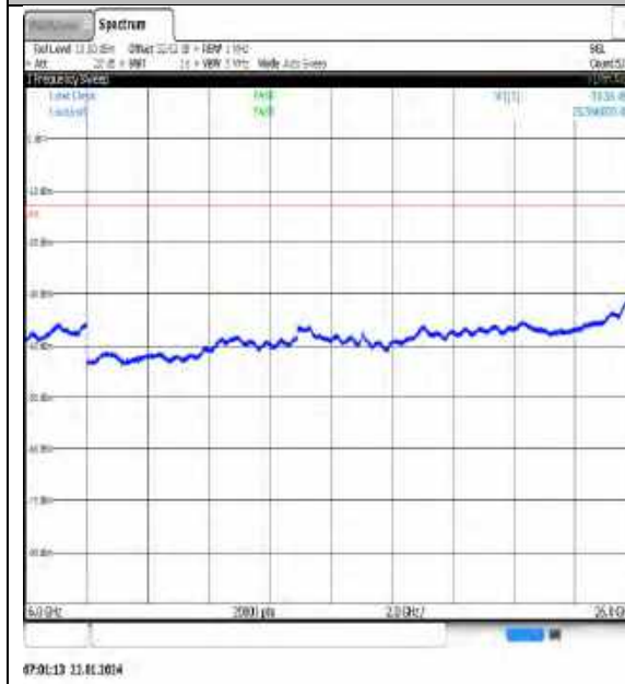
NTNV_N77-3700- 3980_PC3_30_25_M_TID5_NS_01_6000_26000_#1
