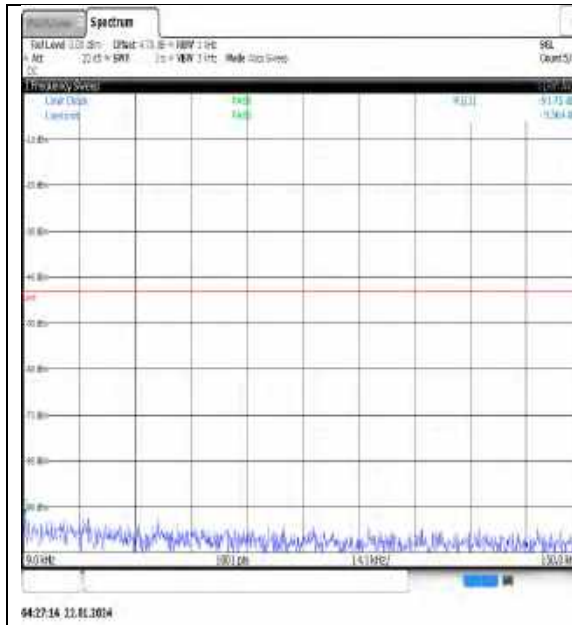
NTNV_N77-3700- 3980_PC3_30_20_M_TID5_NS_01_0.009_0.15_# 1
