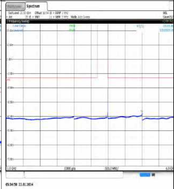
NTNV_N77-3700-3980_PC3_30_20_H_TID10_NS_01_1000_6000_#1
