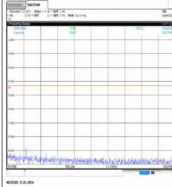
NTNV_N77-3700- 3980_PC3_30_25_M_TID3_NS_01_0.009_0.15_ #1
