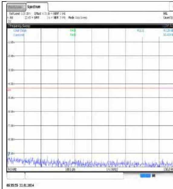
NTNV_N77-3700- 3980_PC3_30_25_L_TID13_NS_01_0.009_0.15_ #1
