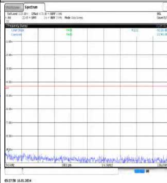
NTNV_N77-3450-3550_PC3_30_90_H_TID2_NS_01_0.009_0.15_#1
