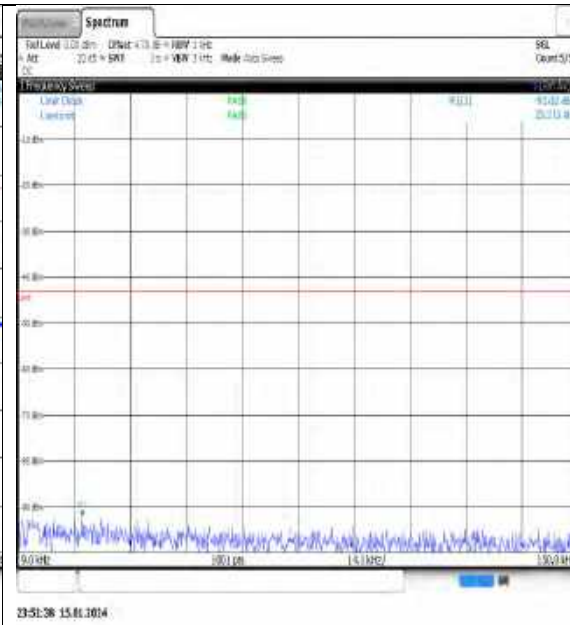
NTNV_N77-3450- 3550_PC3_30_70_H_TID6_NS_01_0.009_0.15_# 1
