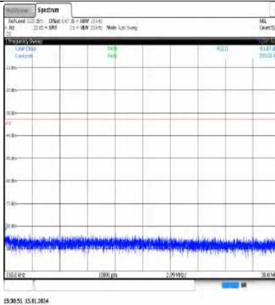
NTNV_N77-3450- 3550_PC3_30_50_M_TID10_NS_01_0.15_30_ #1
