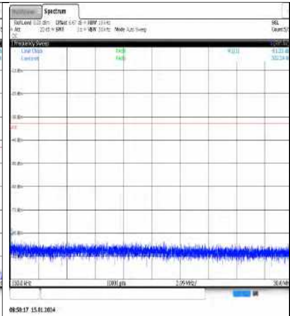
NTVN_N77-3450- 3550_PC3_30_30_L_TID9_NS_01_0.15_30_#1
