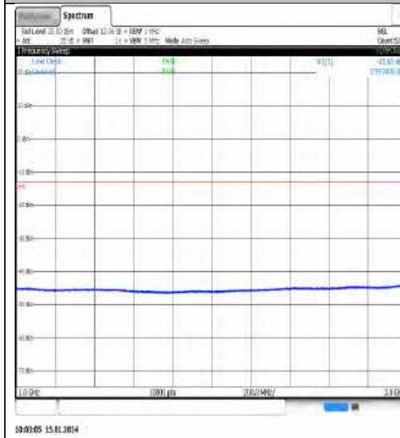
NTNV_N77-3450- 3550_PC3_30_30_M_TID11_NS_01_1000_3000_#1
