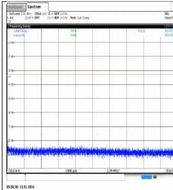
NTNV_N77-3450- 3550_PC3_30_25_L_TID7_NS_01_0.15_30_#1
