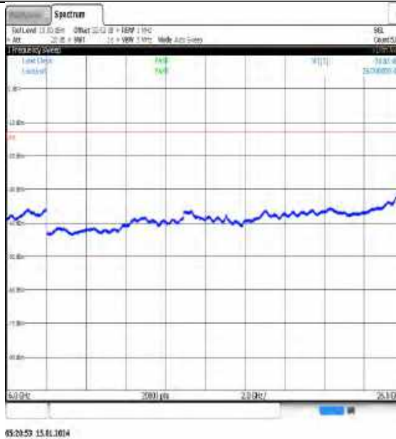
NTNV_N77-3450- 3550_PC3_30_20_H_TID11_NS_01_6000_26000_#1
