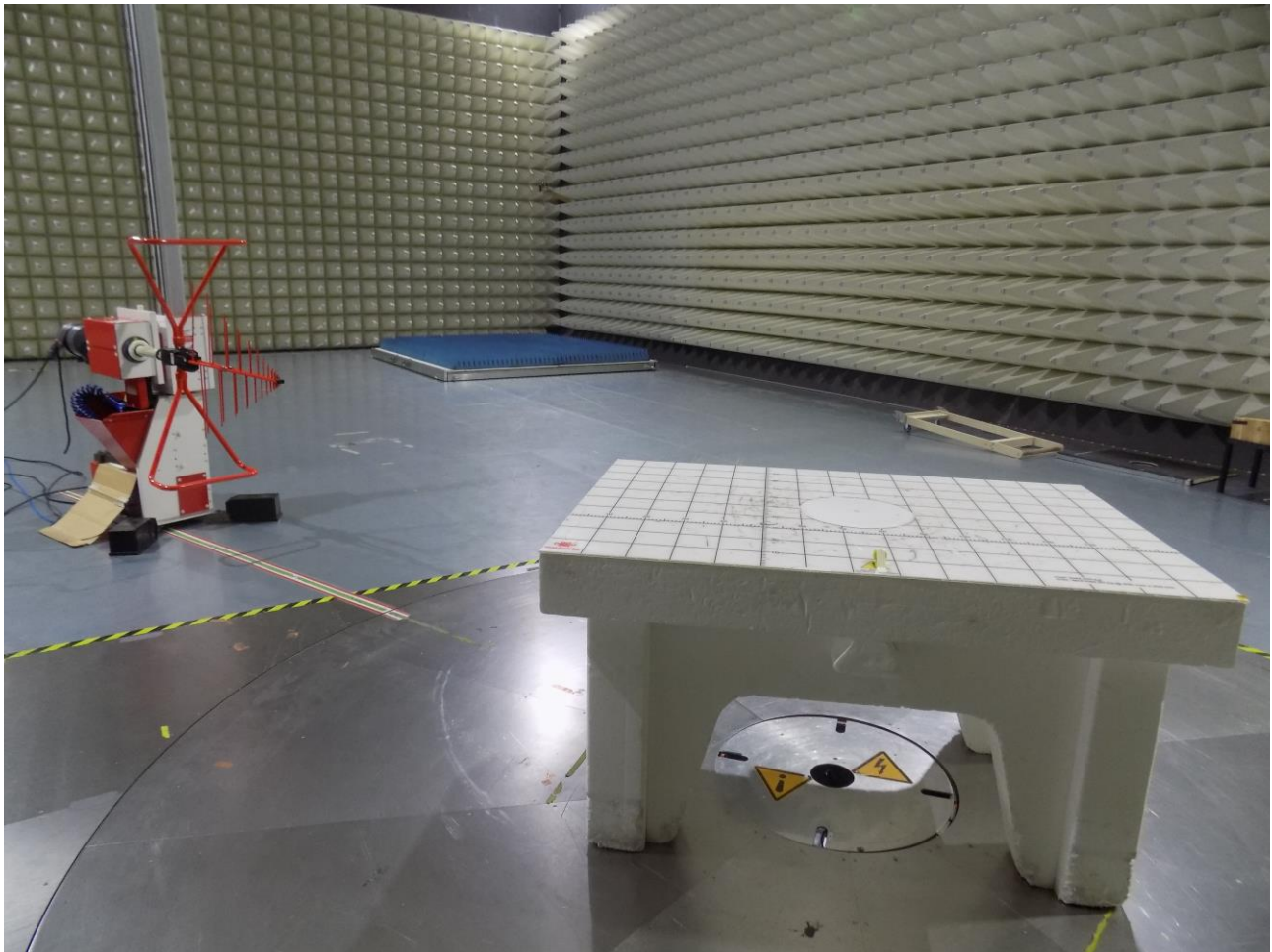
Figure 1: Test Setup for Radiated Emissions 30 MHz to 1000 MHz (BT LE, and Unintentional Modes)
