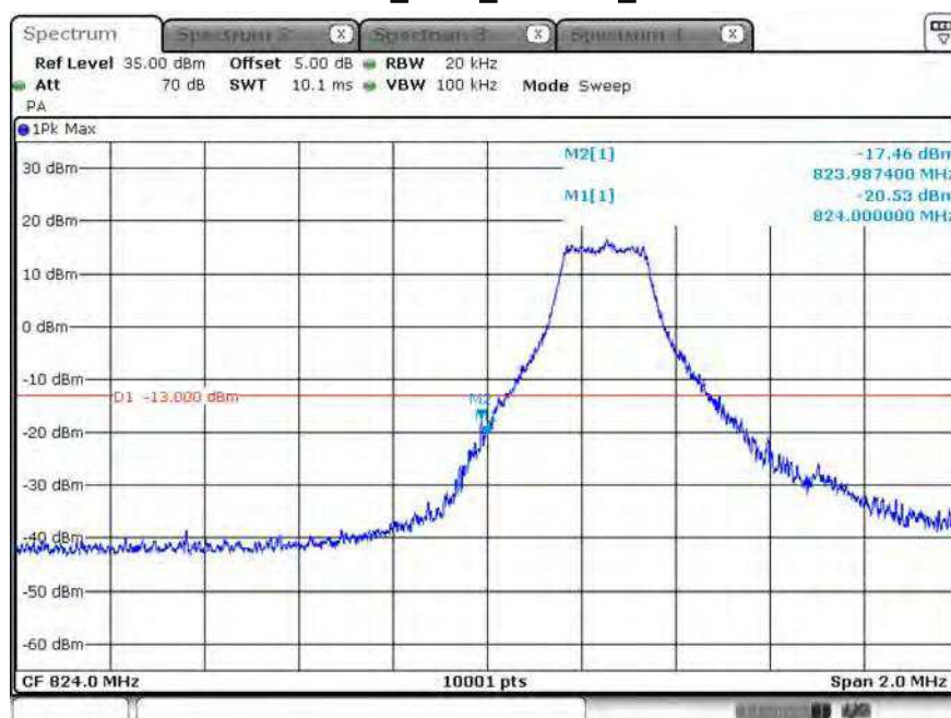
CH20407_1.4M_16-QAM_1RB0
