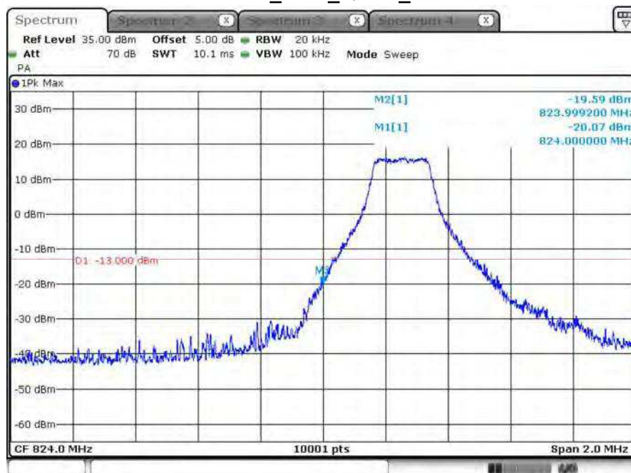
CH20407_1.4M_QPSK_1RB0
