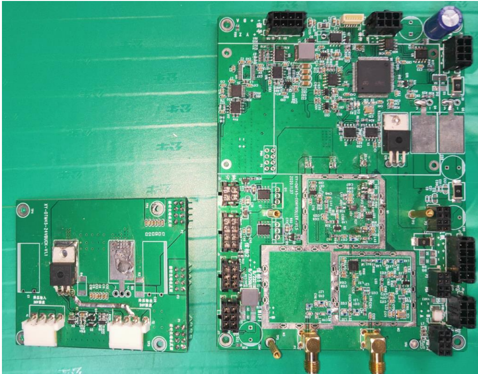
(26) EUT Photo (Out-cabin Unit)
