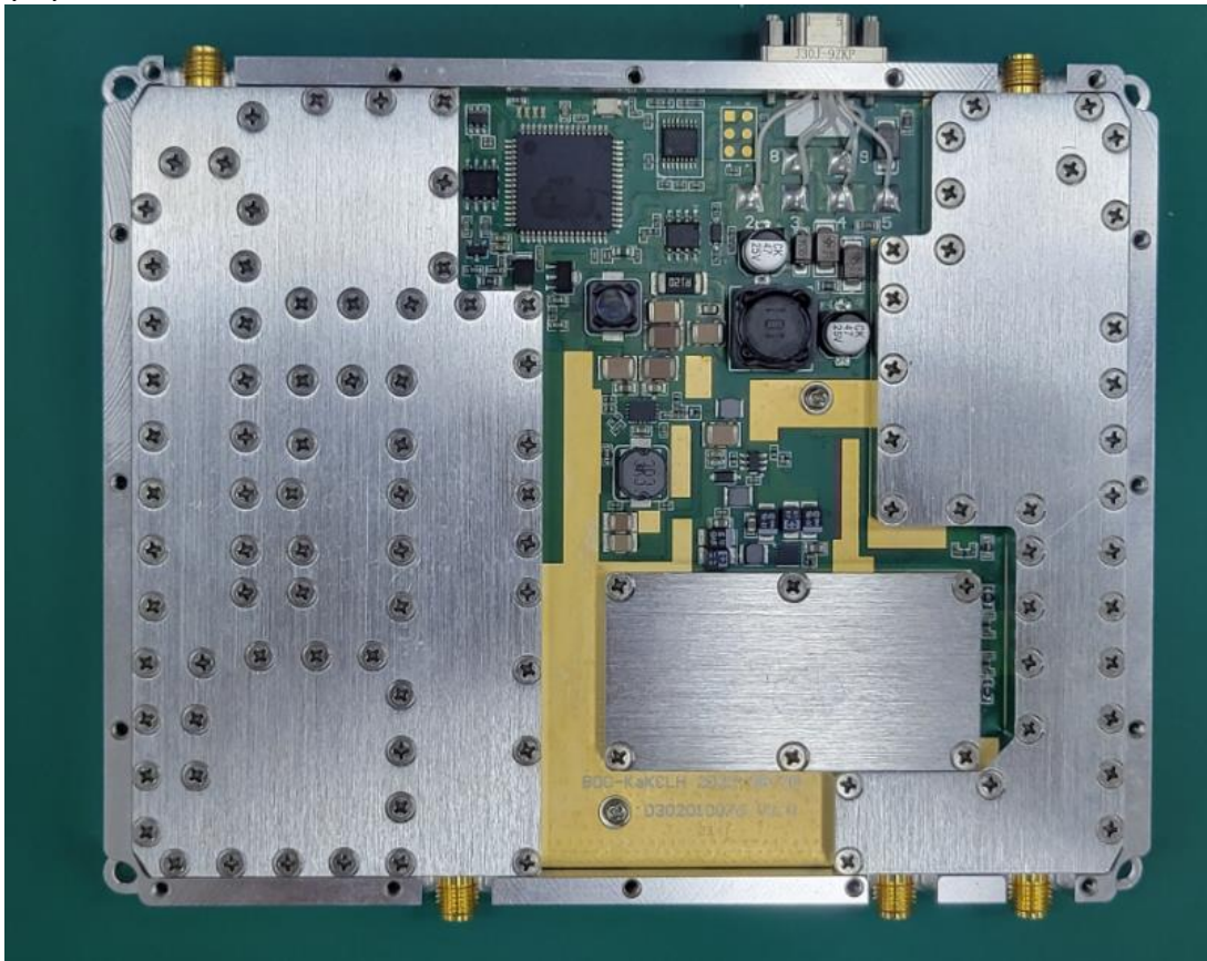
(28) EUT Photo
