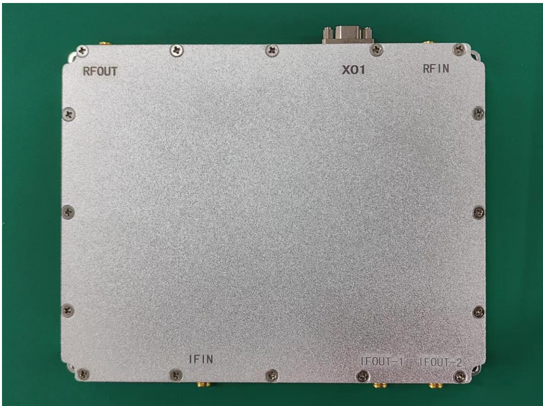
(26) EUT Photo
