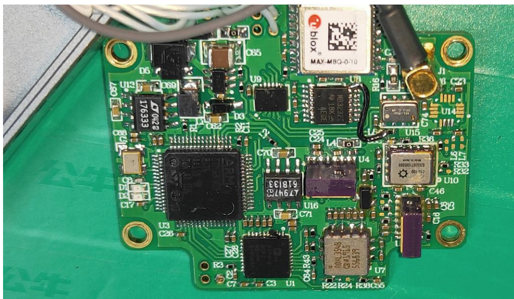
(22) EUT Photo
