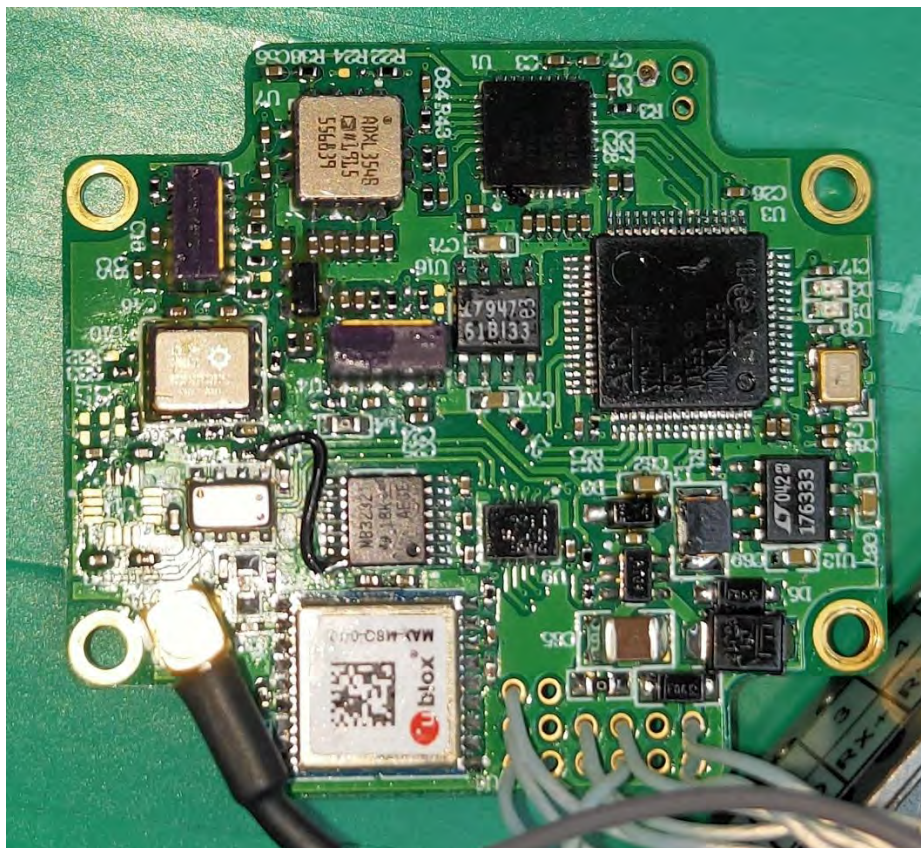
(42) EUT Photo
