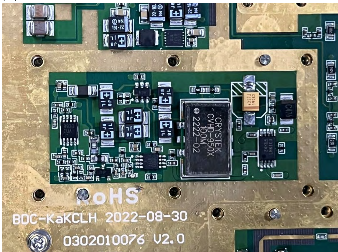
(34) EUT Photo
