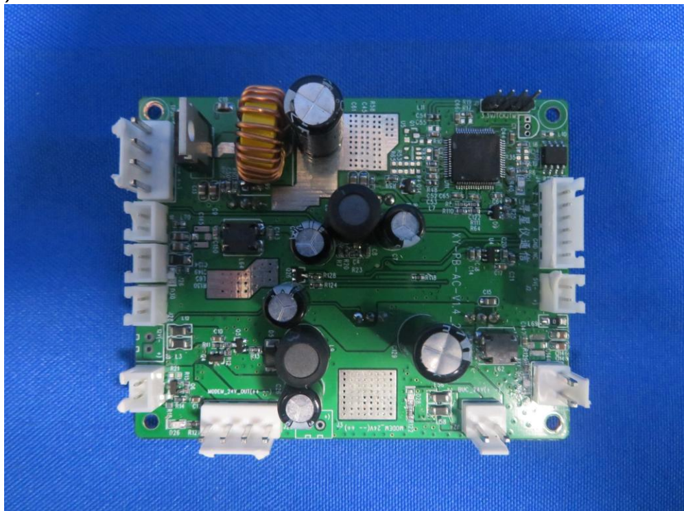
(34) EUT Photo
