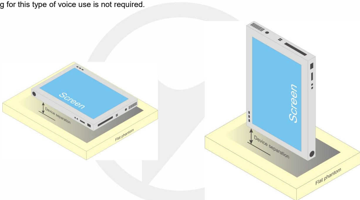
Fig-4.1 Illustration for Tablet Setup
