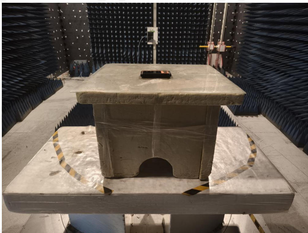
Radiation Test Setup photo(above 1000MHz)
