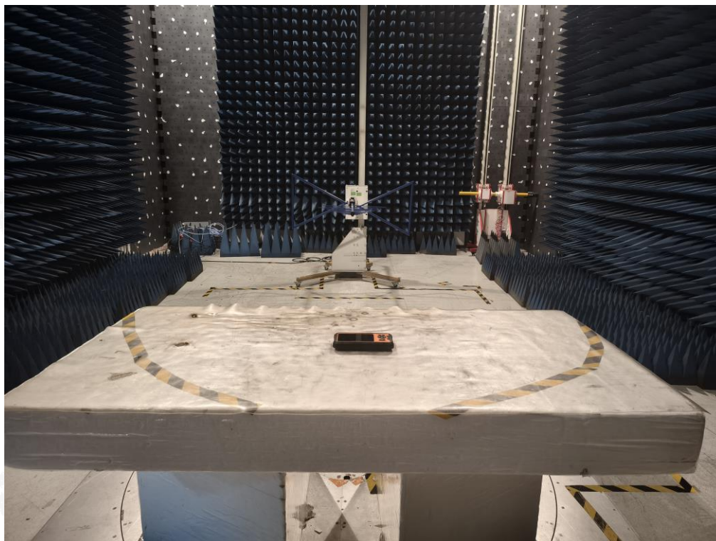
Radiation Test Setup photo(30-1000MHz)
