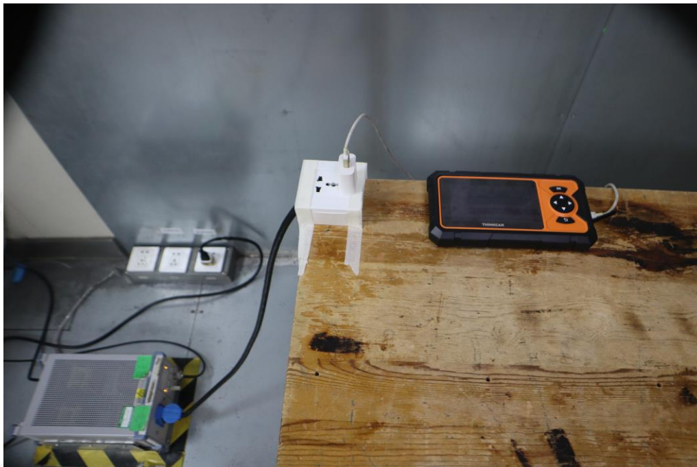
Radiation Test Setup photo(30-1000MHz)
