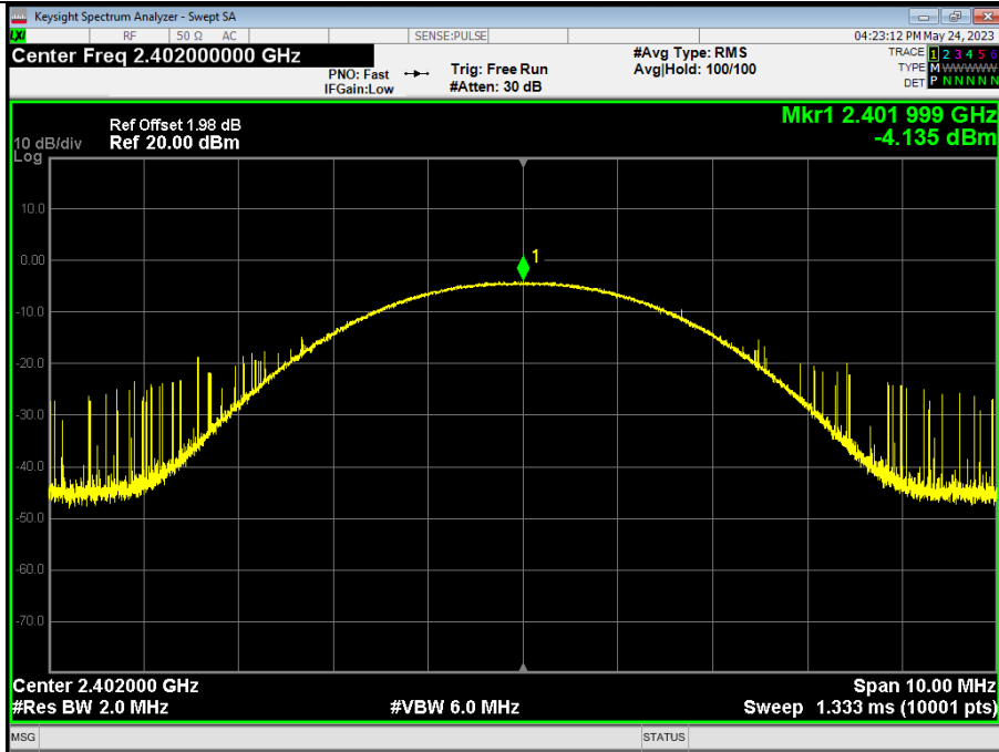
Pi/4DQPSK_2DH5_LCH_2402MHz_Ant1_NTNV
