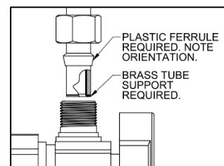
Figure 2: Supply Valve Connection
