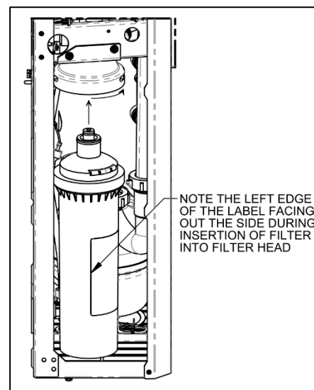
Figure 5: Filter Replacement
