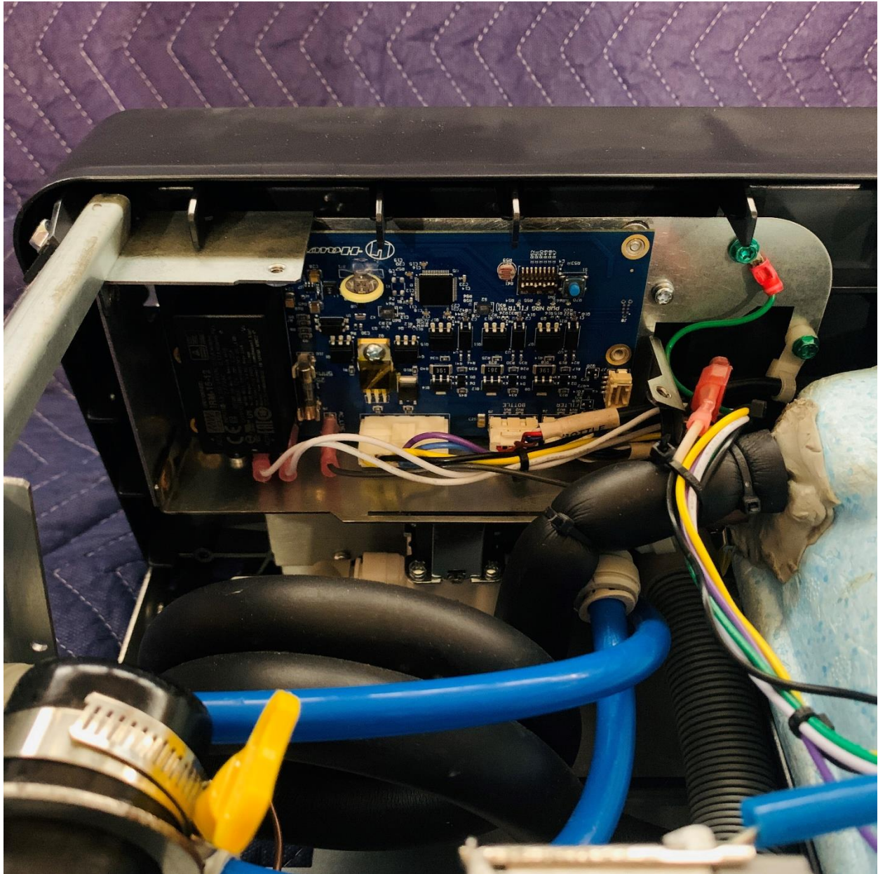
1210SF Main Board (Shown Without Cover)
