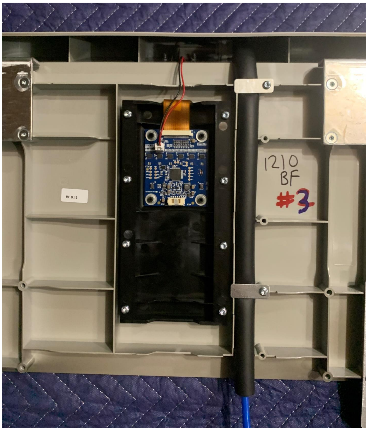
1210SF Rear of Bottle Filler, Bottle Filler Board Shown
