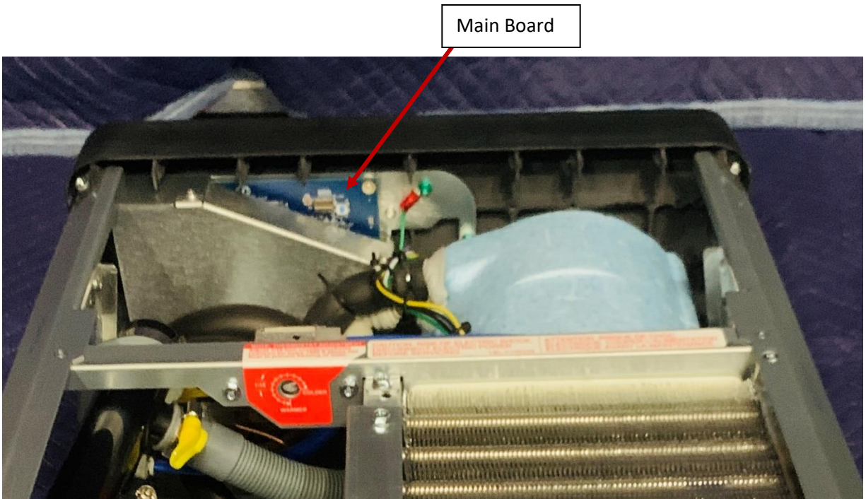
1210SF INTERIOR MAIN BOARD
