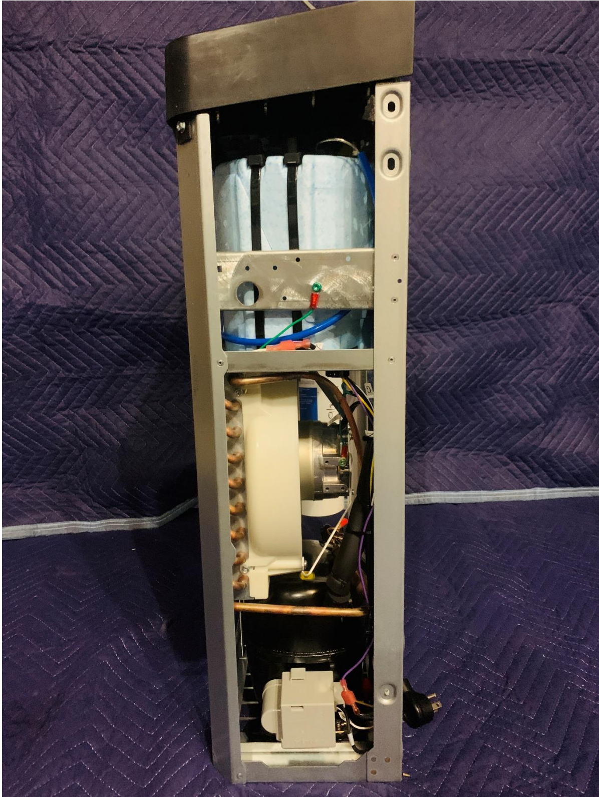
1210SF INTERIOR RIGHT SIDE
