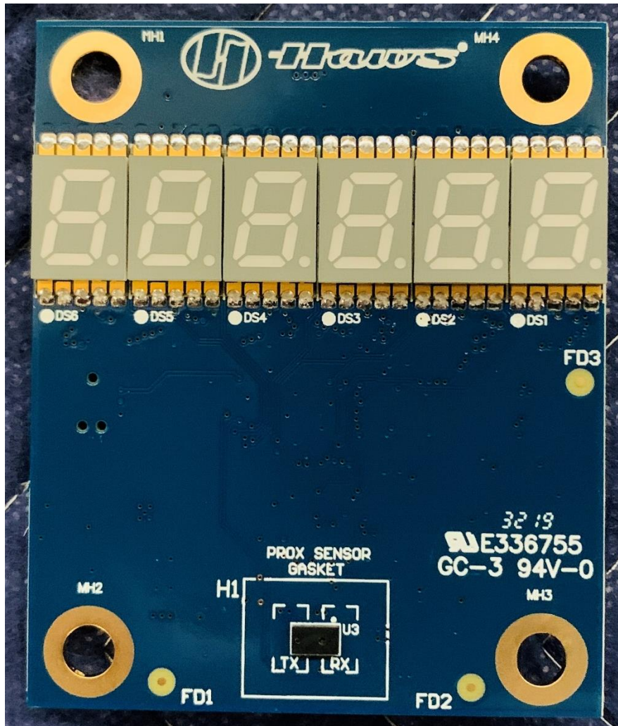
Bottle Filler Board Front (0210000744)
