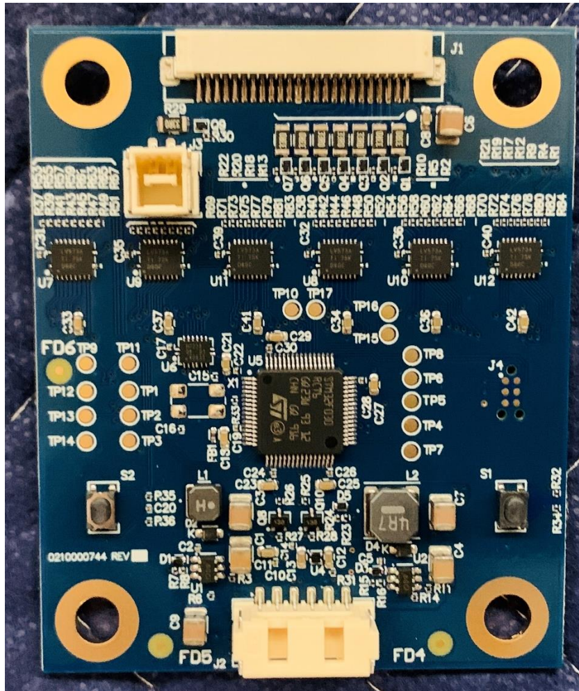
Bottle Filler Board Rear (0210000744)
