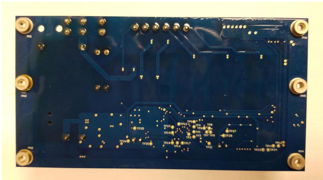
Figure 2 - EWC Board Back (0210000743)
