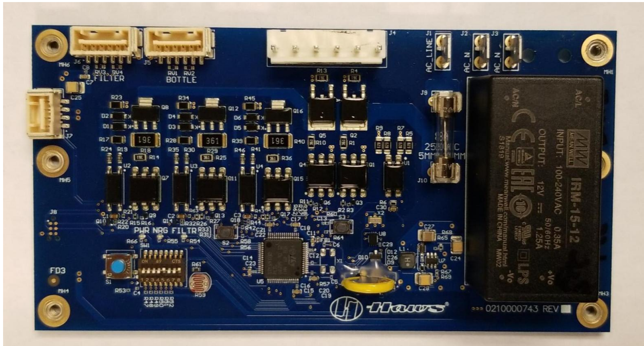
Figure 1 - EWC Board Front (0210000743)
