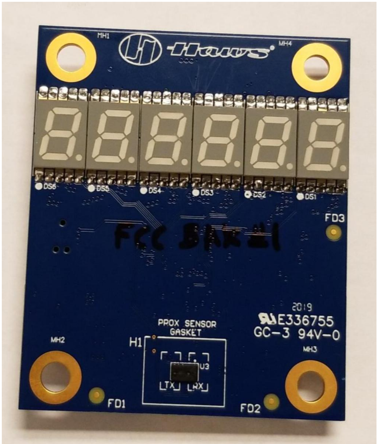
Figure 3 - BF Board Front (0210000744)
