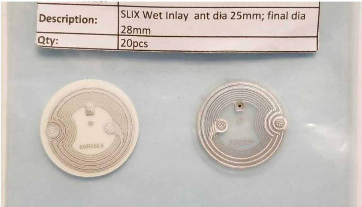
Figure 10 – RFID Tag Front and Back (0210000822) – IDENTIV 25mm Wet Inlay (NXP – SLIX)
