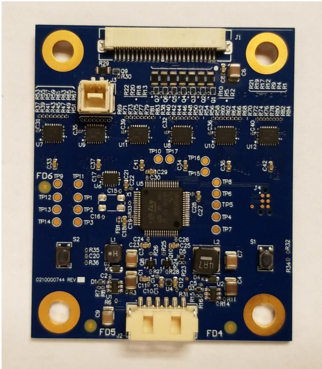
Figure 4 - BF Board Back (0210000744)
