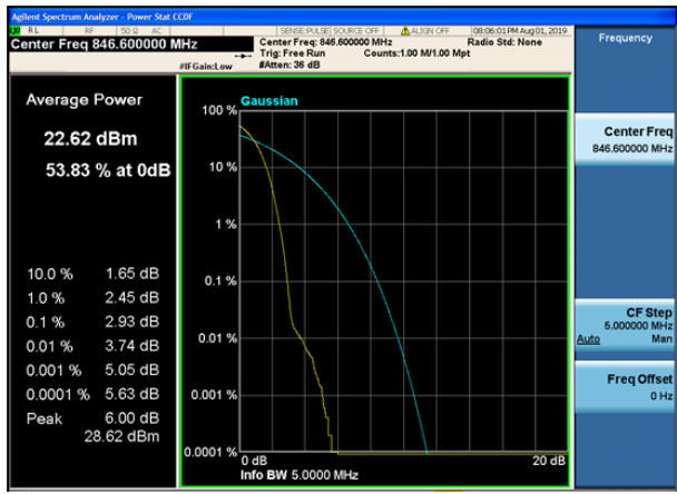
Channel 4233 / 846.6 MHz
