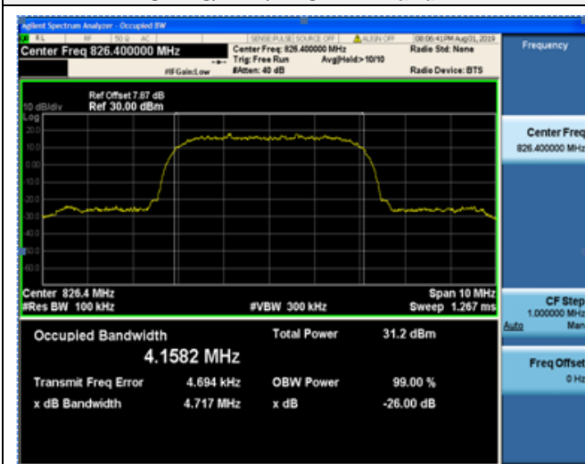
Channel 4132 / 826.4 MHz
