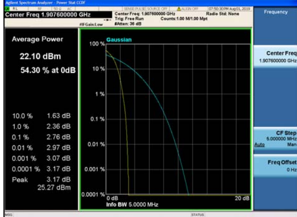
Channel 9538 / 1907.6 MHz
