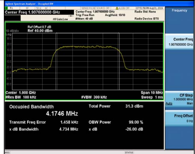
Channel 9538 / 1907.6 MHz
