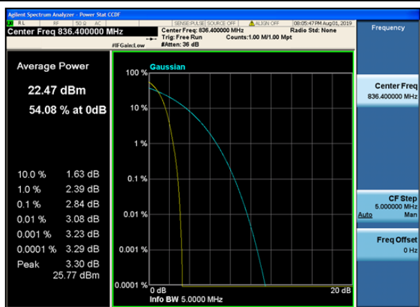
Channel 4183 / 836.4 MHz
