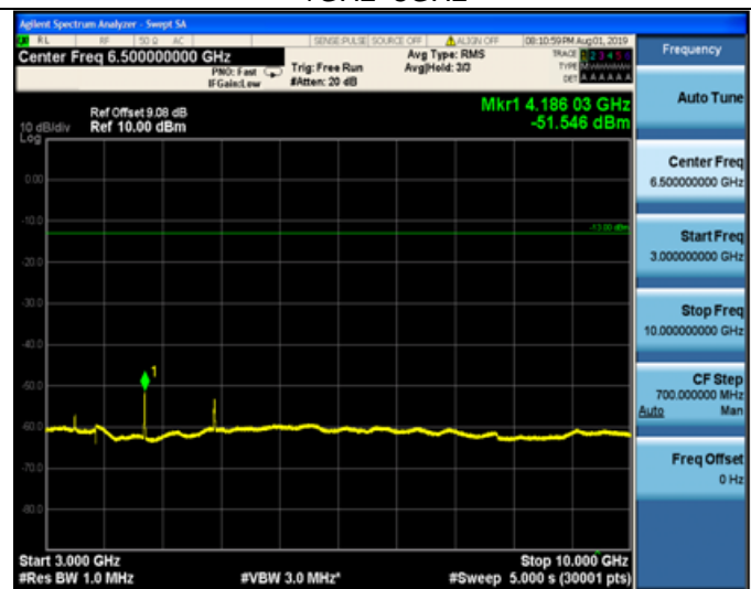
3GHz-10GHz
