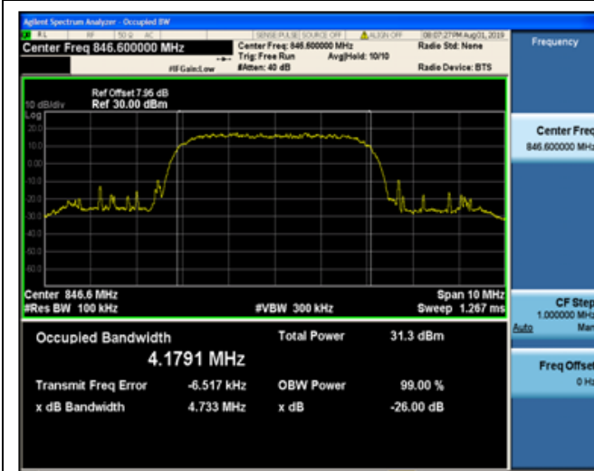
Channel 4233 / 846.6 MHz
