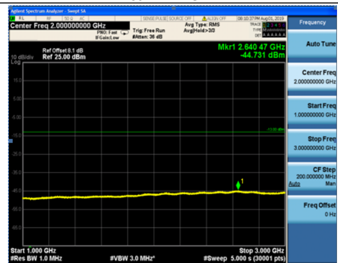
1GHz-3GHz
