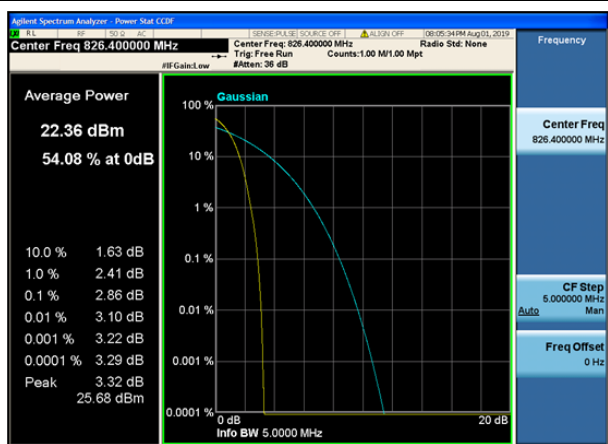
Channel 4132 / 826.4 MHz
