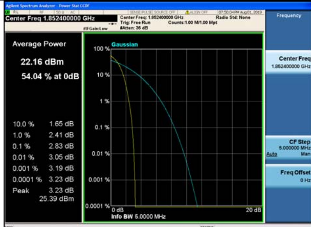
Channel 9262 / 1852.4 MHz
