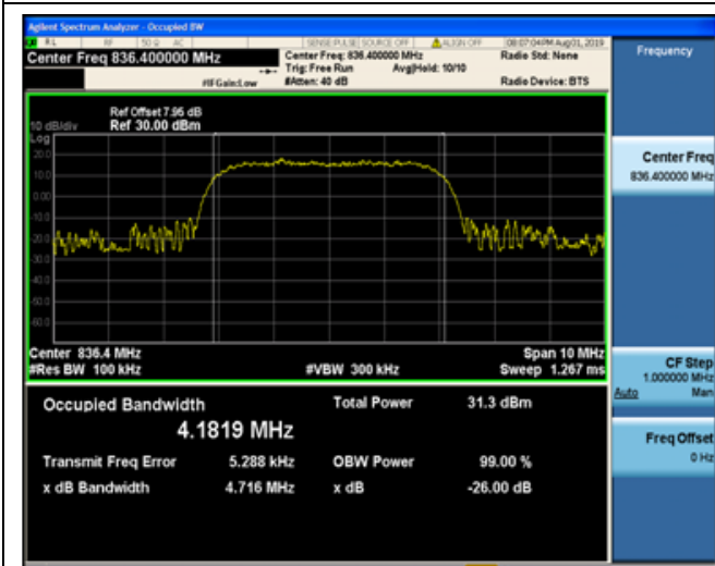
Channel 4183 / 836.4 MHz
