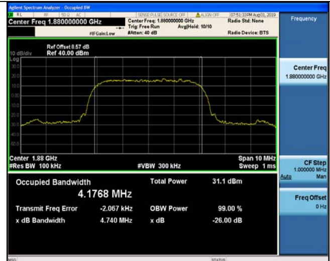
Channel 9400 / 1880.0 MHz
