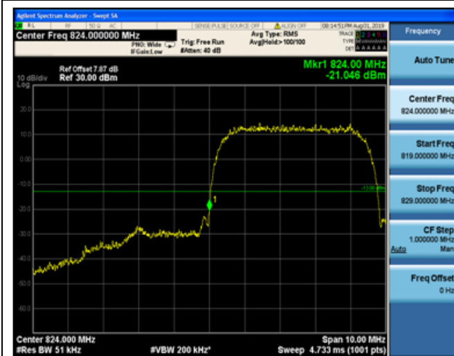
Channel 4132 / 826.4 MHz
