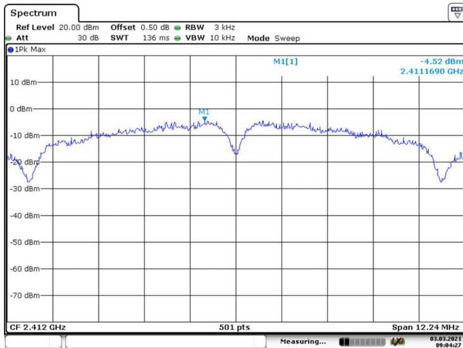
Chain 0, Power Spectral Density, 802.11b Low Channel
