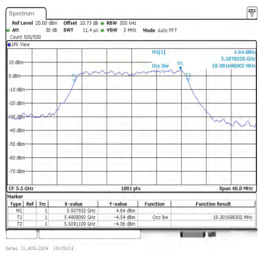
11N20SISO-Ant1-5500
