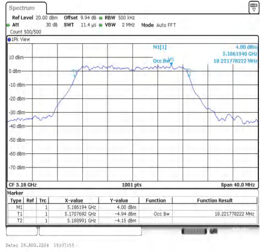
11N20SISO-Ant1-5180
