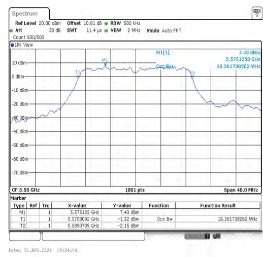
11N20SISO-Ant1-5580
