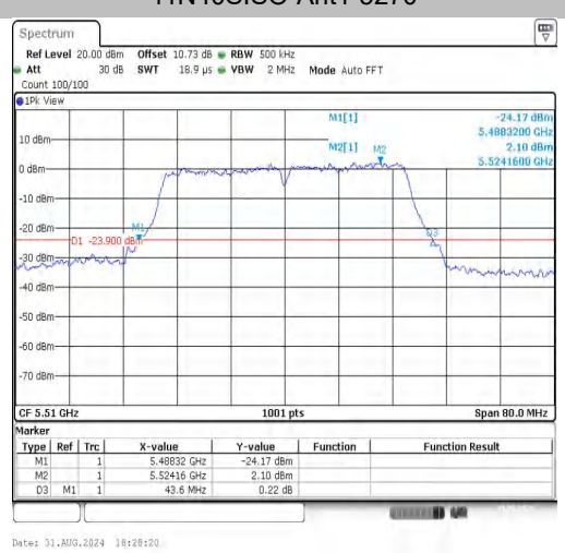
11N40SISO-Ant1-5510
