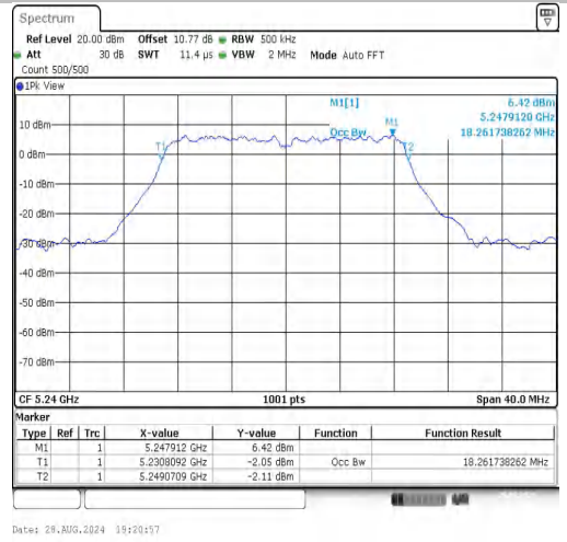
11N20SISO-Ant1-5240
