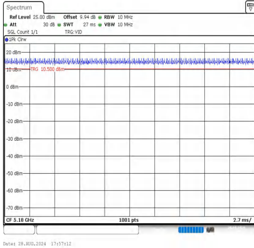
NTNV-11A-Ant1-5180
