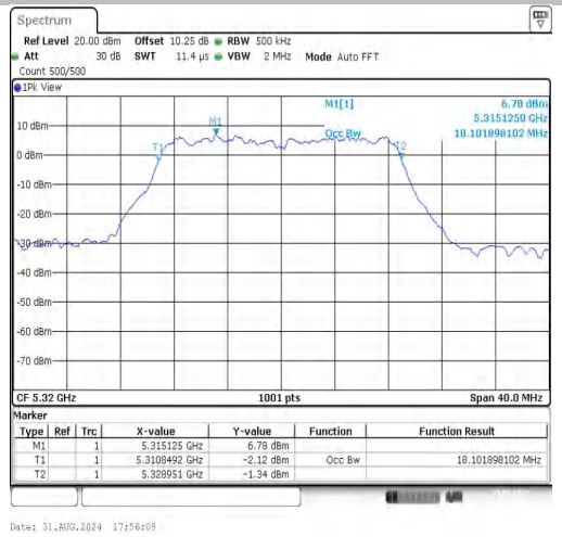
11N20SISO-Ant1-5320
