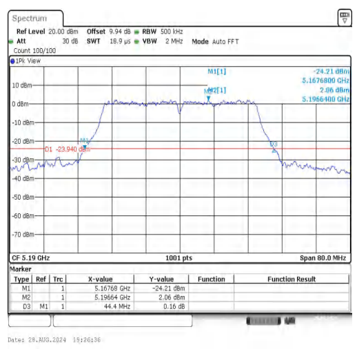
11N40SISO-Ant1-5190
