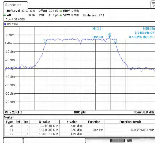
11N40SISO-Ant1-5230
