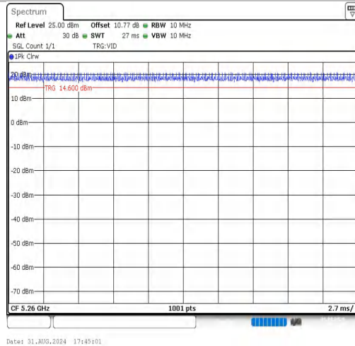
NTNV-11A-Ant1-5260
