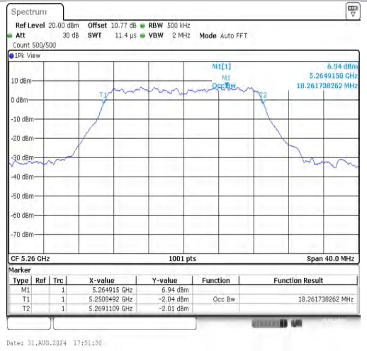
11N20SISO-Ant1-5260
