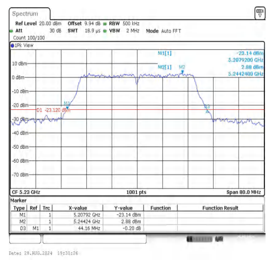
11N40SISO-Ant1-5230
