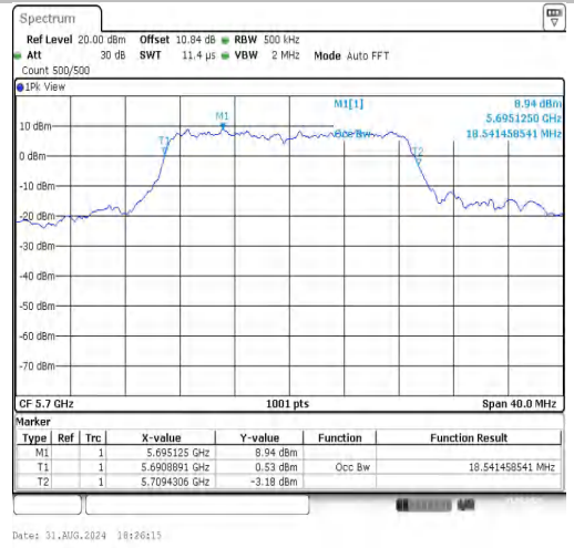
11N20SISO-Ant1-5700
