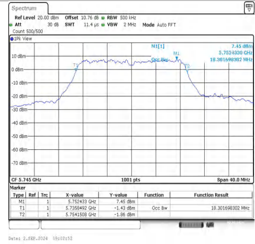
11N20SISO-Ant1-5745
