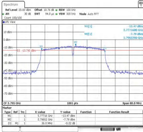
11AC40SISO-Ant1-5795-PASS
