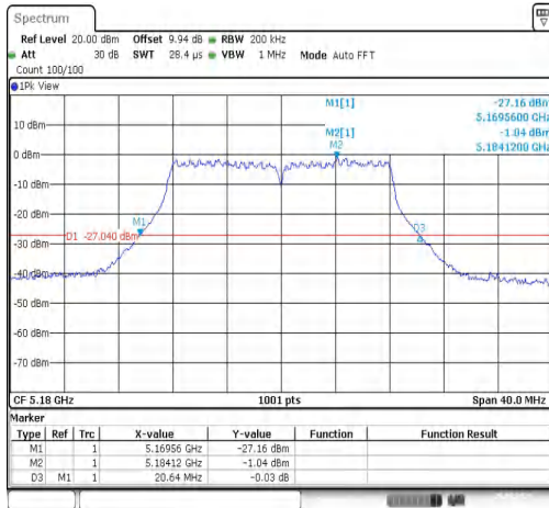
11A-Ant1-5180
