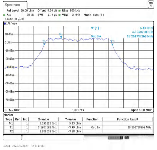
11N20SISO-Ant1-5200
