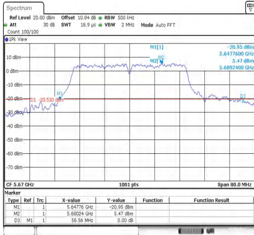
11N40SISO-Ant1-5670
