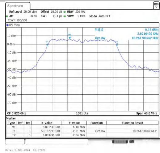
11N20SISO-Ant1-5825
