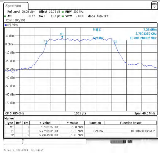
11N20SISO-Ant1-5785
