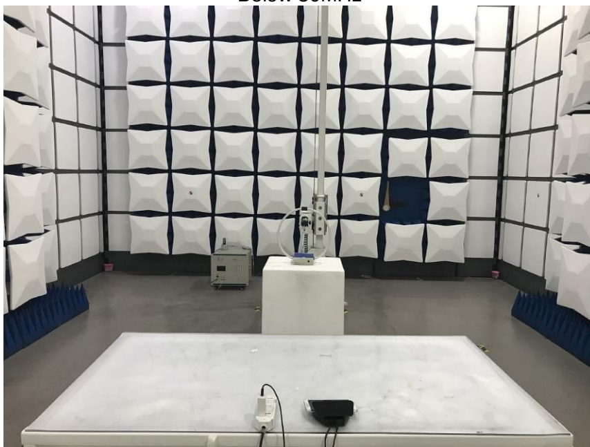
Below 30MHz
