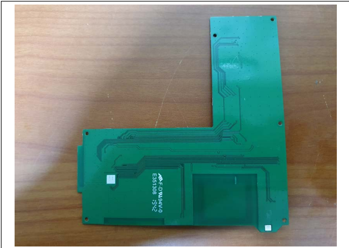
MainBoard-Rear
