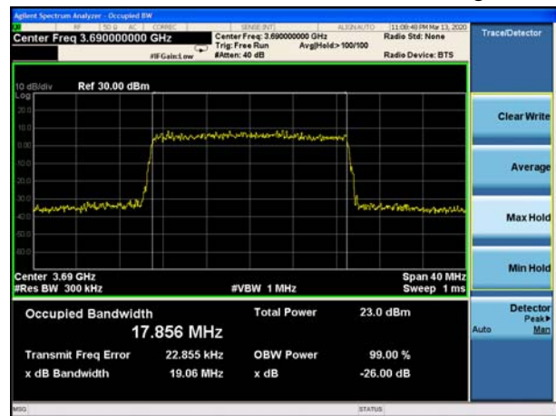
LTE Band 48 20MHz 16QAM CH-High
