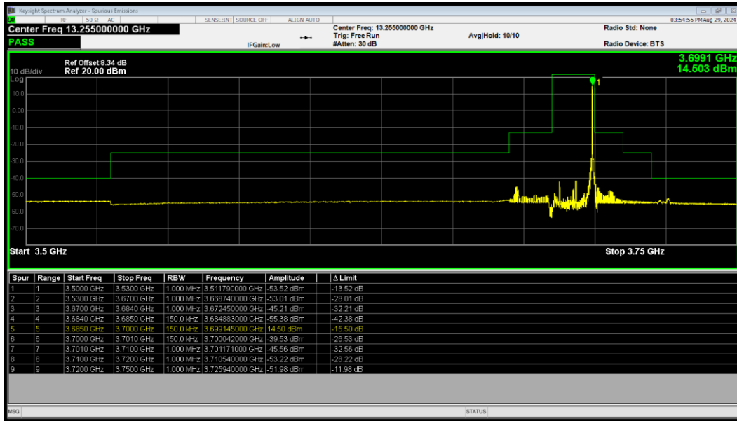
LTE Band 48 64QAM BW=15MHz HighChannel=56665 RB Size=1 Position=#Max
