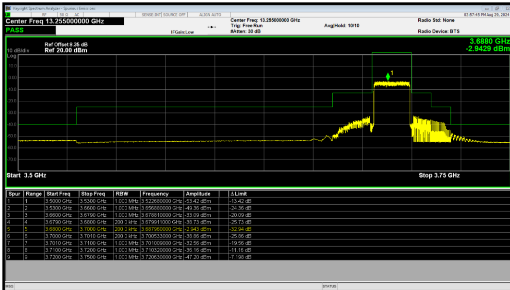
LTE Band 48 QPSK BW=20MHz HighChannel=56640 RB Size=100 Position=#0
