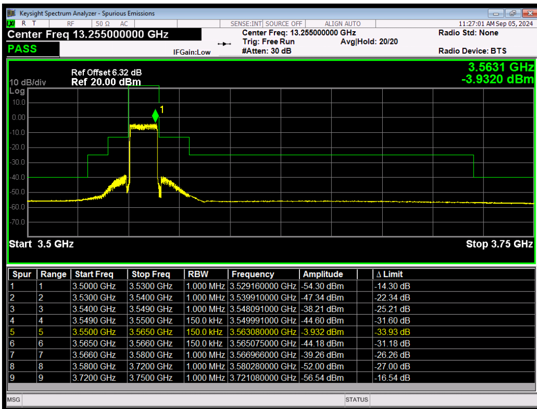
LTE Band 48 256QAM BW=15MHz LowChannel=55315 RB Size=75 Position=#0
