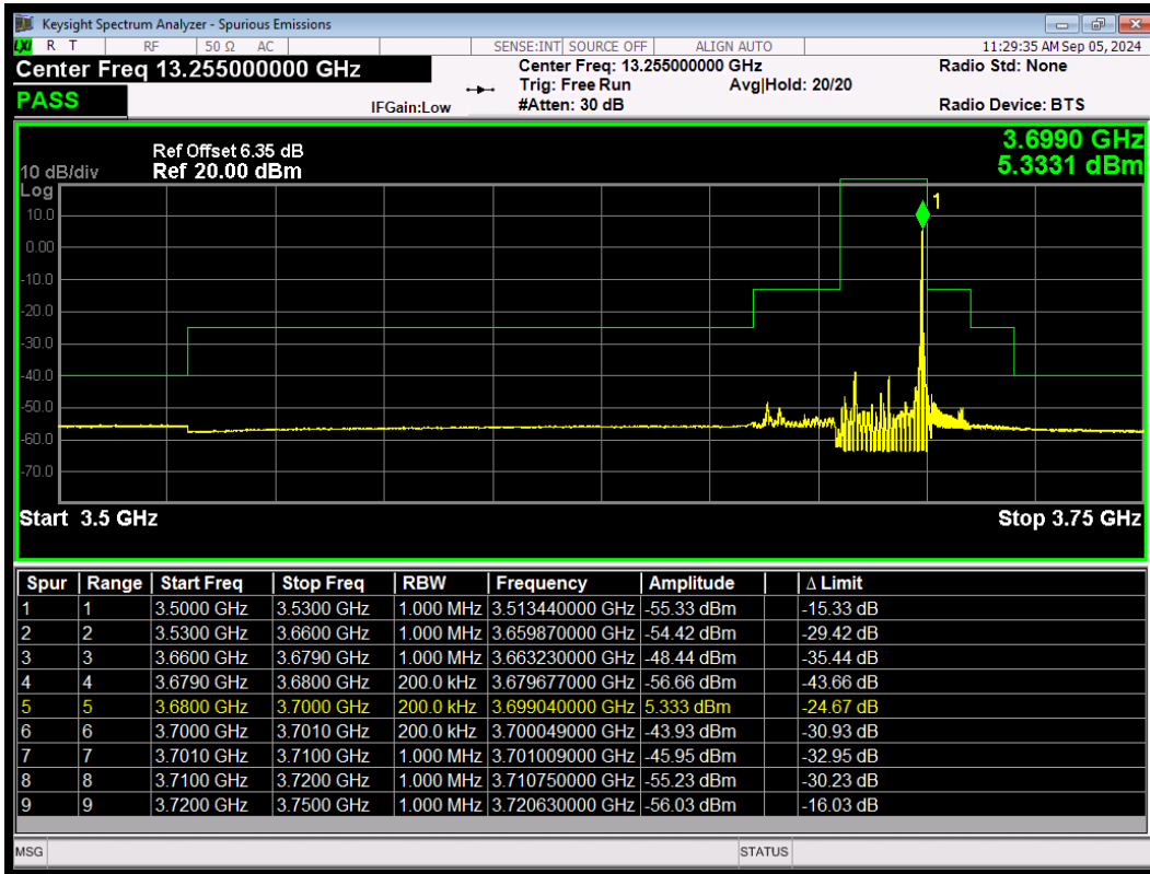
LTE Band 48 256QAM BW=20MHz HighChannel=56640 RB Size=1 Position=#Max
