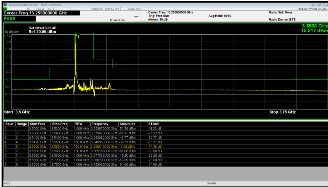
LTE Band 48 16QAM BW=15MHz LowChannel=55315 RB Size=1 Position=#0
