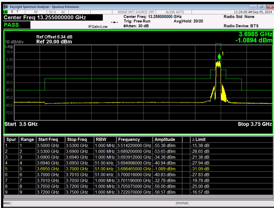
LTE Band 48 256QAM BW=5MHz HighChannel=56715 RB Size=25 Position=#0
