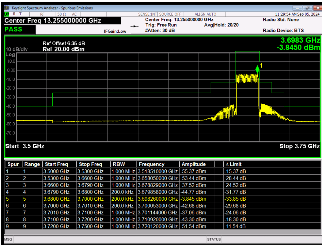
LTE Band 48 256QAM BW=20MHz HighChannel=56640 RB Size=100 Position=#0
