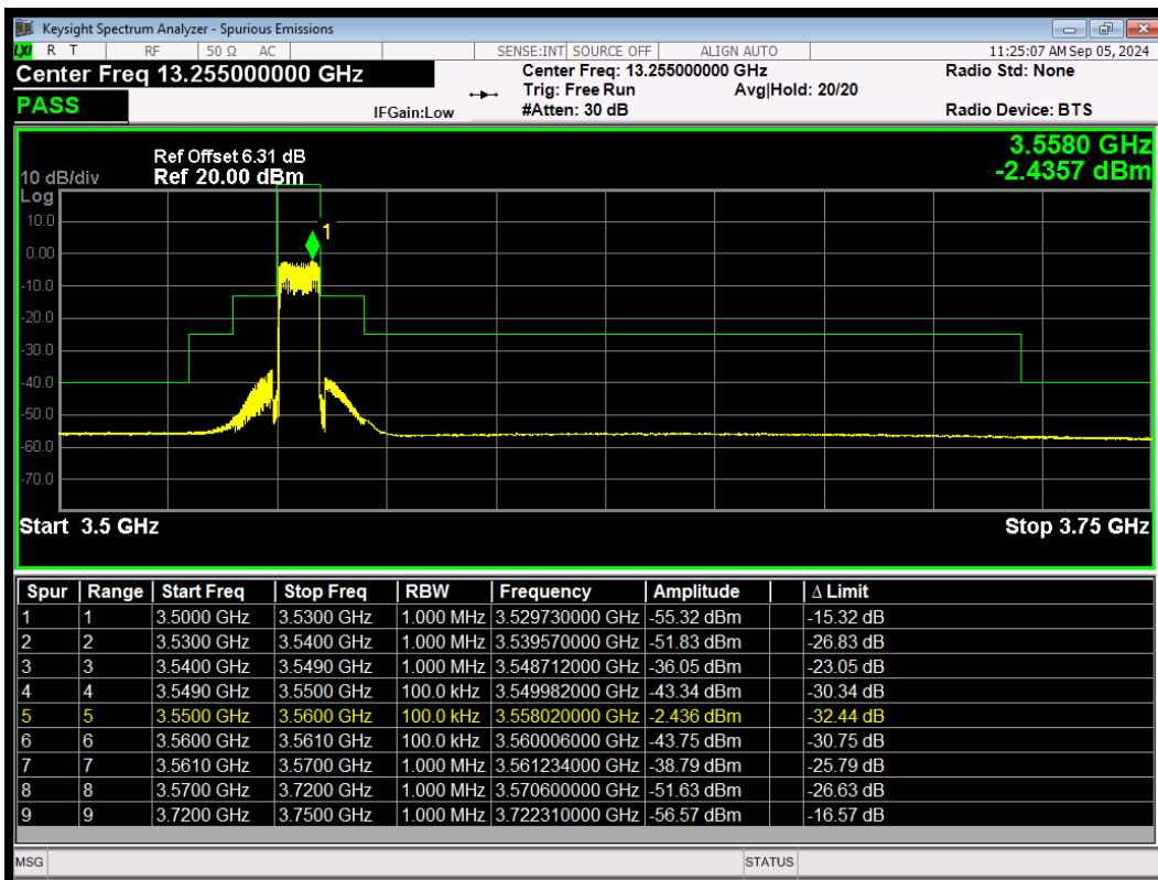
LTE Band 48 256QAM BW=10MHz LowChannel=55290 RB Size=50 Position=#0
