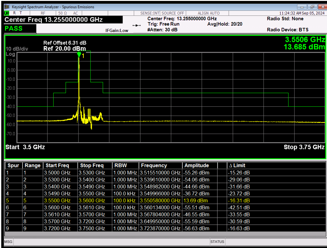
LTE Band 48 256QAM BW=10MHz LowChannel=55290 RB Size=1 Position=#0
