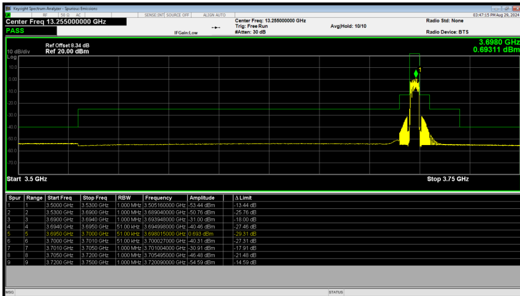
LTE Band 48 64QAM BW=5MHz HighChannel=56715 RB Size=25 Position=#0
