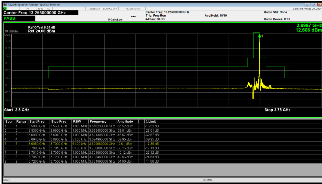
LTE Band 48 64QAM BW=5MHz HighChannel=56715 RB Size=1 Position=#Max
