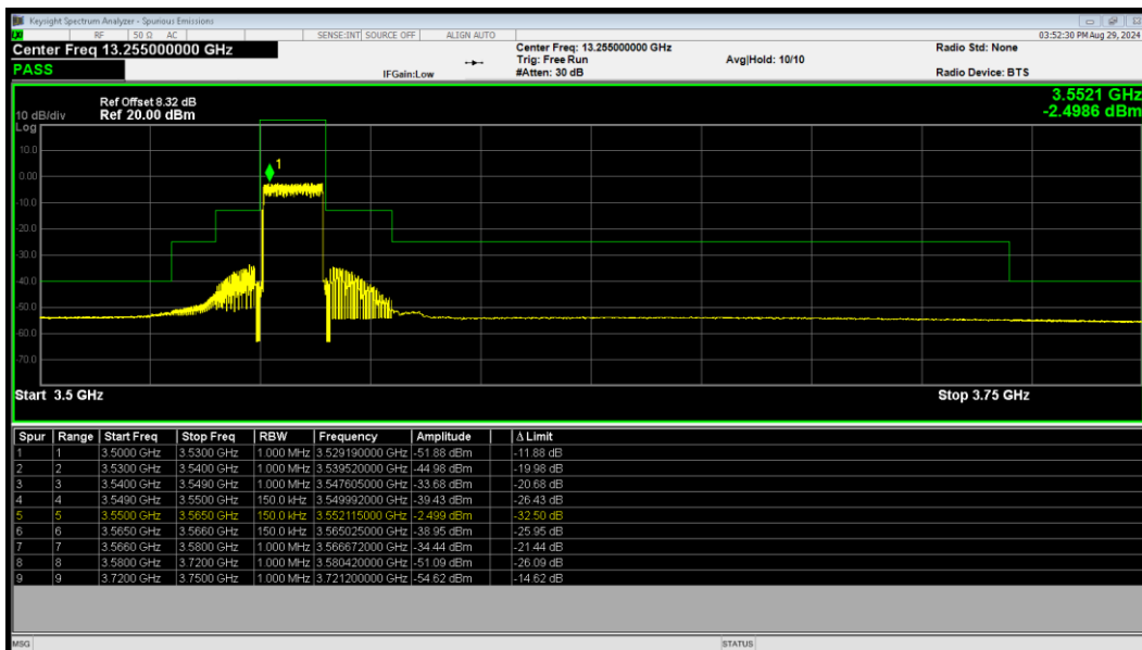
LTE Band 48 16QAM BW=15MHz LowChannel=55315 RB Size=75 Position=#0
