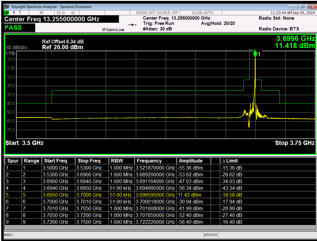
LTE Band 48 256QAM BW=5MHz HighChannel=56715 RB Size=1 Position=#Max
