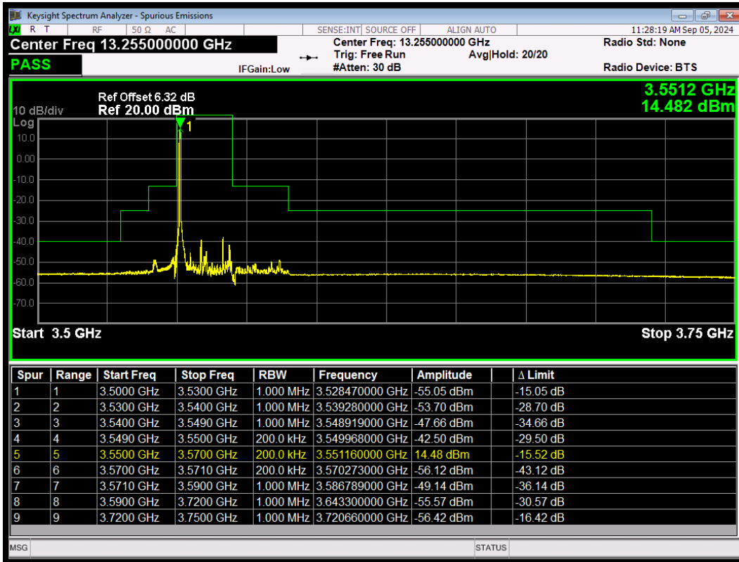
LTE Band 48 256QAM BW=20MHz LowChannel=55340 RB Size=1 Position=#0
