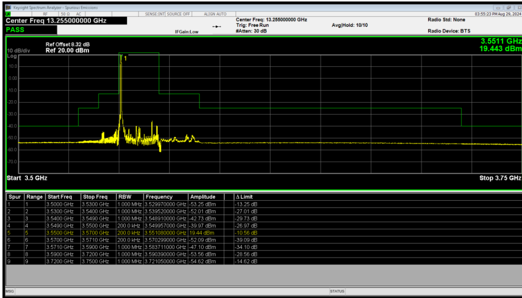
LTE Band 48 QPSK BW=20MHz LowChannel=55340 RB Size=1 Position=#0
