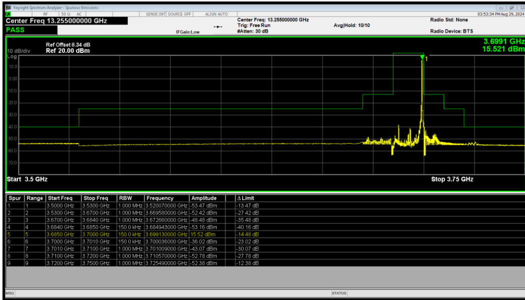
LTE Band 48 QPSK BW=15MHz HighChannel=56665 RB Size=1 Position=#Max
