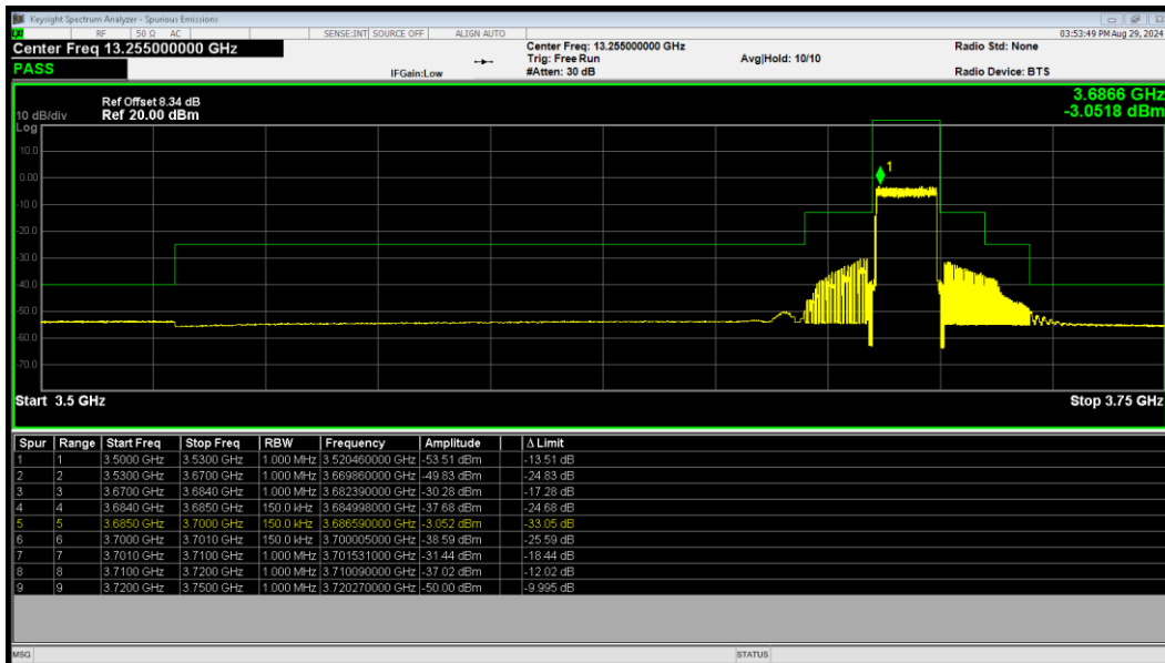
LTE Band 48 QPSK BW=15MHz HighChannel=56665 RB Size=75 Position=#0
