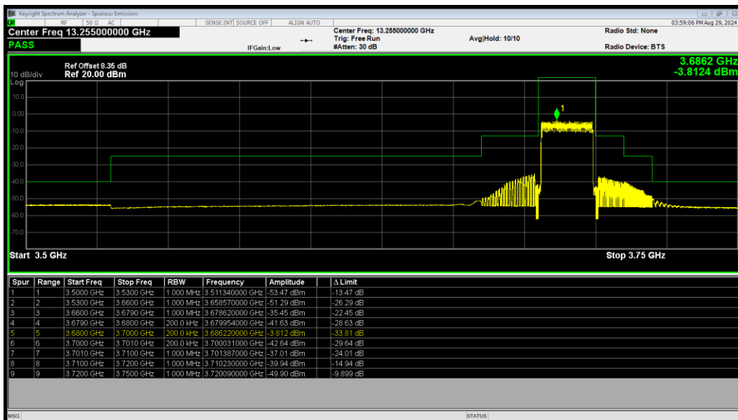
LTE Band 48 64QAM BW=20MHz HighChannel=56640 RB Size=100 Position=#0
