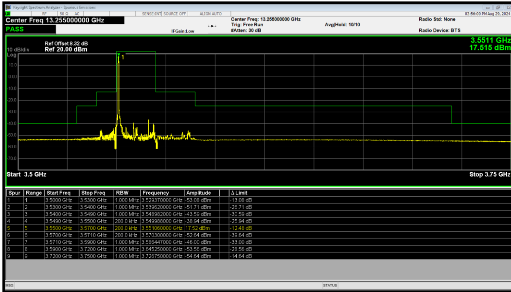
LTE Band 48 16QAM BW=20MHz LowChannel=55340 RB Size=1 Position=#0
