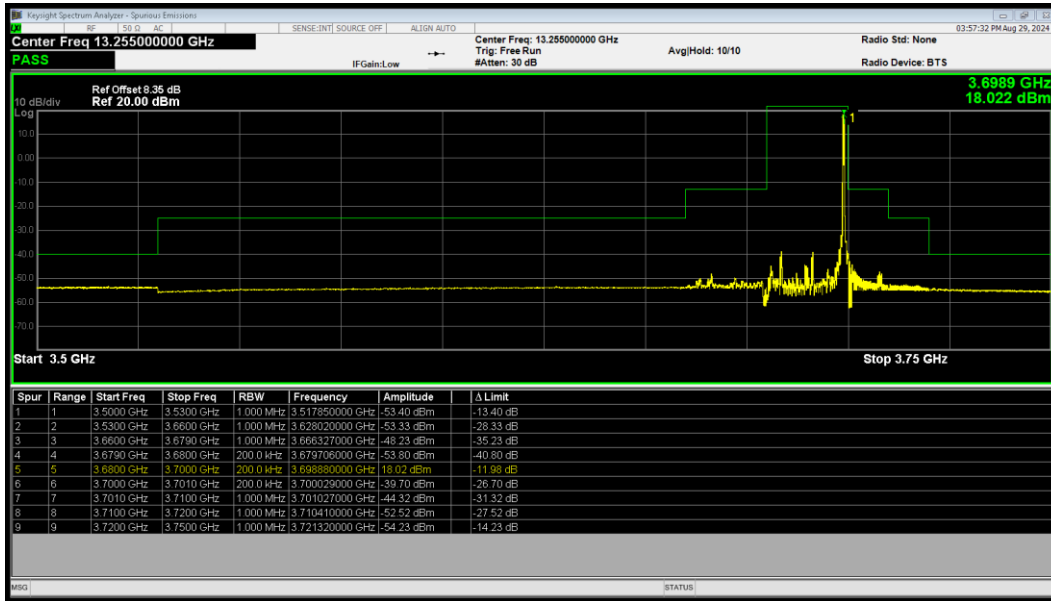
LTE Band 48 QPSK BW=20MHz HighChannel=56640 RB Size=1 Position=#Max
