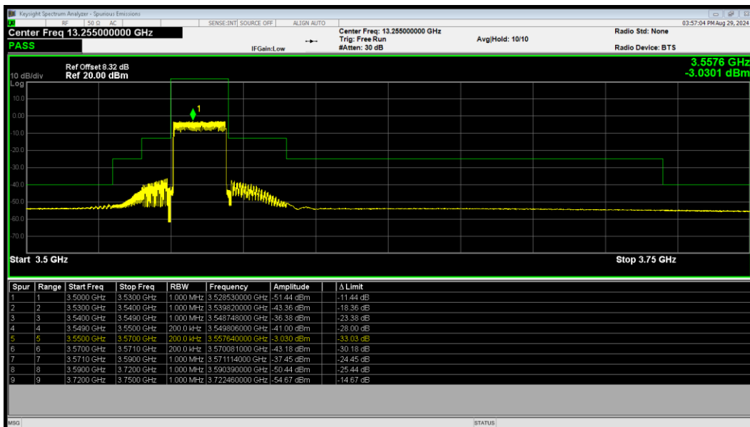
LTE Band 48 64QAM BW=20MHz LowChannel=55340 RB Size=100 Position=#0
