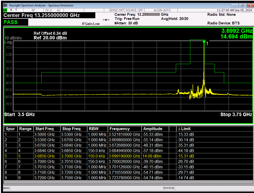
LTE Band 48 256QAM BW=15MHz HighChannel=56665 RB Size=1 Position=#Max
