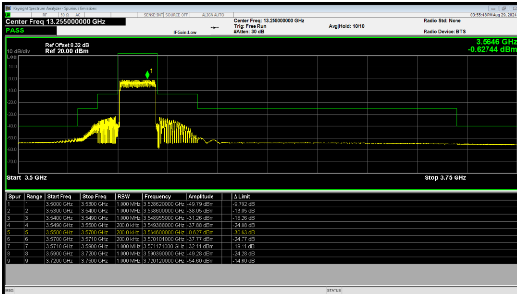
LTE Band 48 QPSK BW=20MHz LowChannel=55340 RB Size=100 Position=#0
