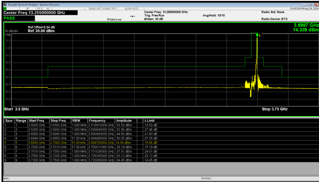
LTE Band 48 QPSK BW=5MHz HighChannel=56715 RB Size=1 Position=#Max
