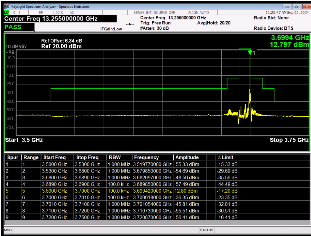
LTE Band 48 256QAM BW=10MHz HighChannel=56690 RB Size=1 Position=#Max
