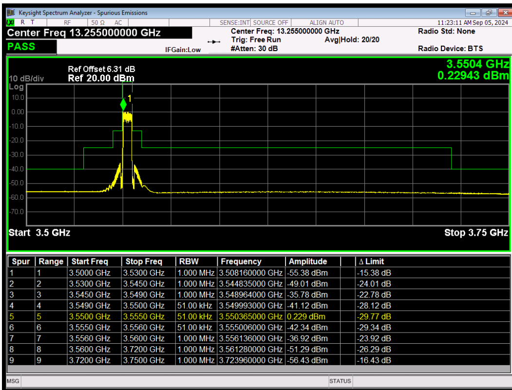
LTE Band 48 256QAM BW=5MHz LowChannel=55265 RB Size=25 Position=#0
