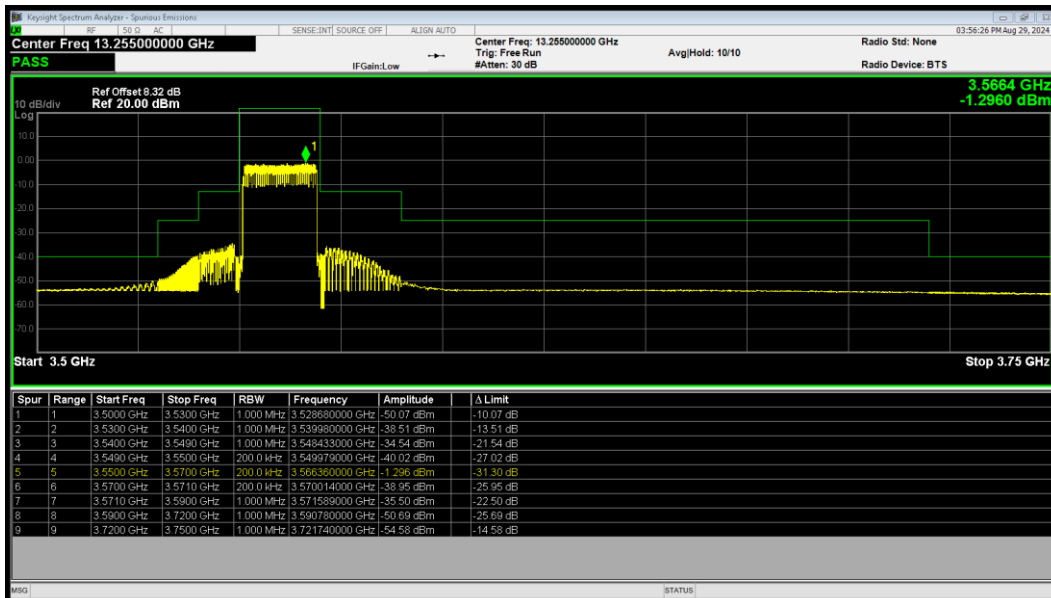
LTE Band 48 16QAM BW=20MHz LowChannel=55340 RB Size=100 Position=#0
