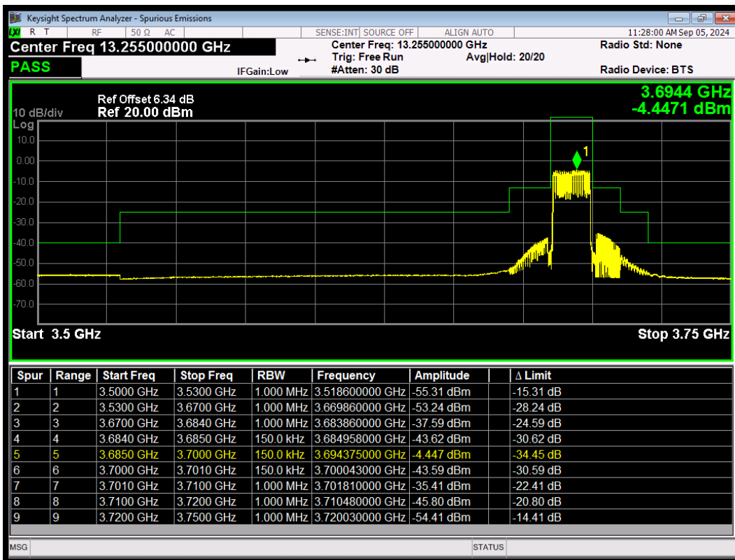
LTE Band 48 256QAM BW=15MHz HighChannel=56665 RB Size=75 Position=#0
