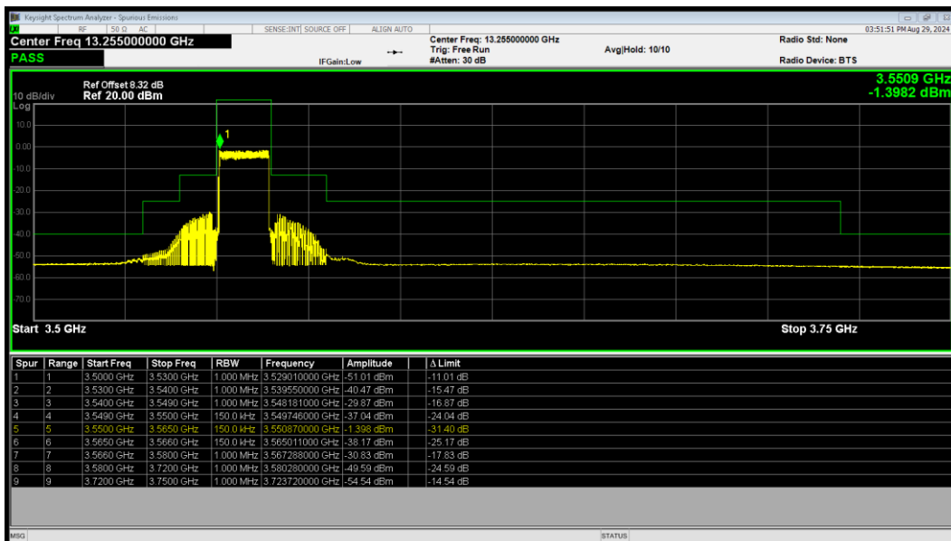
LTE Band 48 QPSK BW=15MHz LowChannel=55315 RB Size=75 Position=#0
