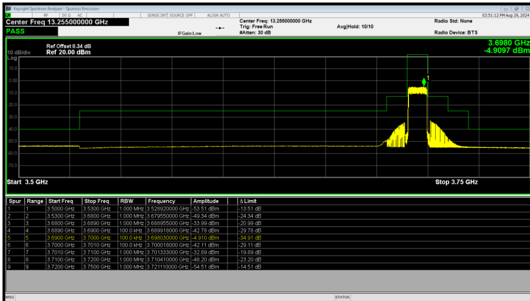
LTE Band 48 64QAM BW=10MHz HighChannel=56690 RB Size=50 Position=#0
