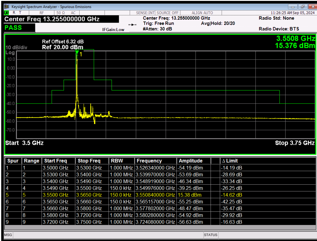
LTE Band 48 256QAM BW=15MHz LowChannel=55315 RB Size=1 Position=#0
