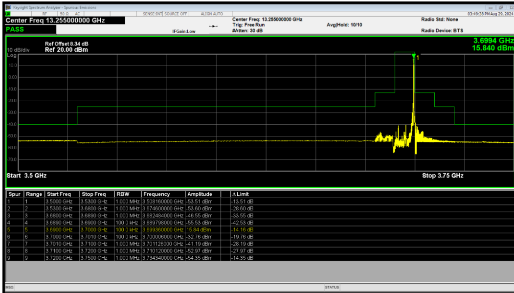
LTE Band 48 QPSK BW=10MHz HighChannel=56690 RB Size=1 Position=#Max
