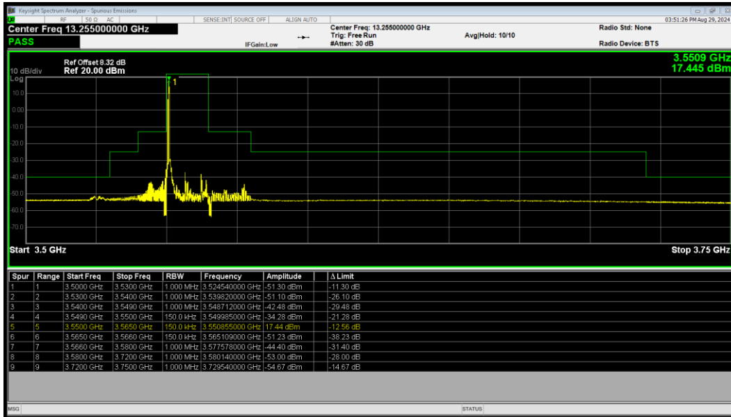
LTE Band 48 QPSK BW=15MHz LowChannel=55315 RB Size=1 Position=#0
