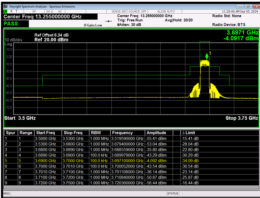
LTE Band 48 256QAM BW=10MHz HighChannel=56690 RB Size=50 Position=#0
