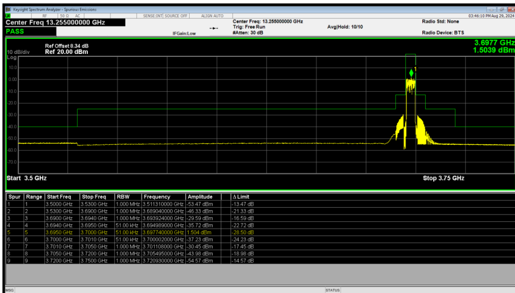
LTE Band 48 QPSK BW=5MHz HighChannel=56715 RB Size=25 Position=#0
