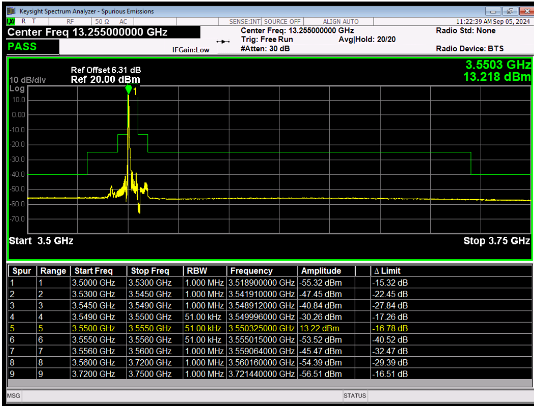
LTE Band 48 256QAM BW=5MHz LowChannel=55265 RB Size=1 Position=#0
