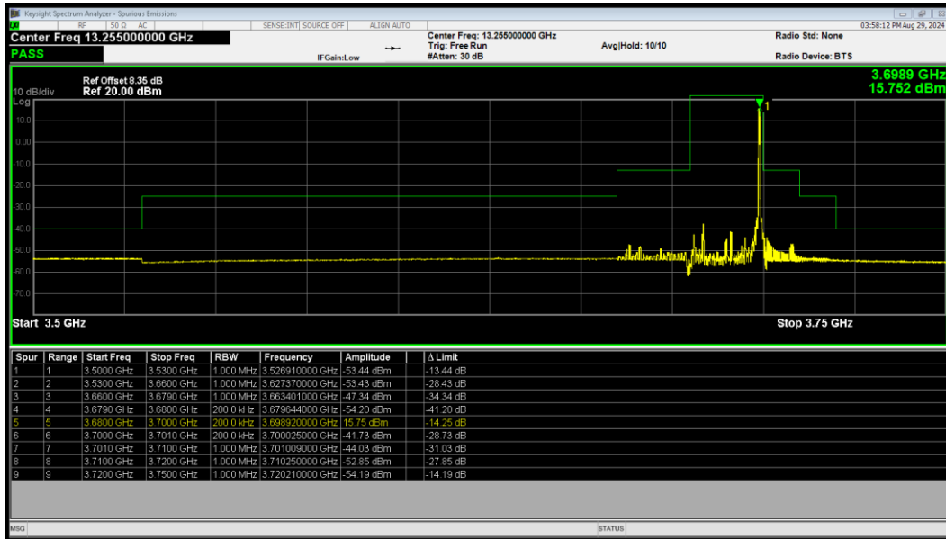
LTE Band 48 16QAM BW=20MHz HighChannel=56640 RB Size=1 Position=#Max
