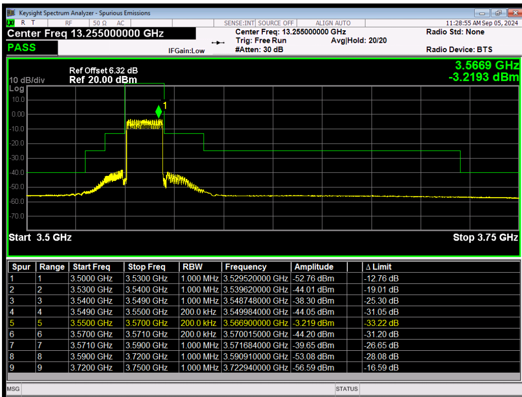
LTE Band 48 256QAM BW=20MHz LowChannel=55340 RB Size=100 Position=#0
