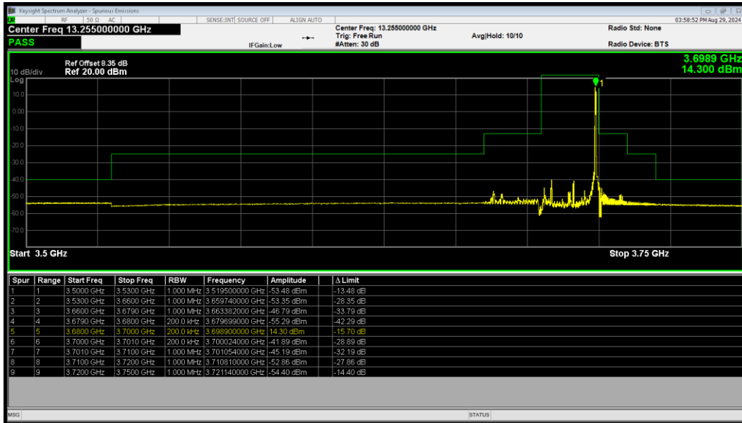
LTE Band 48 64QAM BW=20MHz HighChannel=56640 RB Size=1 Position=#Max
