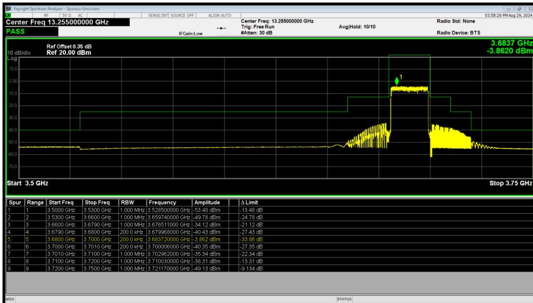
LTE Band 48 16QAM BW=20MHz HighChannel=56640 RB Size=100 Position=#0
