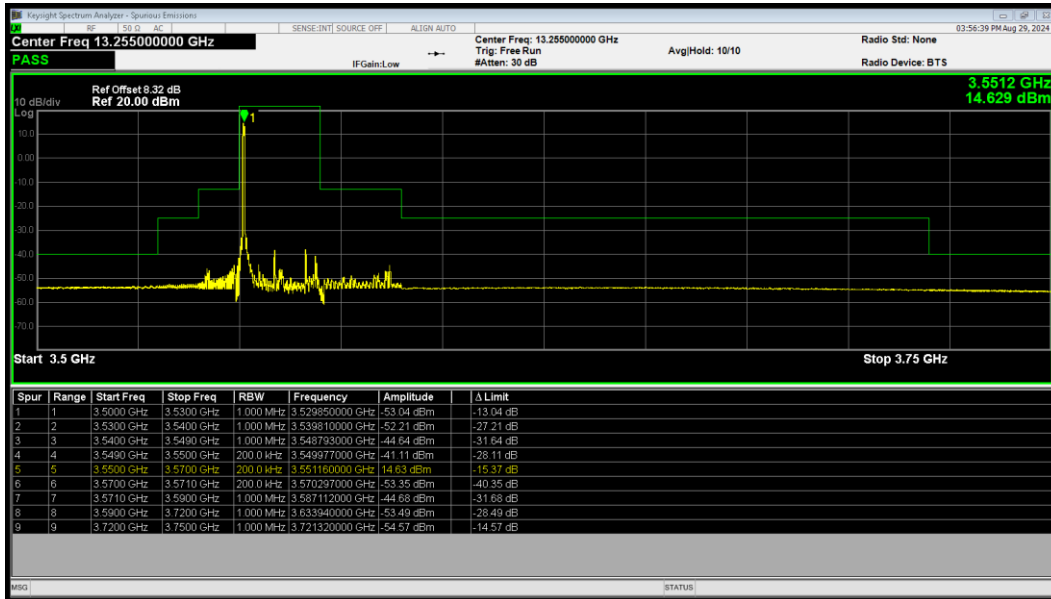
LTE Band 48 64QAM BW=20MHz LowChannel=55340 RB Size=1 Position=#0
