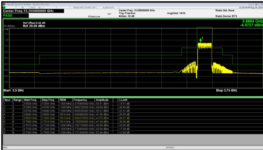
LTE Band 48 64QAM BW=15MHz HighChannel=56665 RB Size=75 Position=#0
