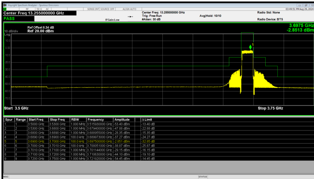
LTE Band 48 QPSK BW=10MHz HighChannel=56690 RB Size=50 Position=#0
