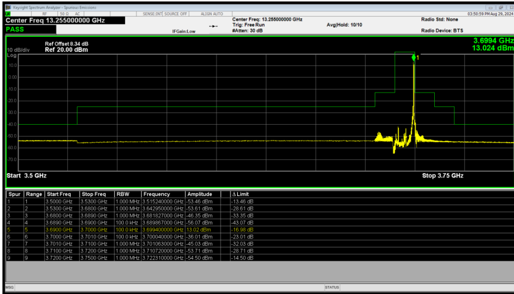
LTE Band 48 64QAM BW=10MHz HighChannel=56690 RB Size=1 Position=#Max
