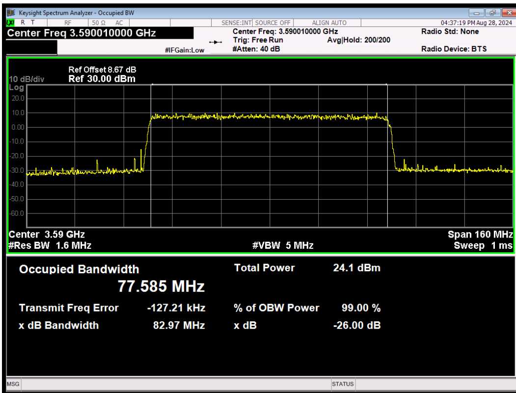
MIMO\PC3\NR n48 SCS=30kHz CP_256QAM BW=80MHz Channel=639334 RB=217@0
