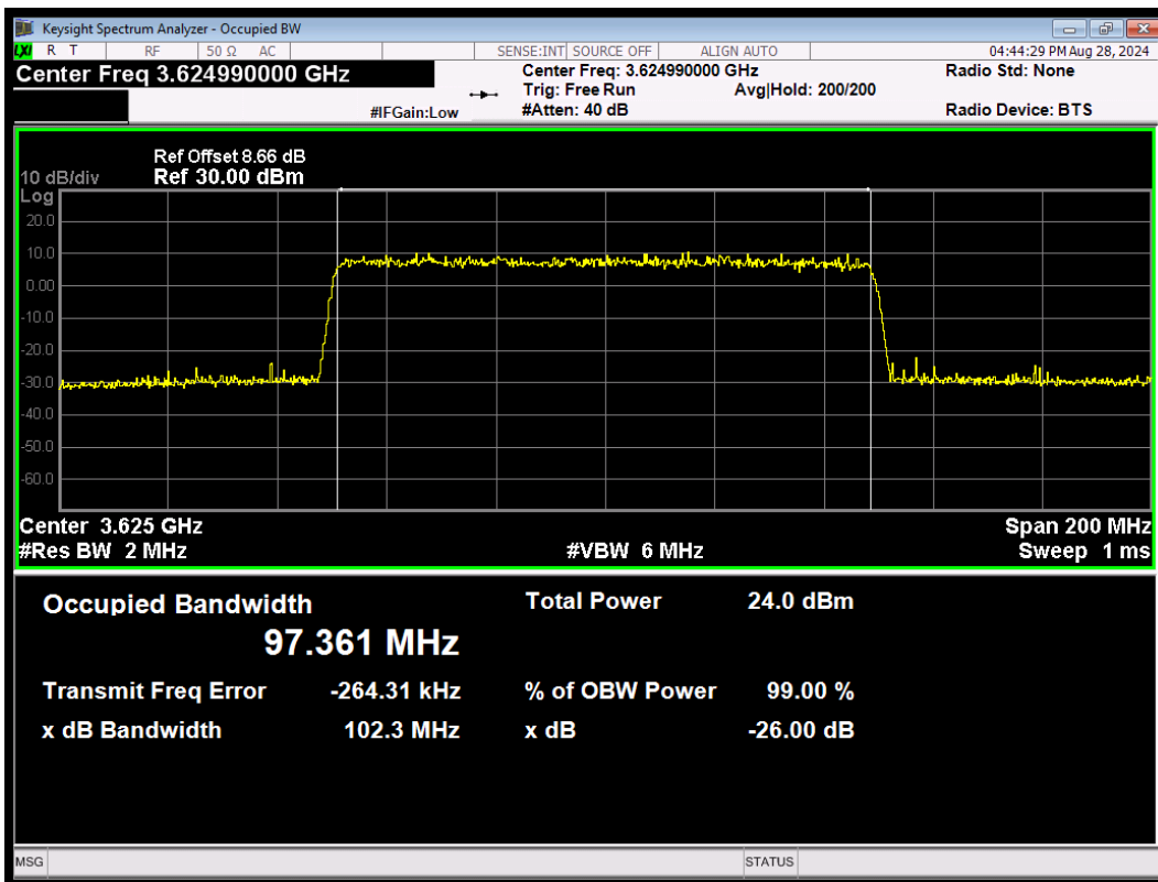
MIMO\PC3\NR n48 SCS=30kHz CP_256QAM BW=100MHz Channel=641666 RB=273@0
