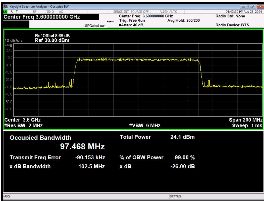
MIMO\PC3\NR n48 SCS=30kHz CP_256QAM BW=100MHz Channel=640000 RB=273@0
