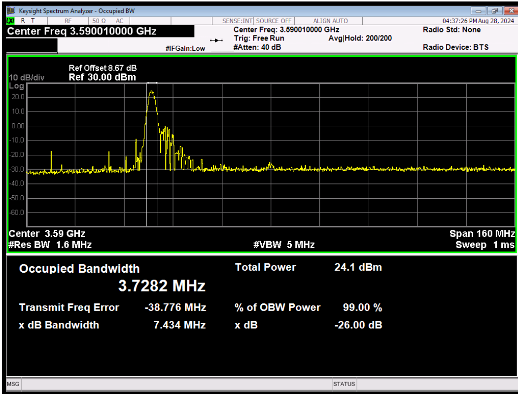
MIMO\PC3\NR n48 SCS=30kHz CP_256QAM BW=80MHz Channel=639334 RB=1@0
