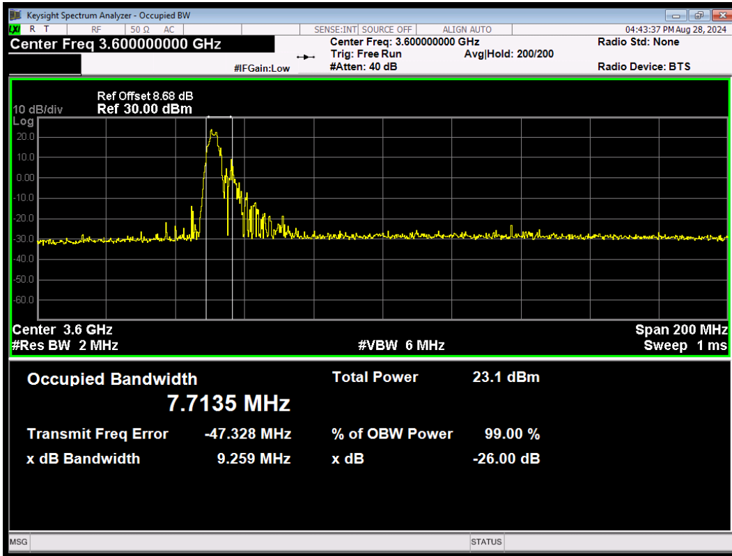
MIMO\PC3\NR n48 SCS=30kHz CP_256QAM BW=100MHz Channel=640000 RB=1@0
