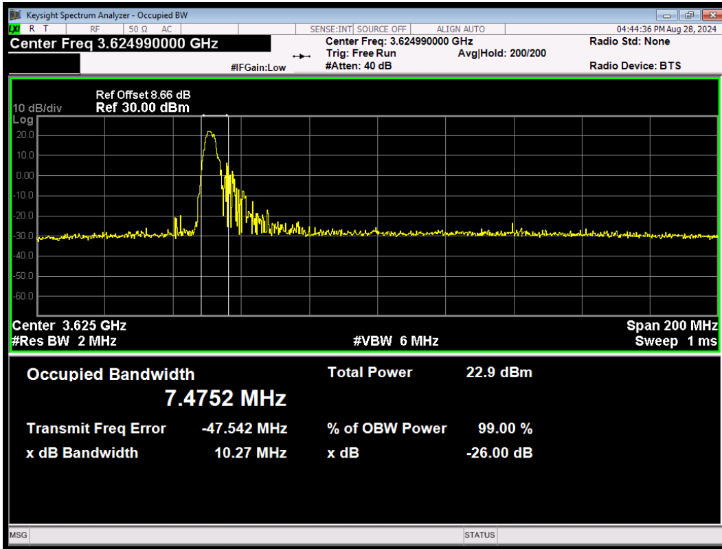
MIMO\PC3\NR n48 SCS=30kHz CP_256QAM BW=100MHz Channel=641666 RB=1@0
