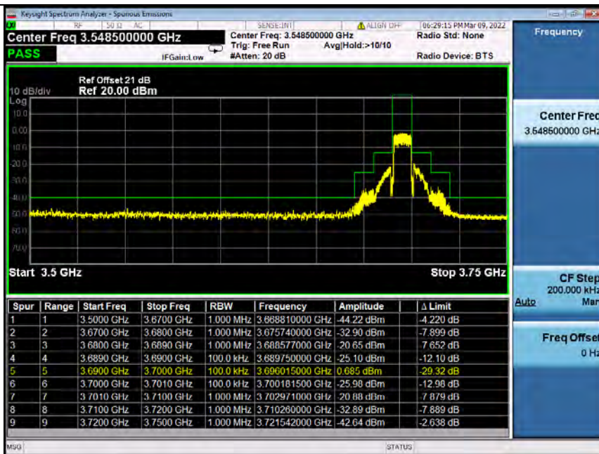
Band48_10MHz_16QAM_HCH_3695MHz_RB_50_0_NTNV
