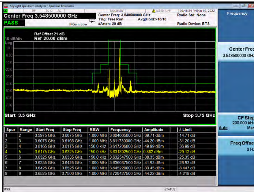
Band48_15MHz_16QAM MCH_3625MHz_RB_75_0_NTNV
