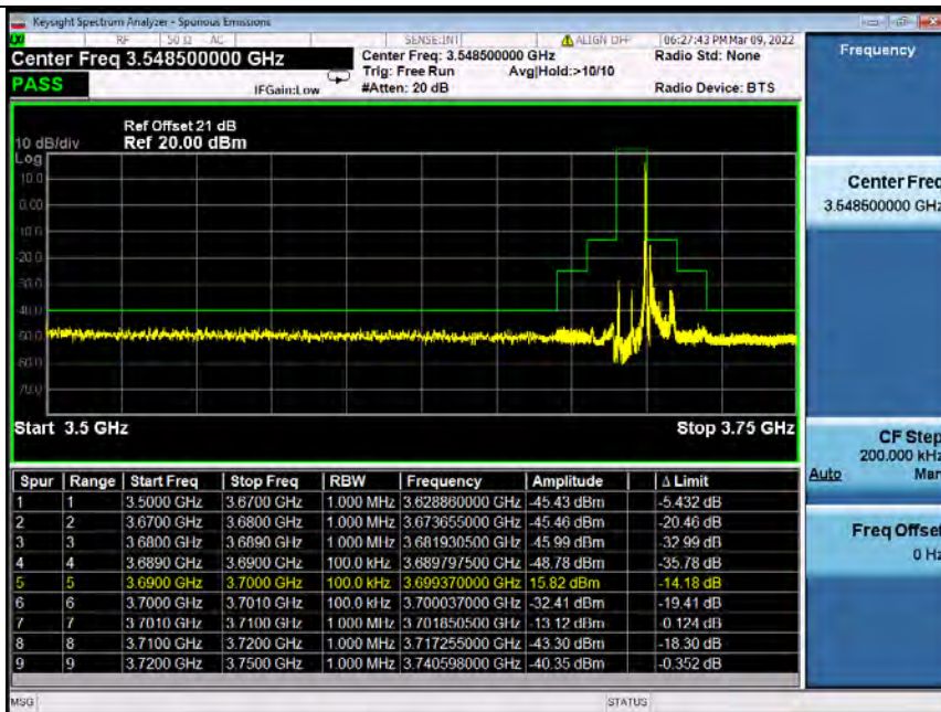
Band48_10MHz_64QAM_HCH_3695MHz_RB_50_0_NTNV
