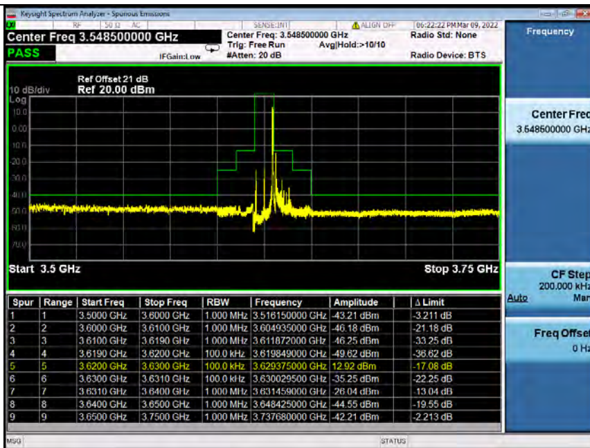
Band48_10MHz_64QAM MCH_3625MHz_RB_50_0_NTNV
