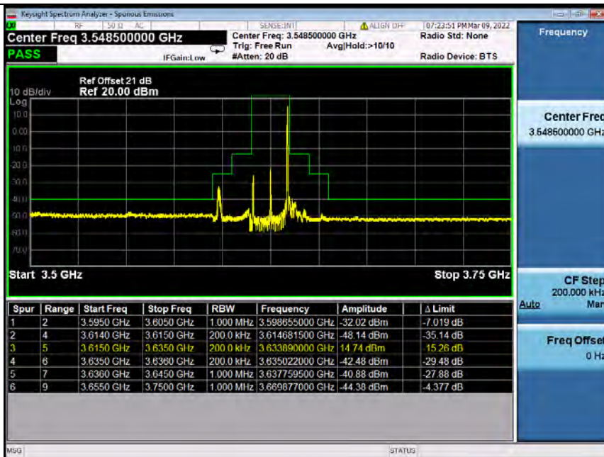
Band48_20MHz_64QAM MCH_3625MHz_RB_100_0_NTNV
