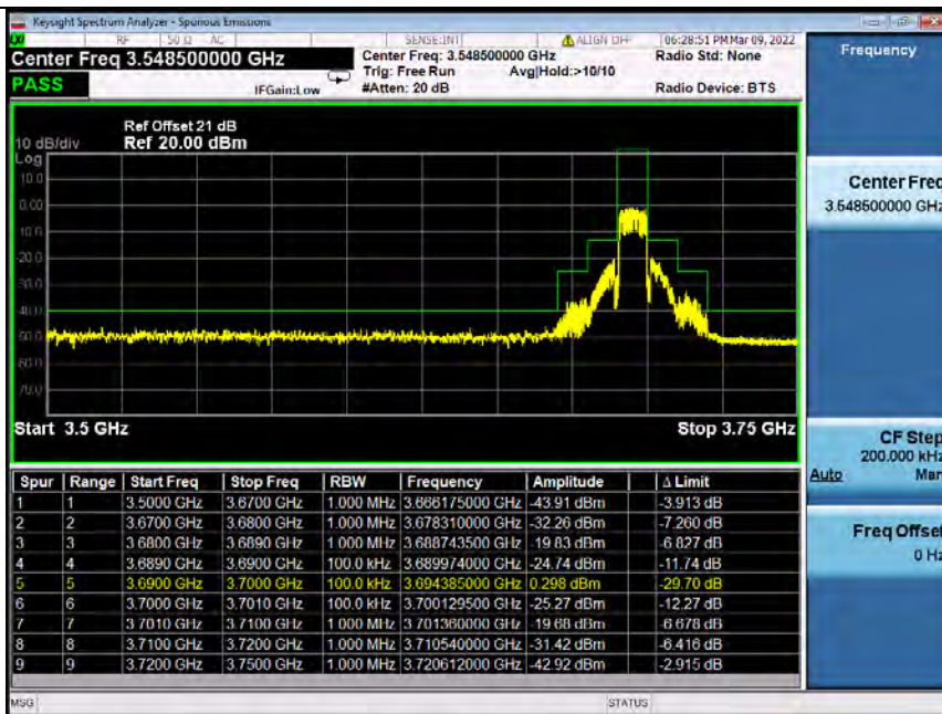
Band48_10MHz_64QAM_HCH_3695MHz_RB_50_0_NTNV
