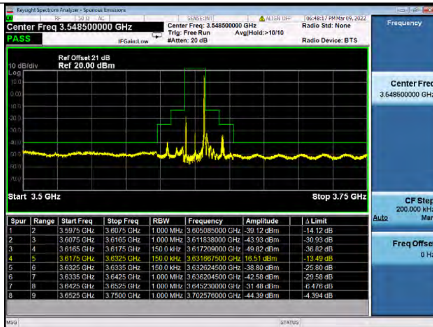
Band48_15MHz_64QAM MCH_3625MHz_RB_75_0_NTNV
