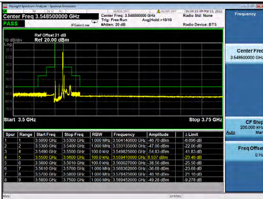
Band48_10MHz_64QAM_LCH_3555MHz_RB_50_0_NTNV
