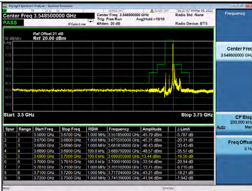
Band48_10MHz_16QAM_HCH_3695MHz_RB_50_0_NTNV
