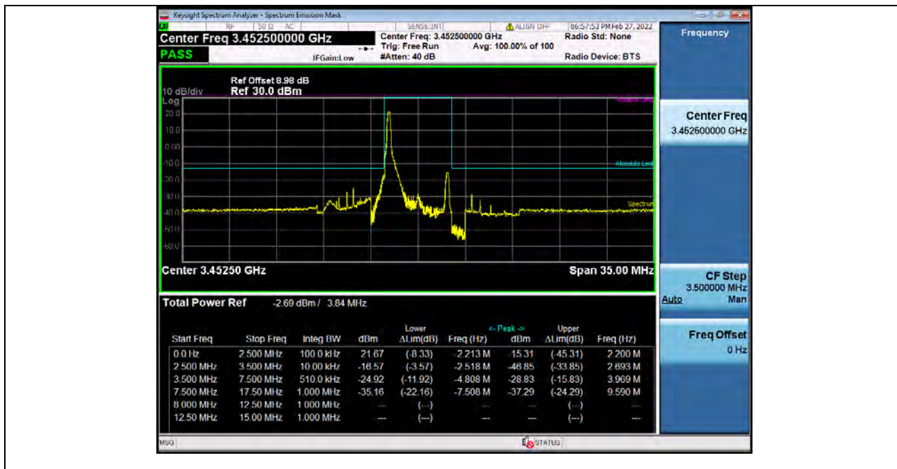
Band42H_5MHz_64QAM_LCH_3452.5MHz_RB_25_0_NTNV_Bandedge
