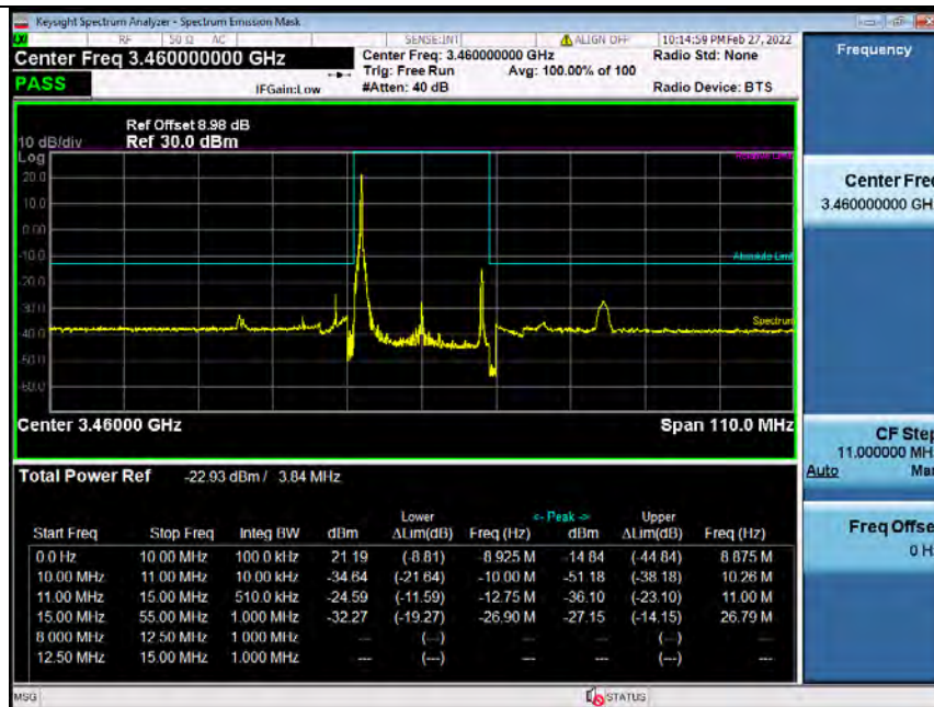
Band42H_20MHz_16QAM_LCH_3460MHz_RB_100_0_NTNV_Bandedge
