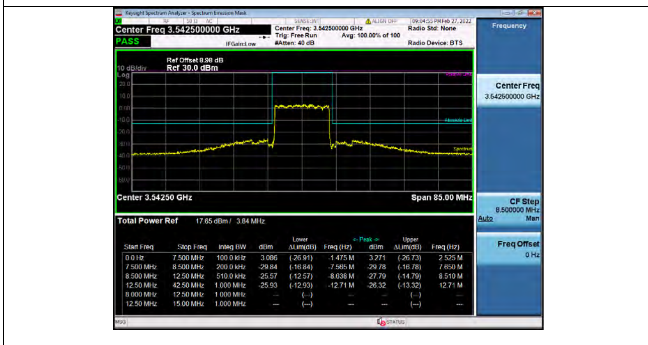
Band42H_15MHz_64QAM_HCH_3542.5MHz_RB_75_0_NTNV_Bandedge
