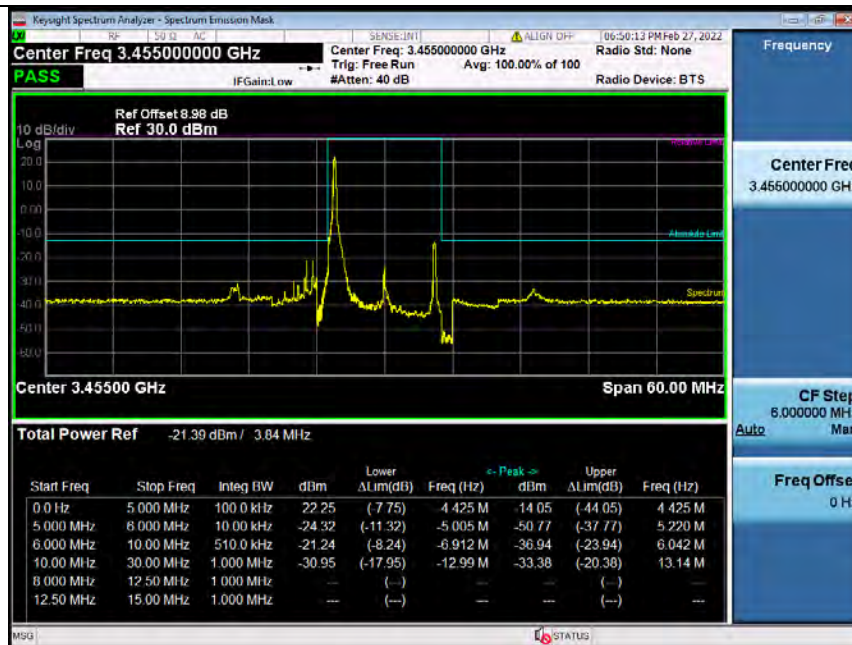
Band42H_10MHz_16QAM_LCH_3455MHz_RB_50_0_NTNV_Bandedge
