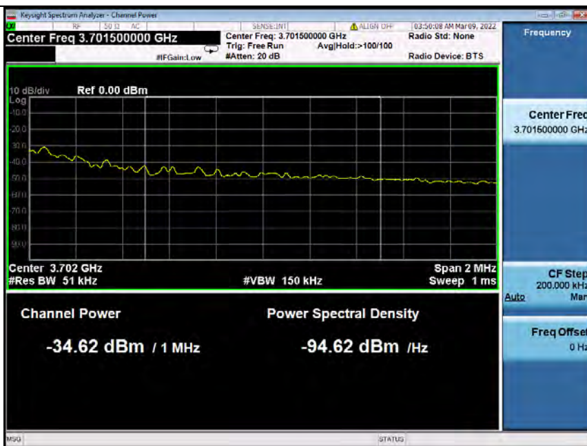
Band48_5MHz_64QAM_HCH_3697.5MHz_RB_25_0_NTNV
