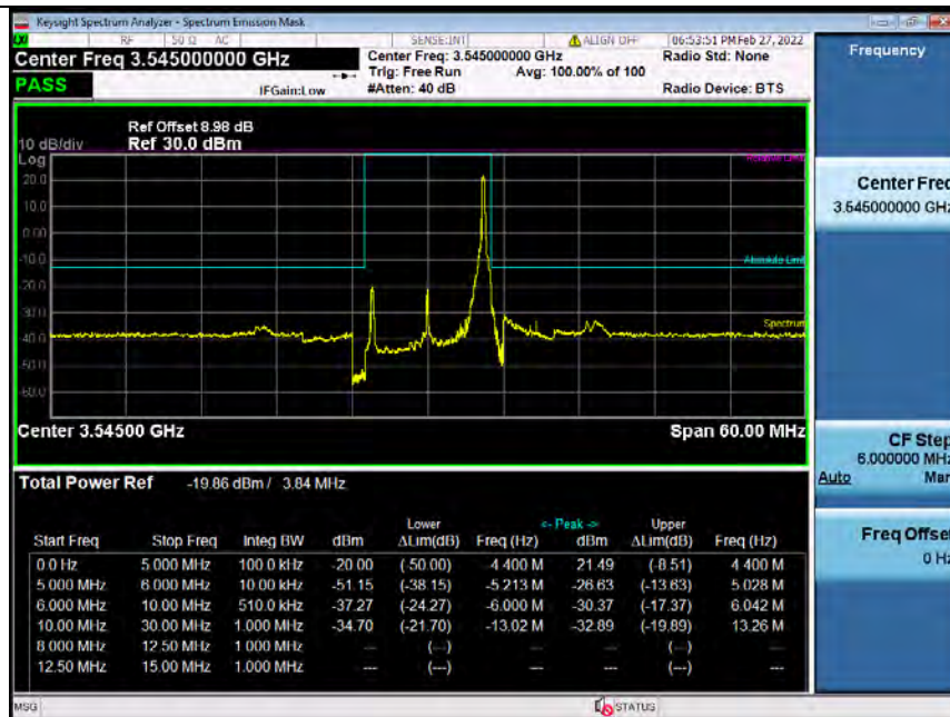
Band42H_10MHz_16QAM_HCH_3545MHz_RB_50_0_NTNV_Bandedge
