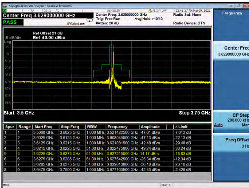
Band48_5MHz_16QAM_MCH_3625MHz_RB_1_24_NTNV (Integrated Power for 3628.5-3629.5MHz)
