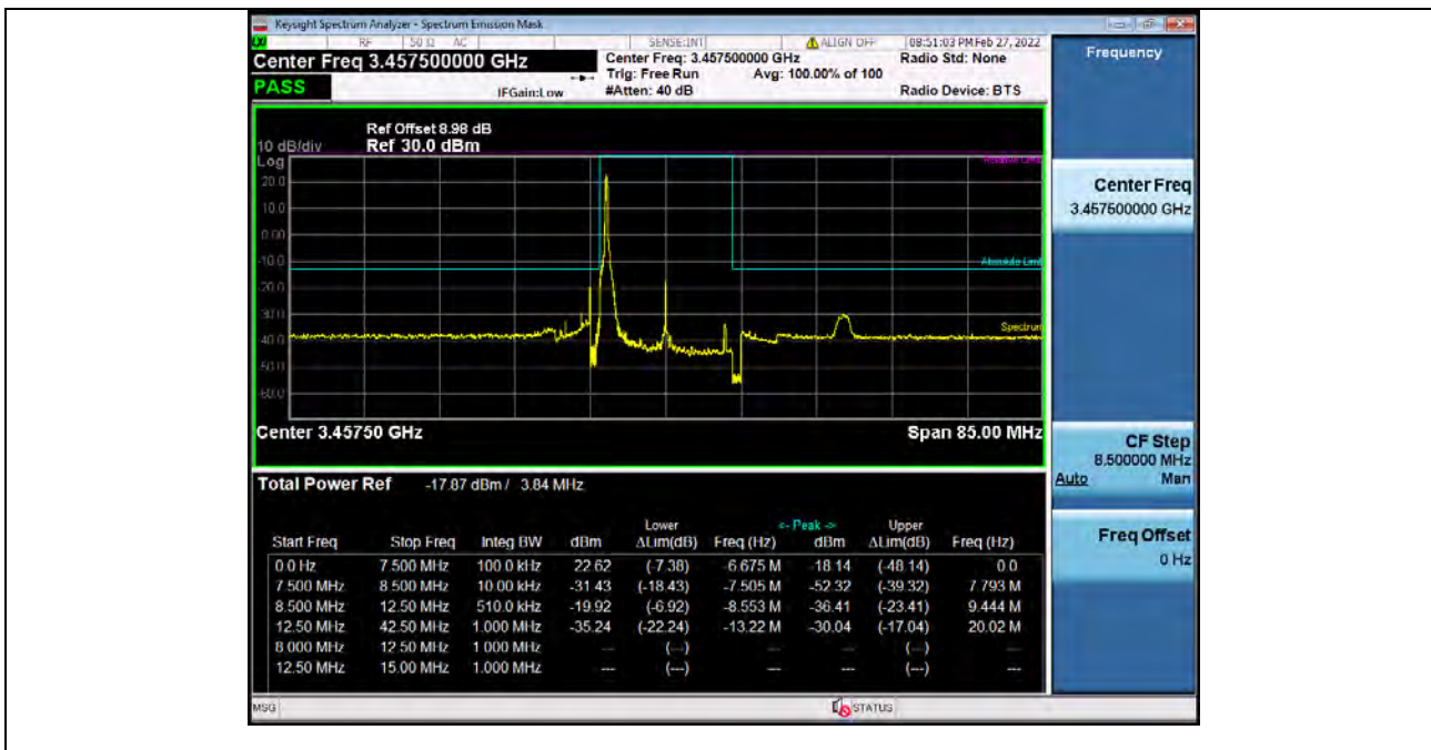
Band42H_15MHz_16QAM_LCH_3457.5MHz_RB_75_0_NTNV_Bandedge
