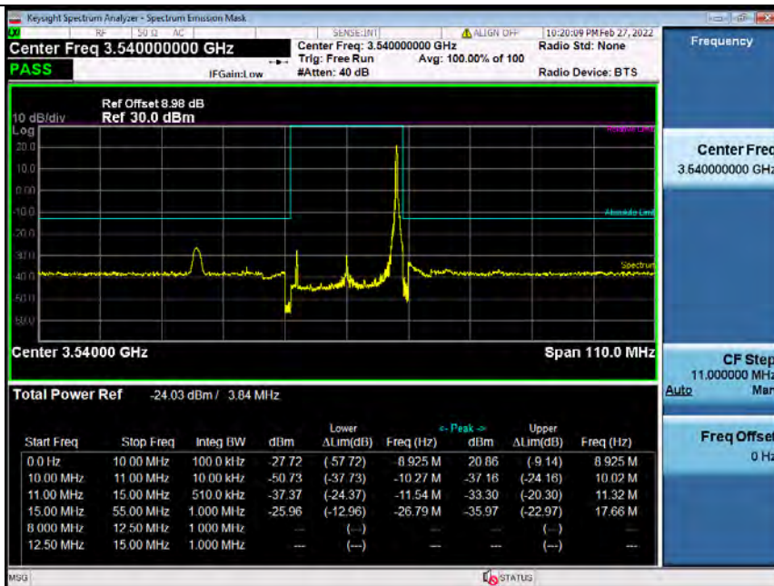
Band42H_20MHz_16QAM_HCH_3540MHz_RB_100_0_NTNV_Bandedge
