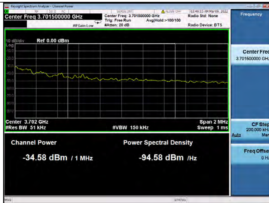
Band48_5MHz_QPSK_HCH_3697.5MHz_RB_25_0_NTNV
