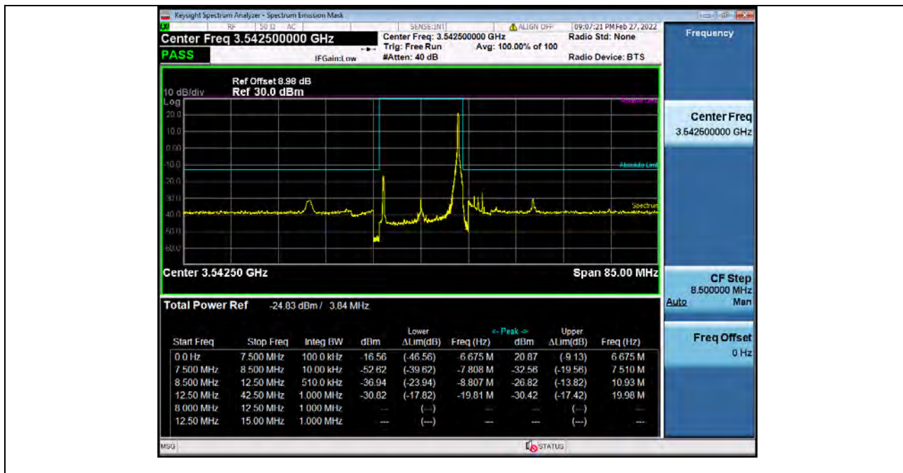
Band42H_15MHz_64QAM_HCH_3542.5MHz_RB_75_0_NTNV_Bandedge
