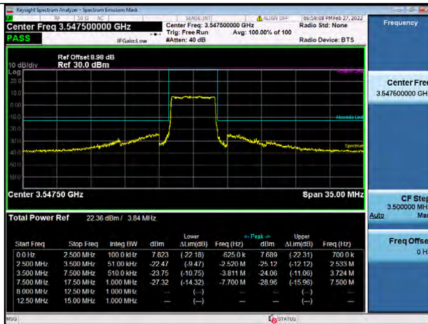
Band42H_5MHz_64QAM_HCH_3547.5MHz_RB_25_0_NTNV_Bandedge
