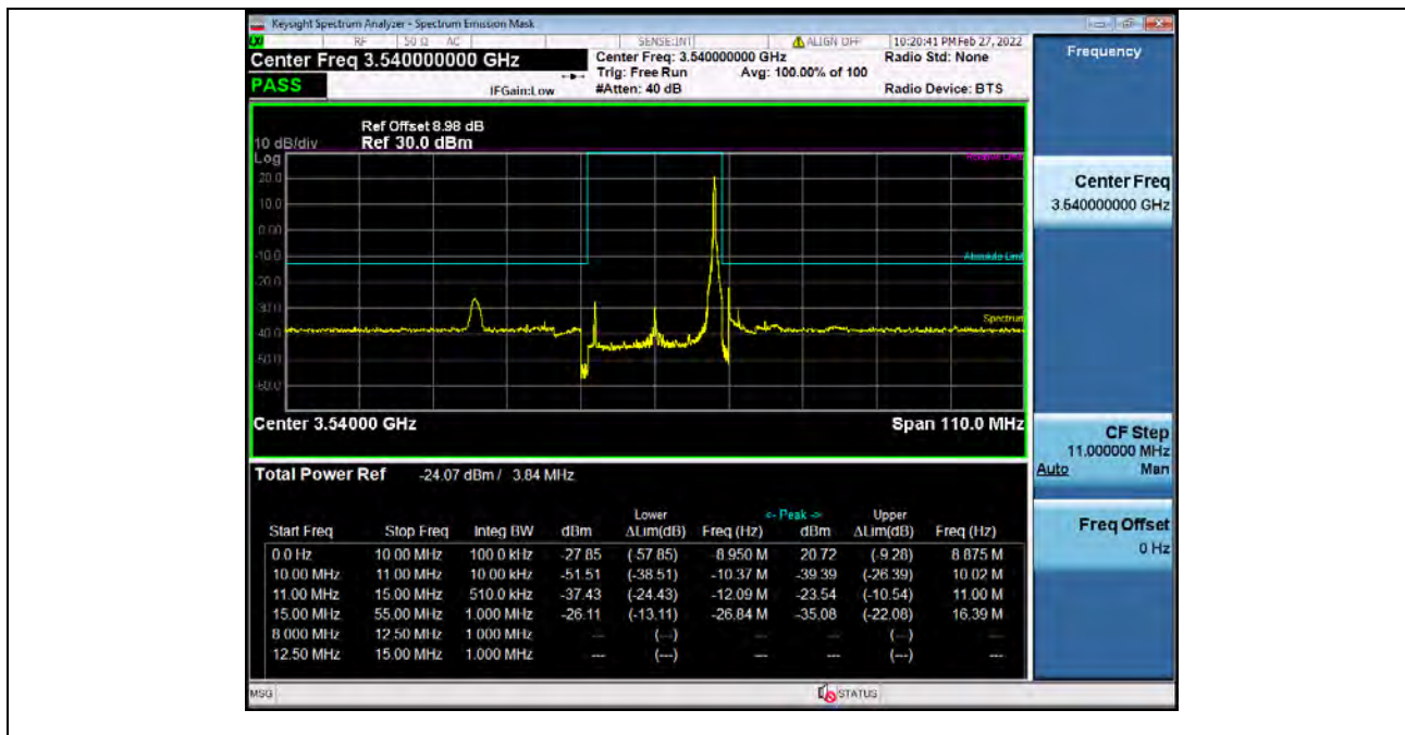
Band42H_20MHz_64QAM_HCH_3540MHz_RB_100_0_NTNV_Bandedge
