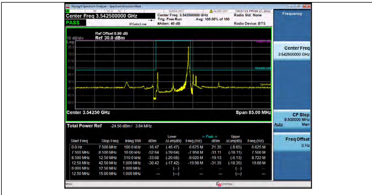
Band42H_15MHz_16QAM_HCH_3542.5MHz_RB_75_0_NTNV_Bandedge
