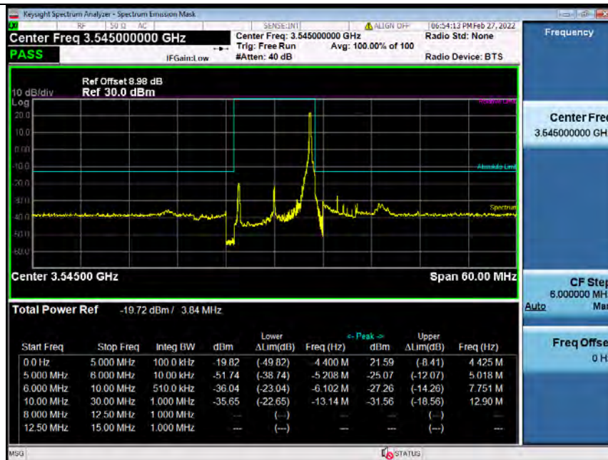
Band42H_10MHz_64QAM_HCH_3545MHz_RB_50_0_NTNV_Bandedge
