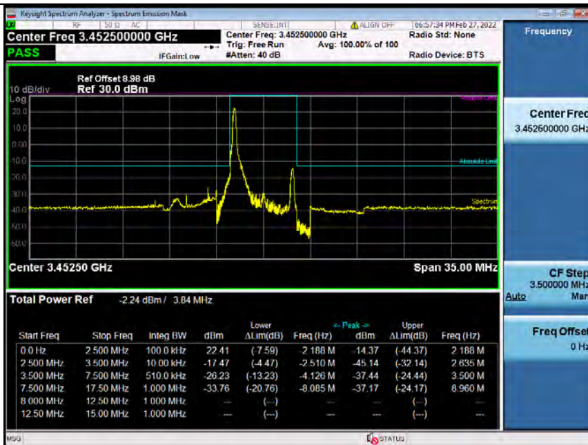
Band42H_5MHz_16QAM_LCH_3452.5MHz_RB_25_0_NTNV_Bandedge
