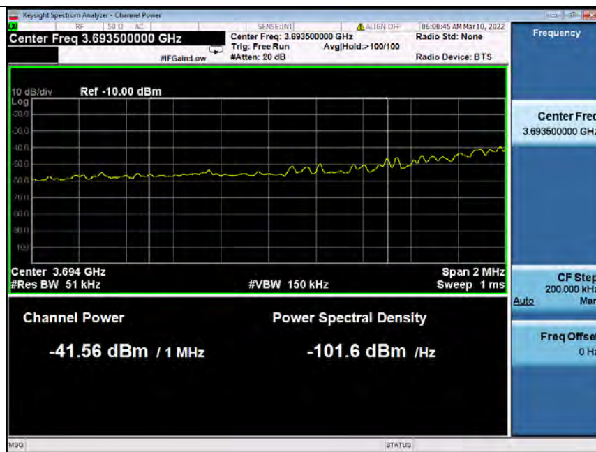
Band48_5MHz_16QAM_HCH_3697.5MHz_RB_1_24_NTNV
