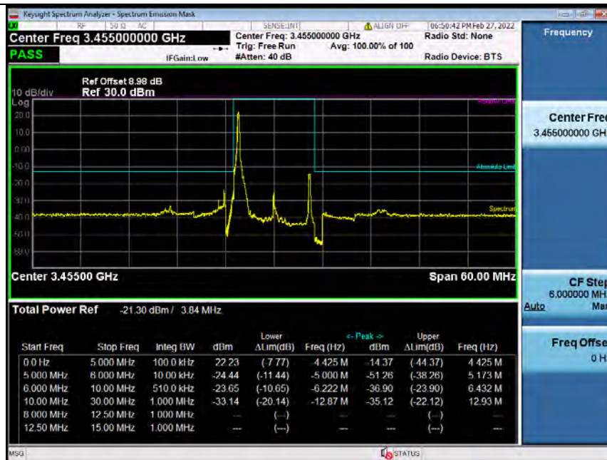
Band42H_10MHz_64QAM_LCH_3455MHz_RB_50_0_NTNV_Bandedge
