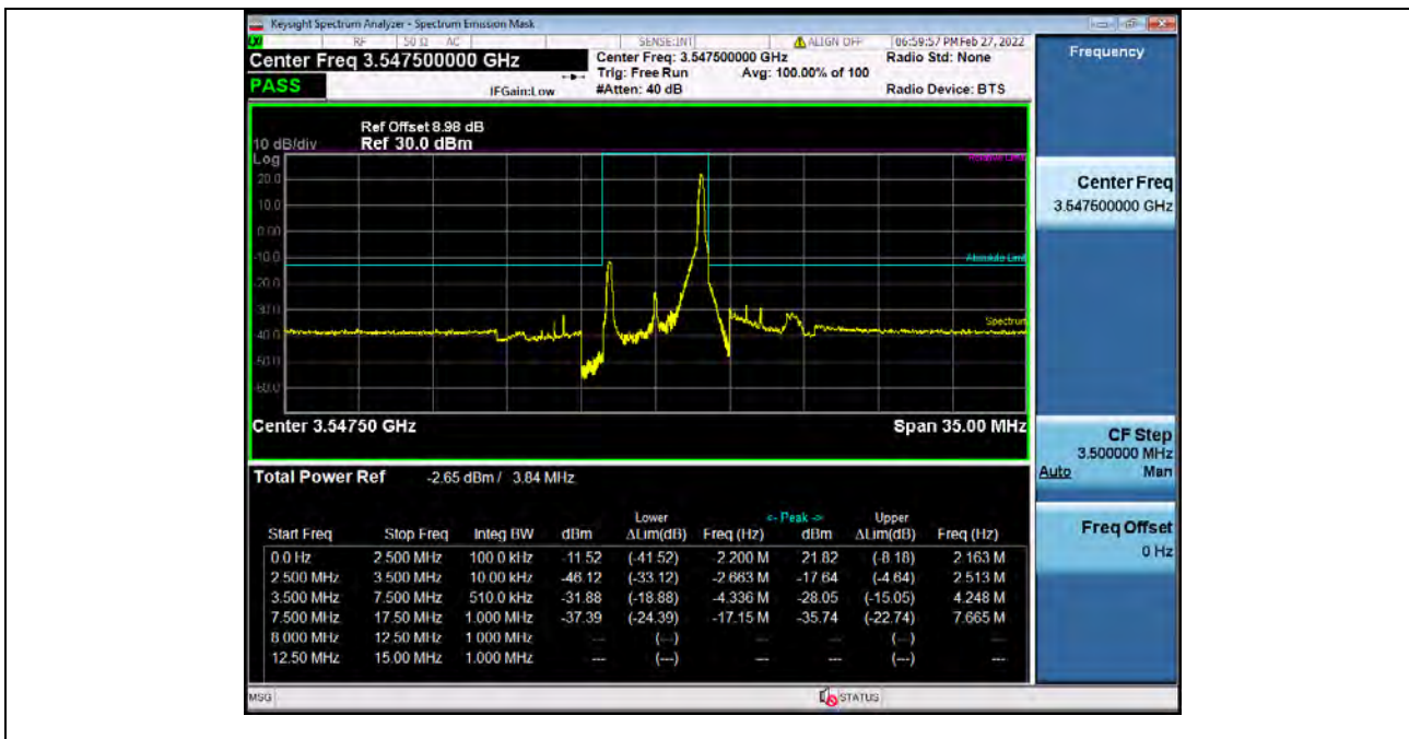
Band42H_5MHz_16QAM_HCH_3547.5MHz_RB_25_0_NTNV_Bandedge
