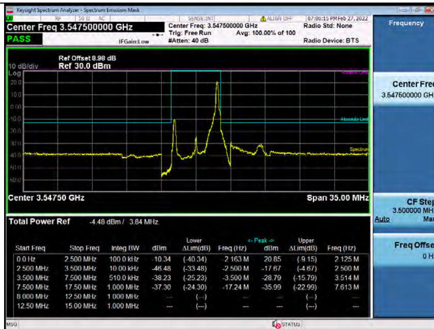
Band42H_5MHz_64QAM_HCH_3547.5MHz_RB_25_0_NTNV_Bandedge
