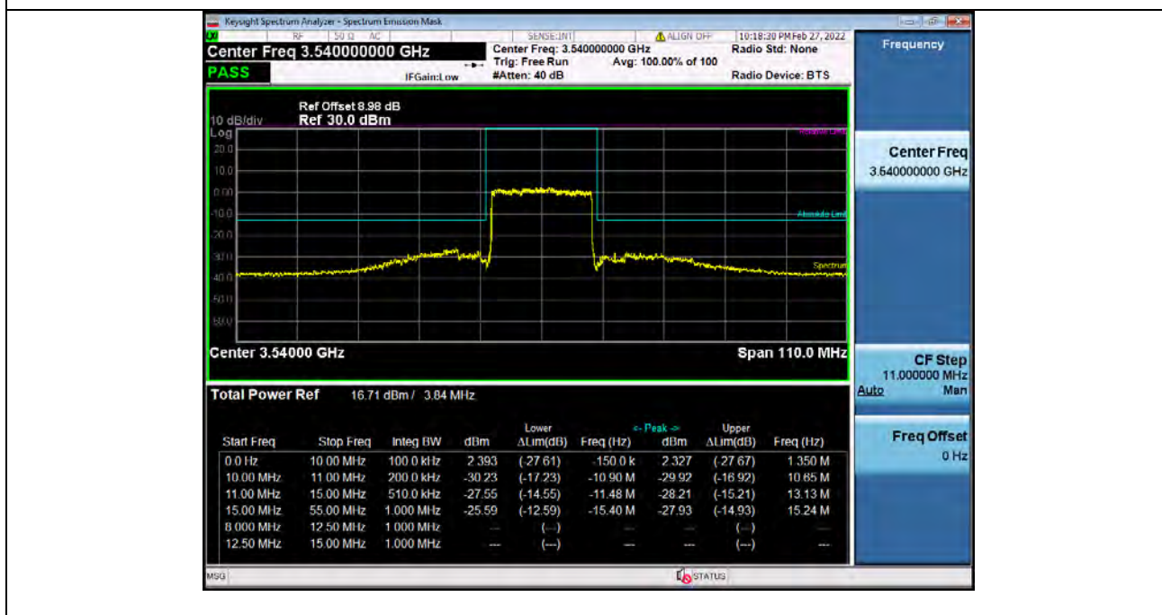
Band42H_20MHz_64QAM_HCH_3540MHz_RB_100_0_NTNV_Bandedge
