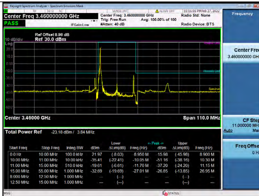
Band42H_20MHz_64QAM_LCH_3460MHz_RB_100_0_NTNV_Bandedge
