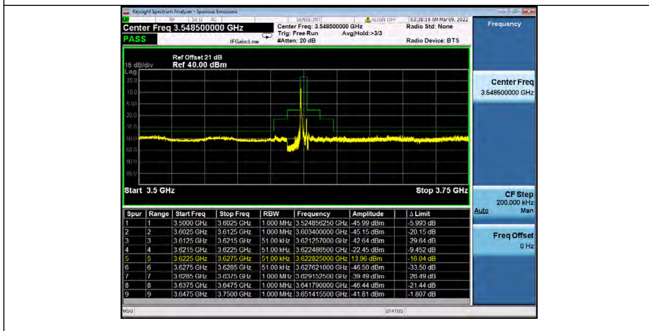
Band48_5MHz_16QAM_MCH_3625MHz_RB_1_0_NTNV (Integrated Power for 3620.5-3621.5MHz)
