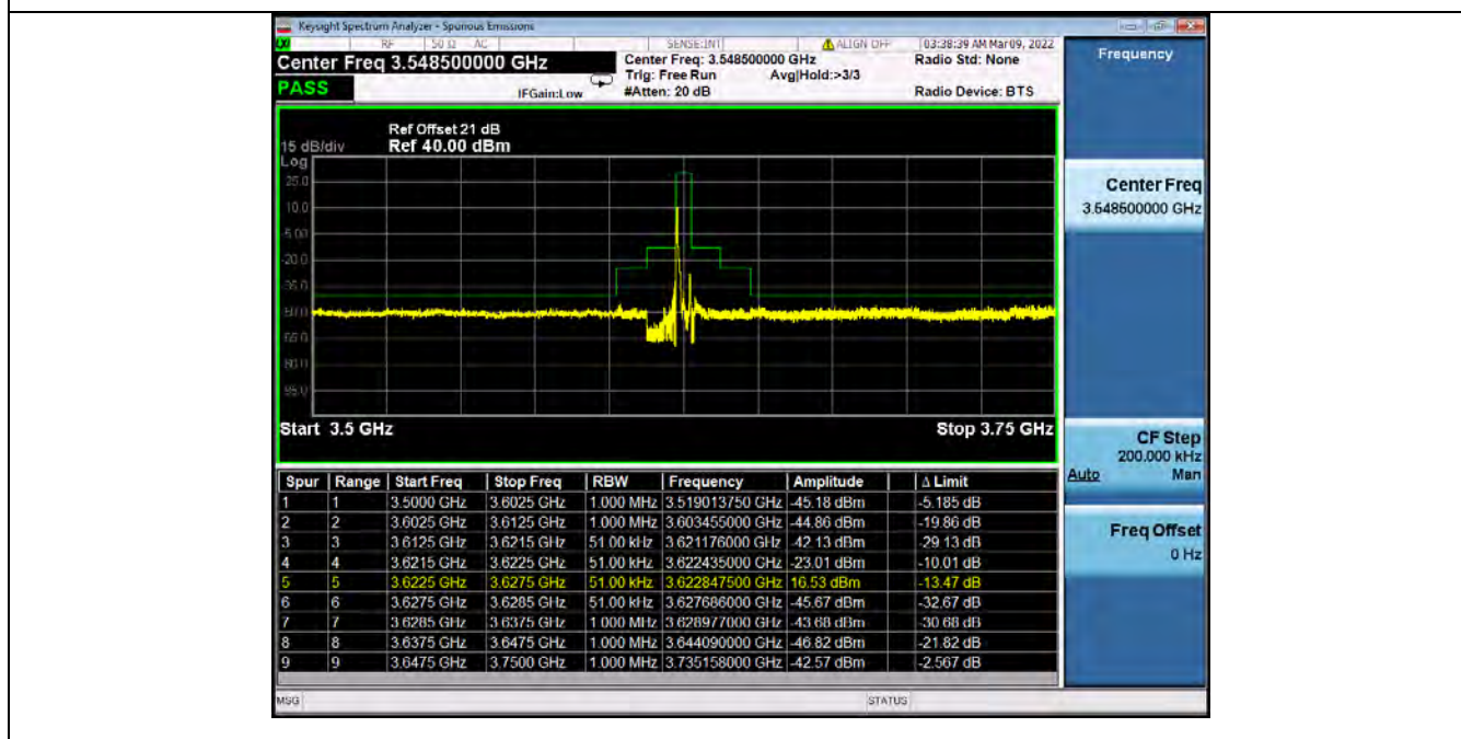
Band48_5MHz_QPSK_MCH_3625MHz_RB_1_0_NTNV (Integrated Power for 3620.5-3621.5MHz)
