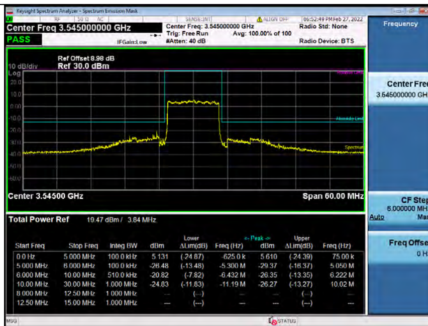
Band42H_10MHz_64QAM_HCH_3545MHz_RB_50_0_NTNV_Bandedge
