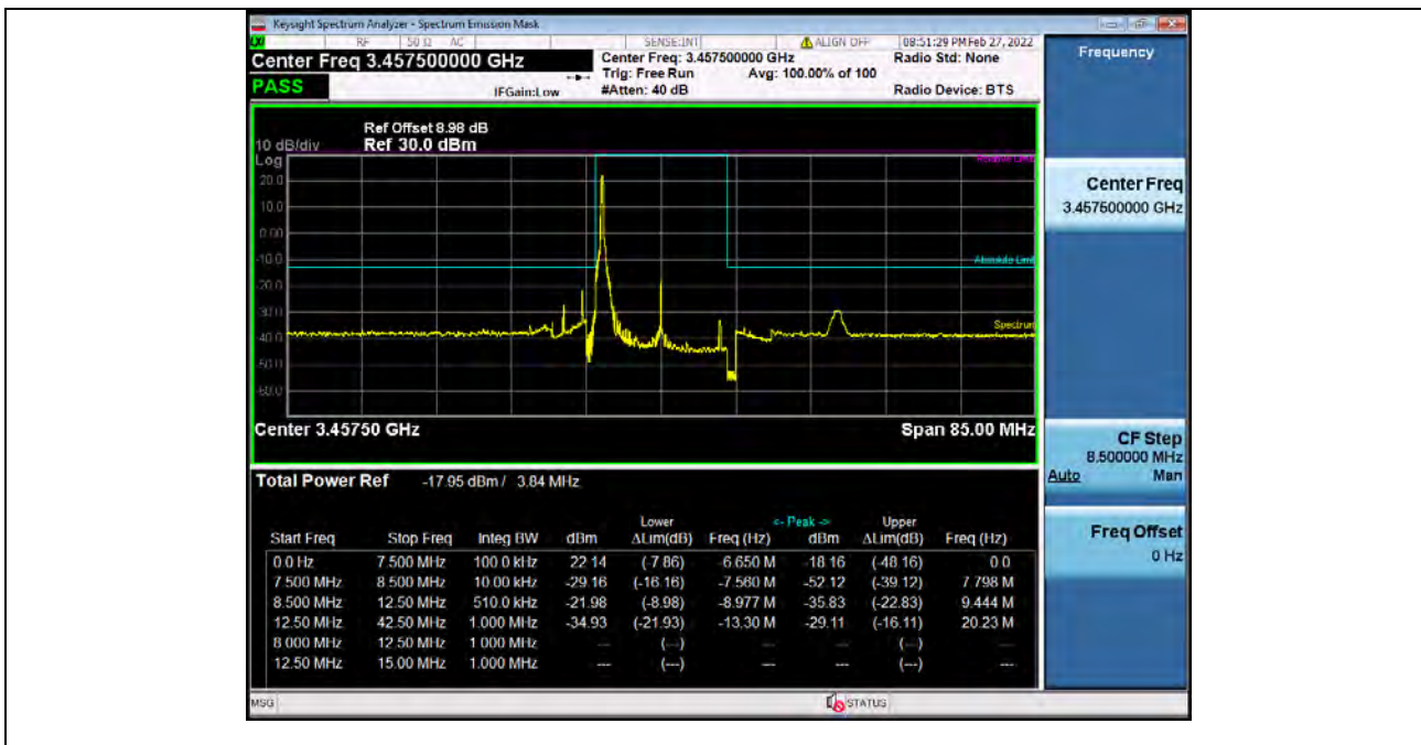
Band42H_15MHz_64QAM_LCH_3457.5MHz_RB_75_0_NTNV_Bandedge
