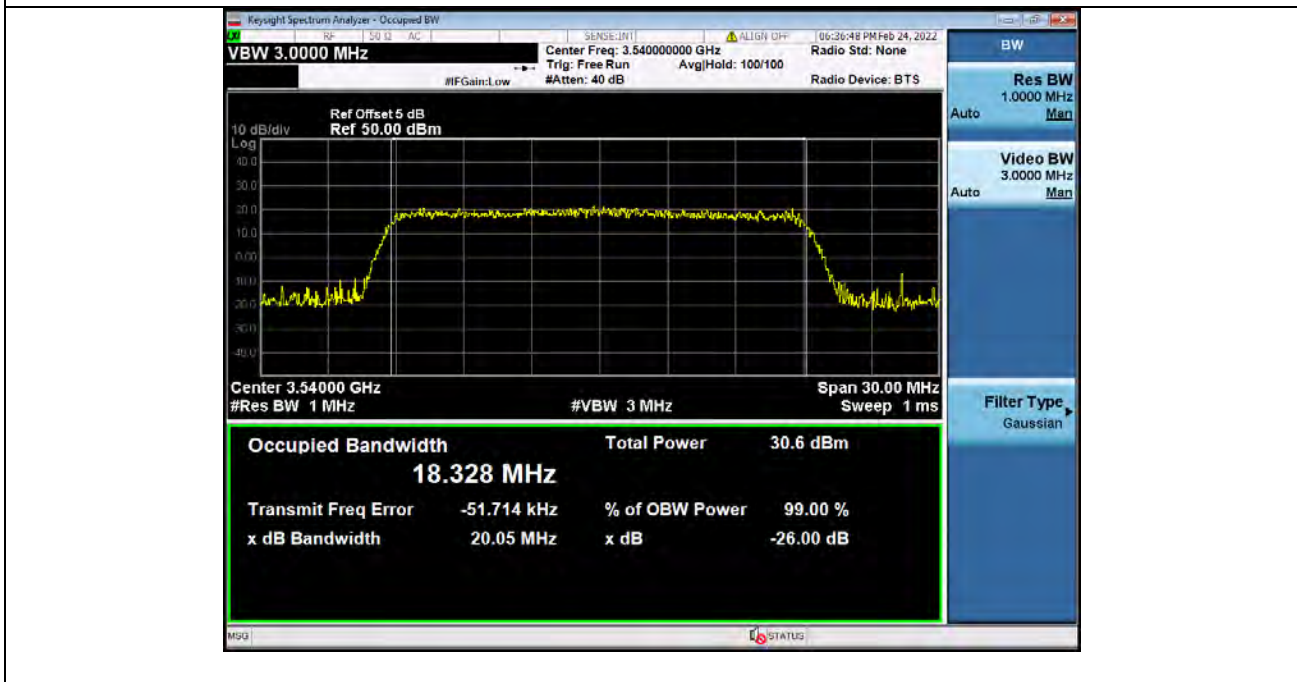
Band42H_20MHz_64QAM_HCH_3540MHz_RB_100_0_NTNV
