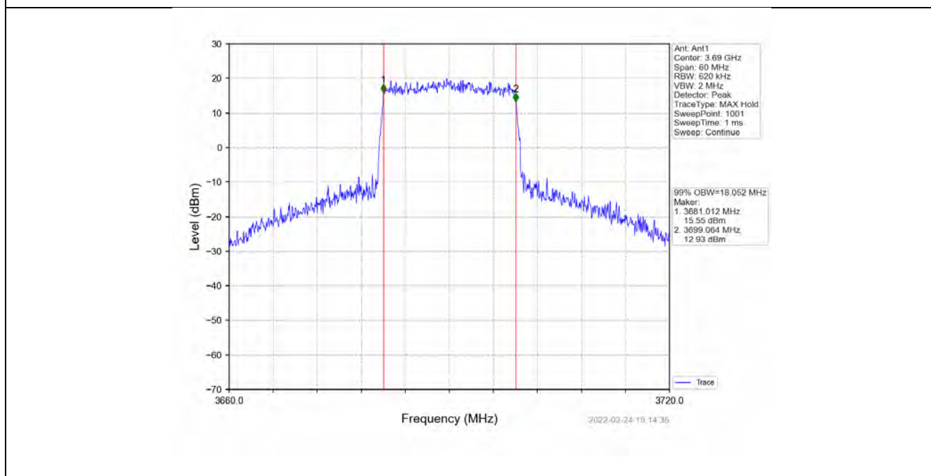
Band48_20MHz_64QAM_HCH_3690MHz_RB_100_0_NTNV
