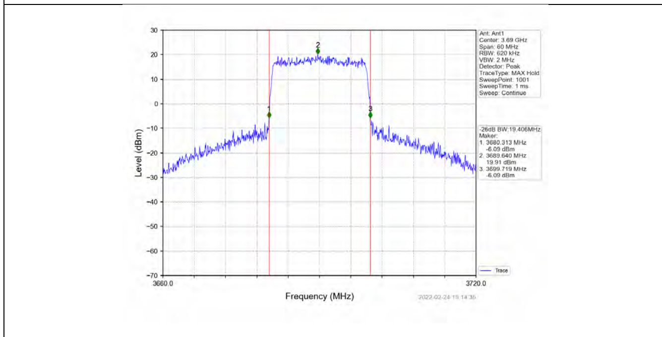
Band48_20MHz_64QAM_HCH_3690MHz_RB_100_0_NTNV
