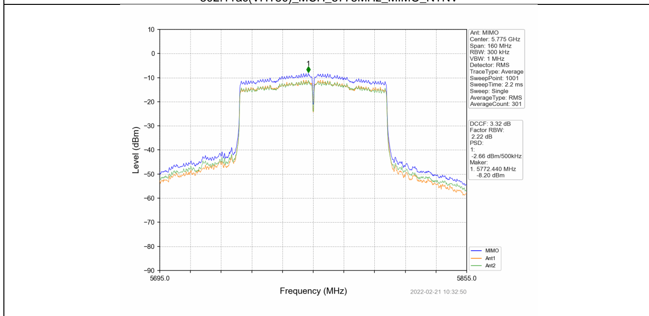
802.11ac(VHT80)_MCH_5775MHz_MIMO_NTNV
