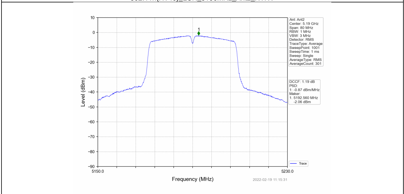
802.11n(HT40)_LCH_5190MHz_MIMO_NTNV
