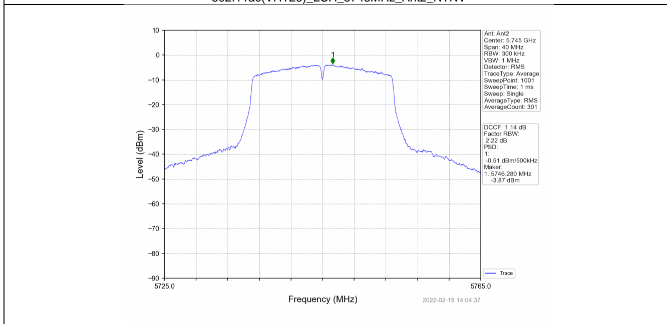
802.11ac(VHT20)_LCH_5745MHz_MIMO_NTNV
