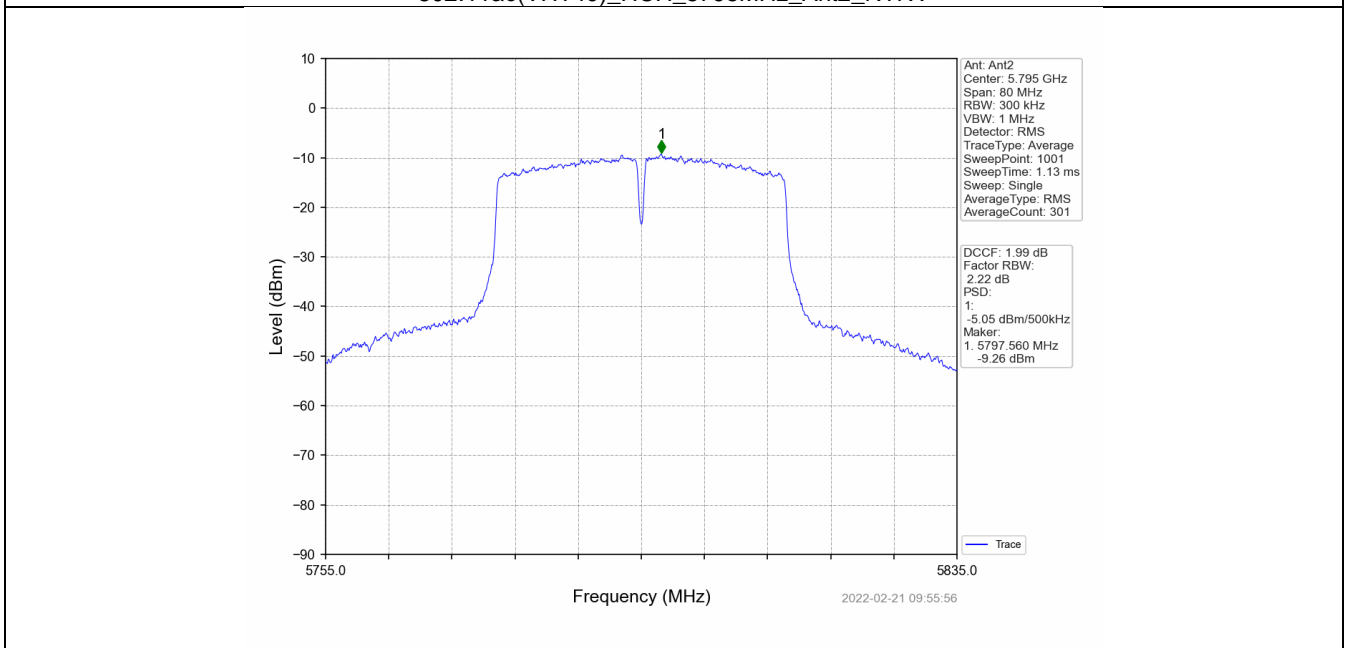
802.11ac(VHT40)_HCH_5795MHz_MIMO_NTNV
