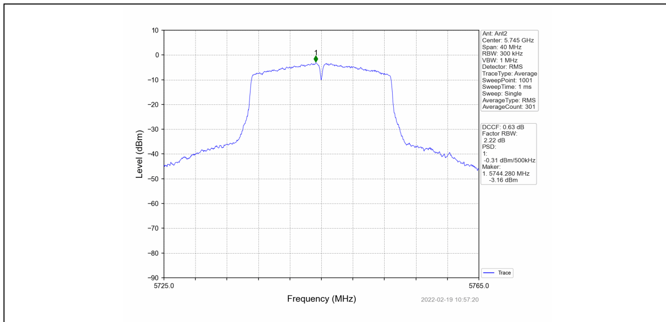
802.11n(HT20)_LCH_5745MHz_MIMO_NTNV
