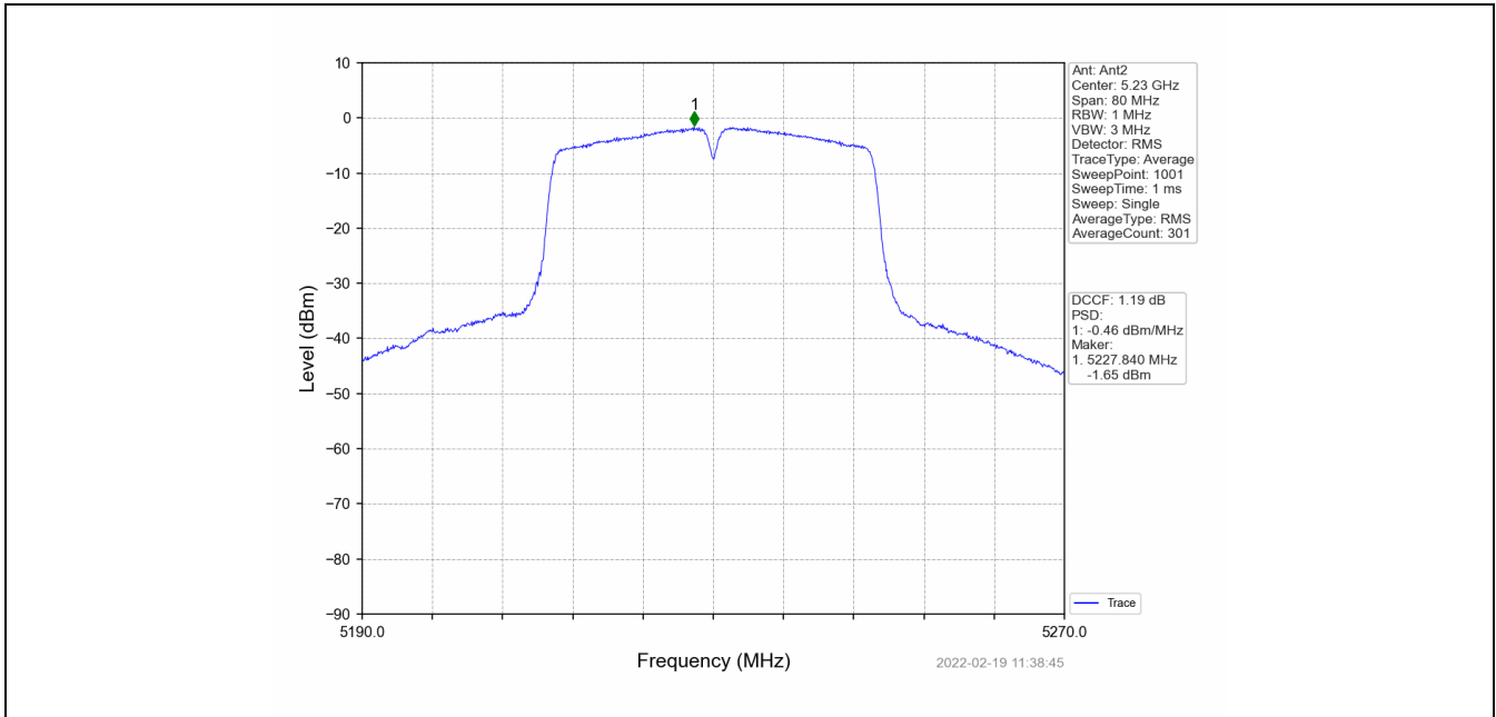
802.11n(HT40)_HCH_5230MHz_MIMO_NTNV
