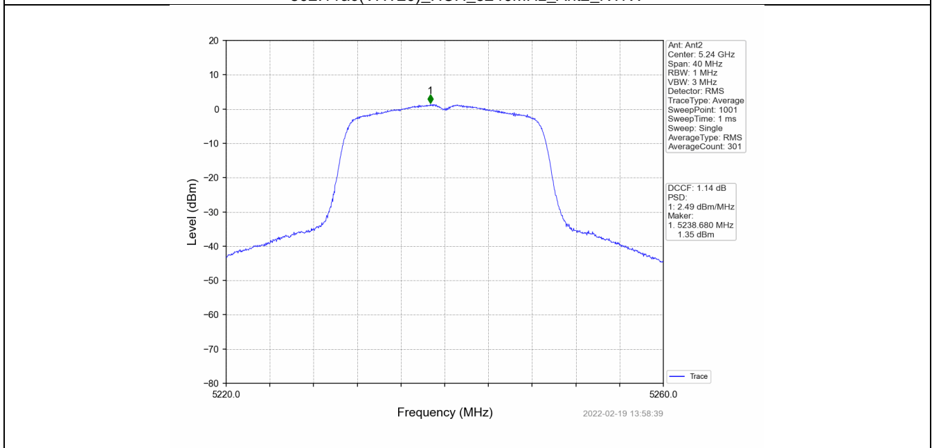
802.11ac(VHT20)_HCH_5240MHz_MIMO_NTNV
