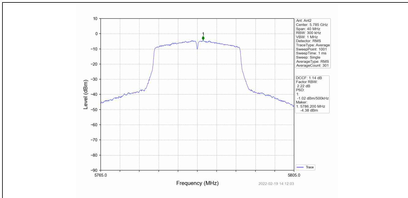
802.11ac(VHT20)_MCH_5785MHz_MIMO_NTNV
