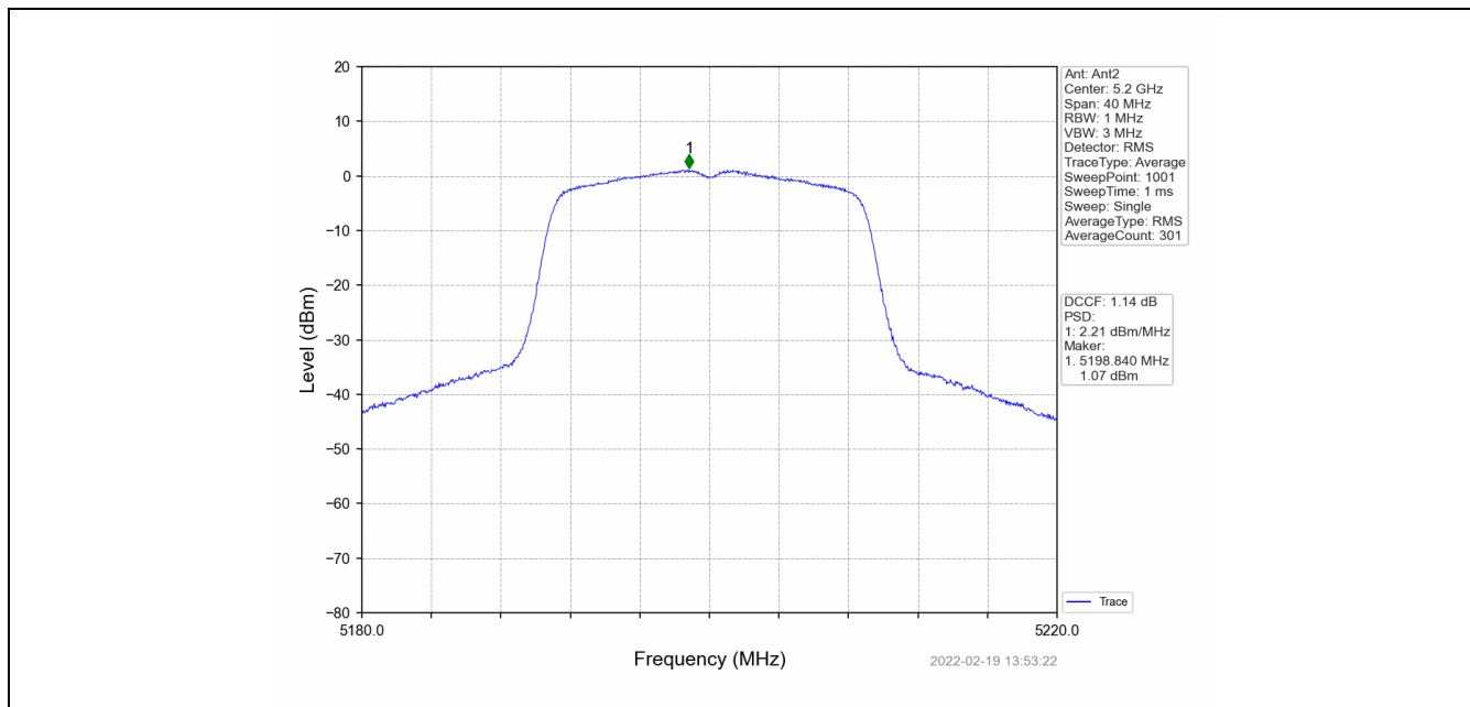
802.11ac(VHT20)_MCH_5200MHz_MIMO_NTNV
