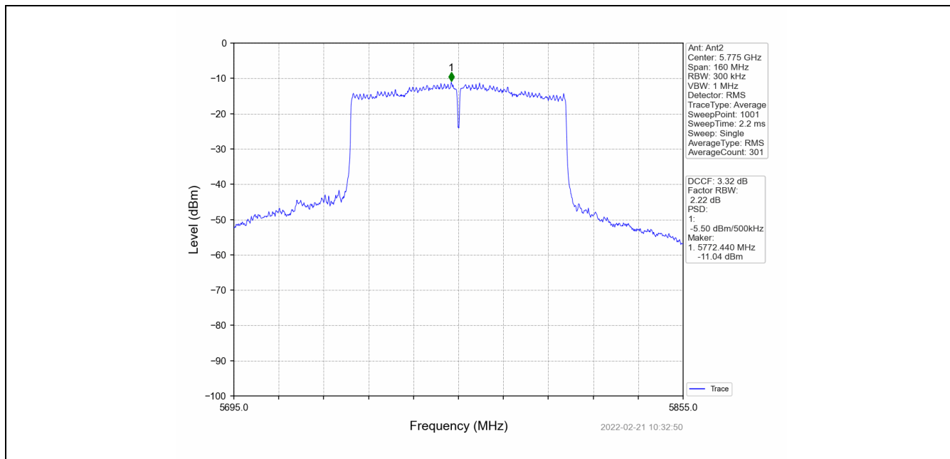
802.11ac(VHT80)_MCH_5775MHz_MIMO_NTNV
