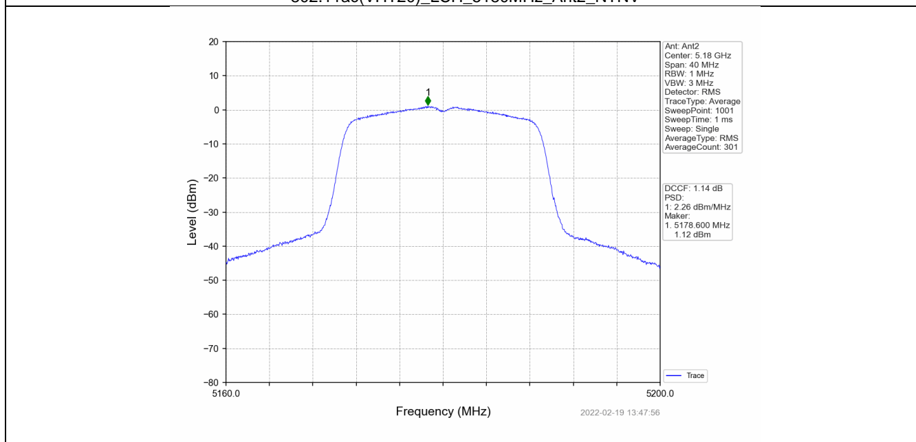
802.11ac(VHT20)_LCH_5180MHz_MIMO_NTNV
