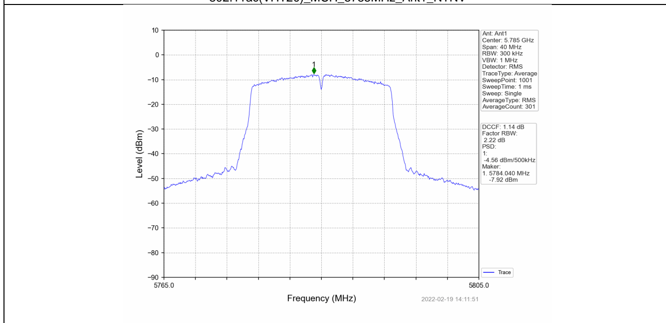
802.11ac(VHT20)_MCH_5785MHz_Ant2_NTNV
