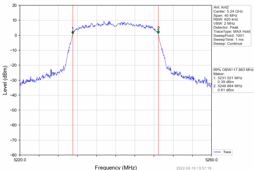
802.11ac(VHT20)_HCH_5240MHz_Ant2_NTNV
