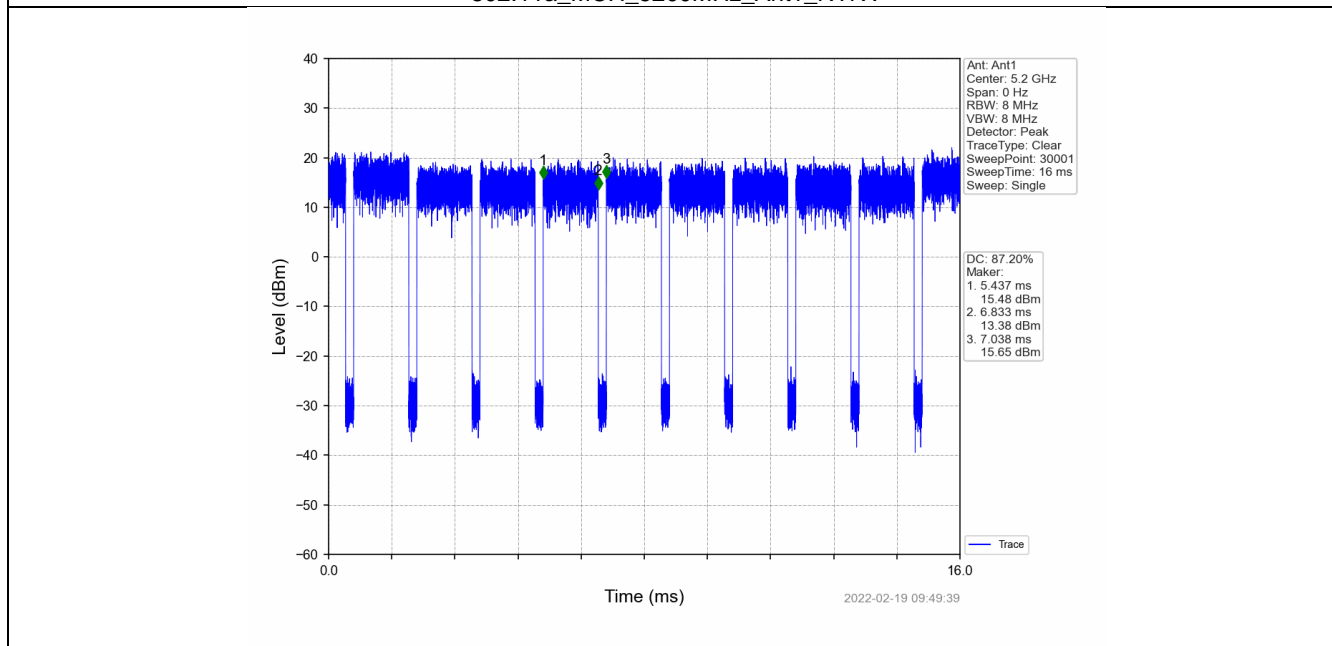
802.11a_HCH_5240MHz_Ant1_NTNV
