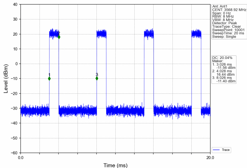
n48_30kHz_SISO_NTNV_40MHz_DFT-s-OFDM 16 QAM_3570MHz_Inner_Full
