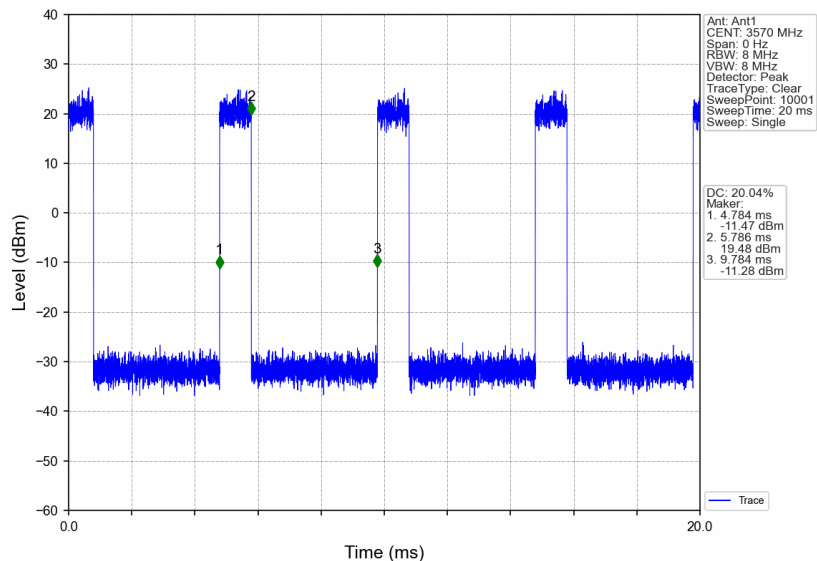
n48_30kHz_SISO_NTNV_40MHz_CP-OFDM 16 QAM_3570MHz_Inner_Full
