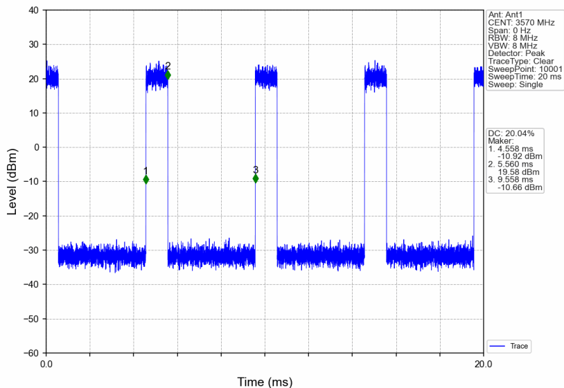
n48_30kHz_SISO_NTNV_40MHz_CP-OFDM QPSK_3570MHz_Inner_Full
