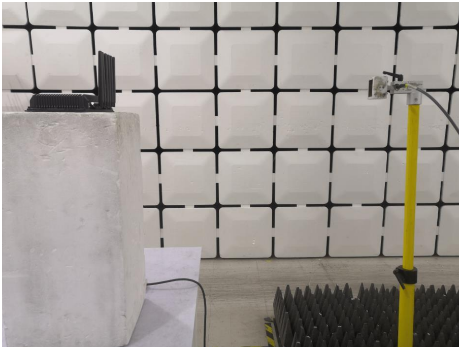
Radiated Spurious Emissions (Above 18GHz)
