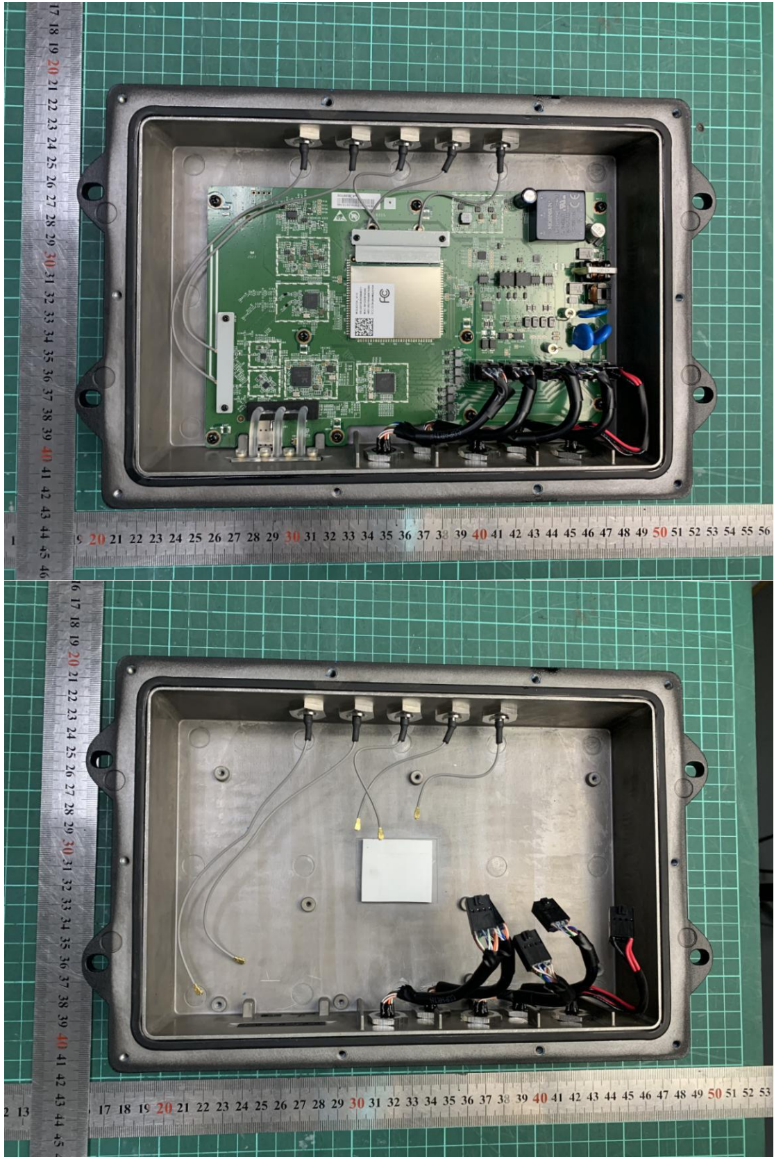
SRP410-b internal photo
