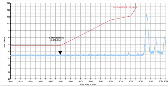
5745M: Peak
