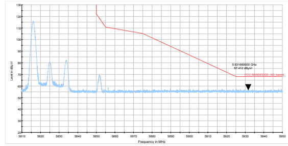
5825M: Peak
