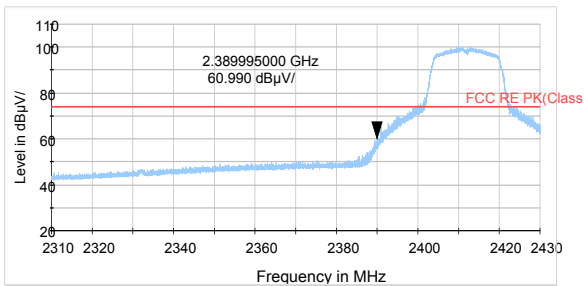
802.11g-Channel 1 Peak
