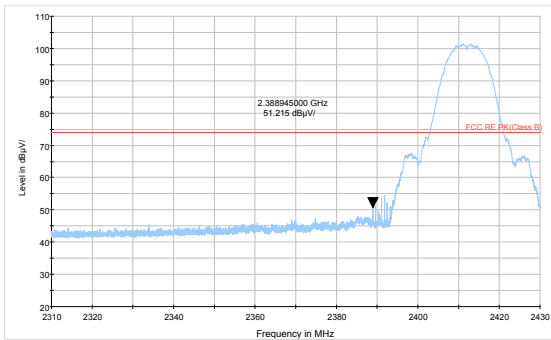
802.11b-Channel 1 Peak
