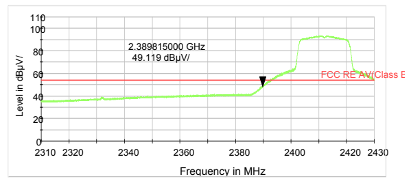
802.11n HT20 -Channel 1 Average
