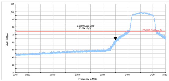
802.11n HT20 -Channel 1 Peak
