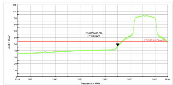
802.11g-Channel 1 Average
