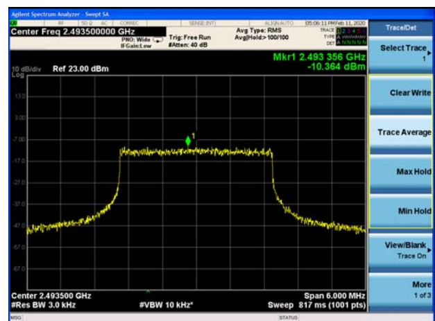
LTE Band 53 3MHz QPSK 1RB CH-High
